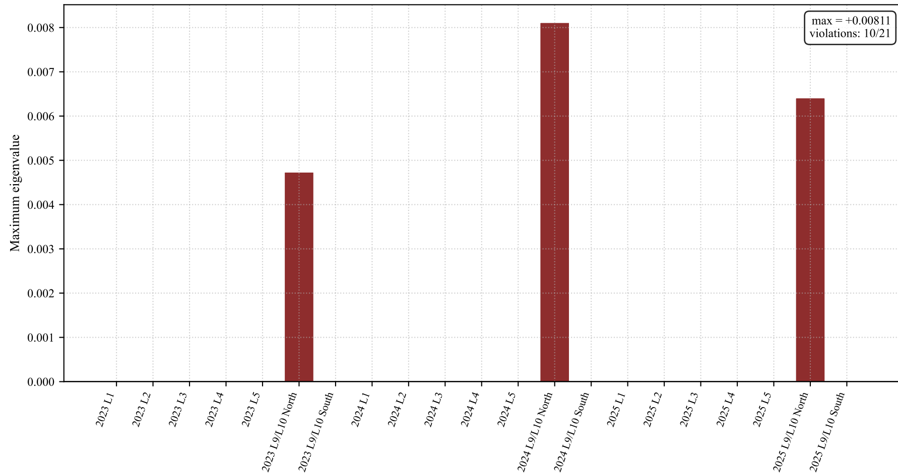
Concavity diagnostic for the full specification (M-FU): maximum eigenvalue of the Allen-Uzawa substitution matrix 10 of 21 observations violate concavity (eigenvalue > 0)
