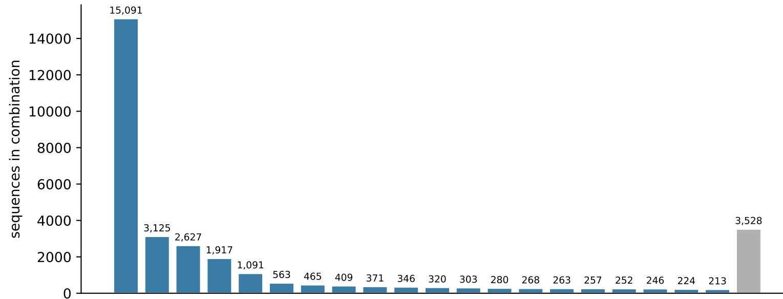
Compartment co-occurrence (UpSet) — top 20 of 104 combinations (89% of sequences; grey = other 84 combos)
