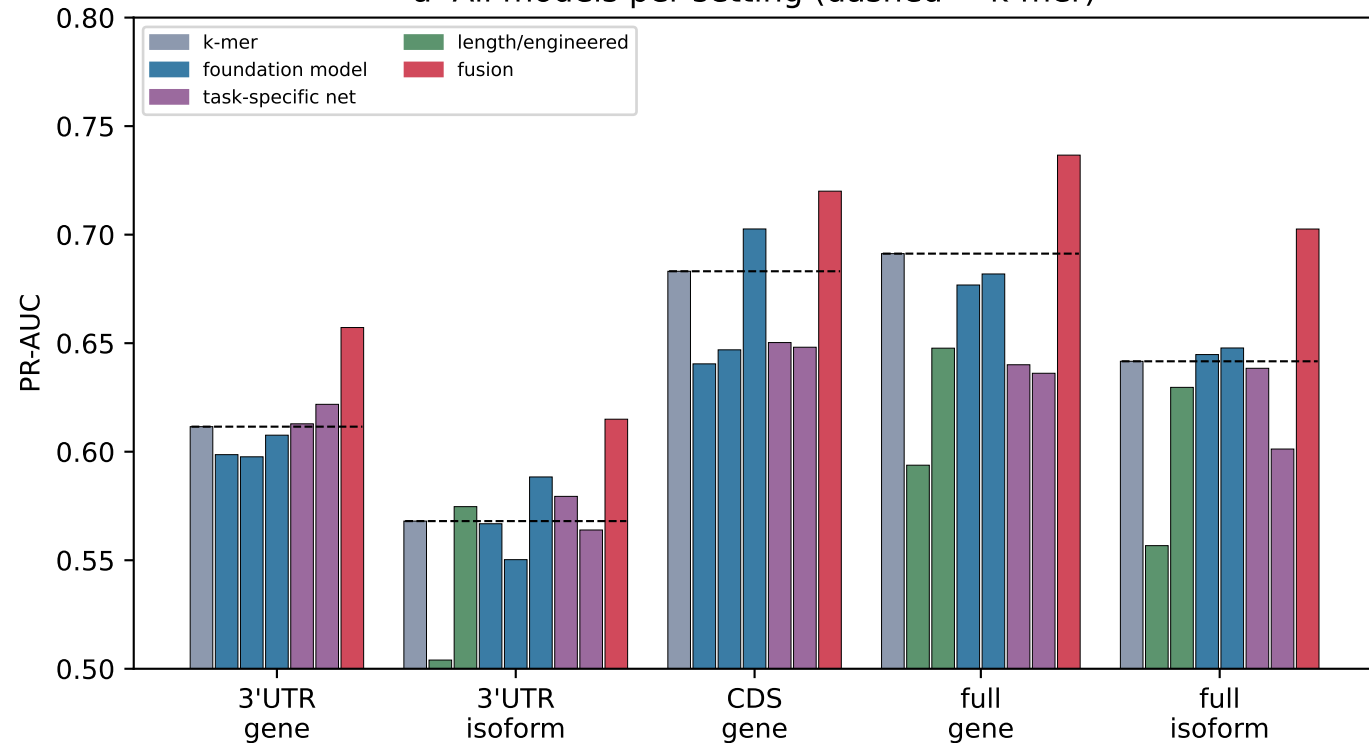
a All models per setting (dashed = k-mer)
