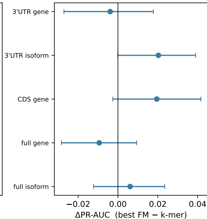
b Foundation models do not beat k-mer
