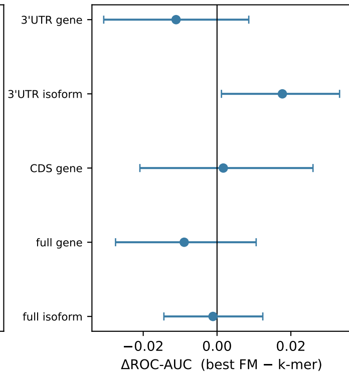
b Foundation models do not beat k-mer
