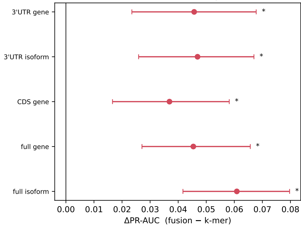
a Fusion vs k-mer (all significant)
