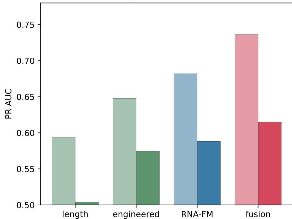
b Component decomposition (light=full, dark=3'UTR iso)
