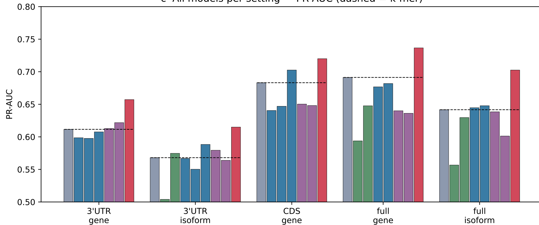
c All models per setting — PR-AUC (dashed = k-mer)
