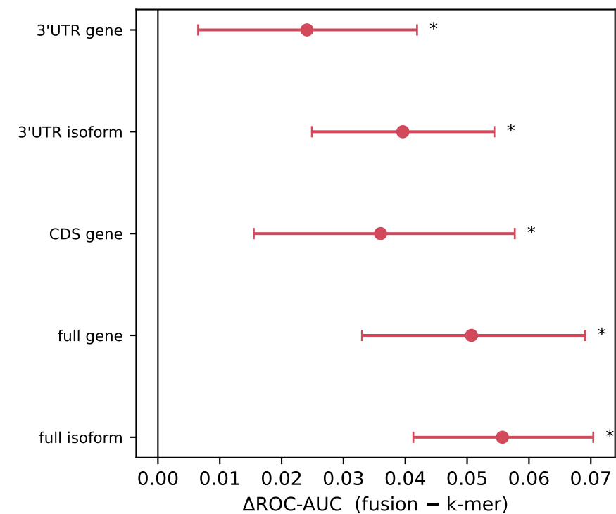
d Fusion vs k-mer
