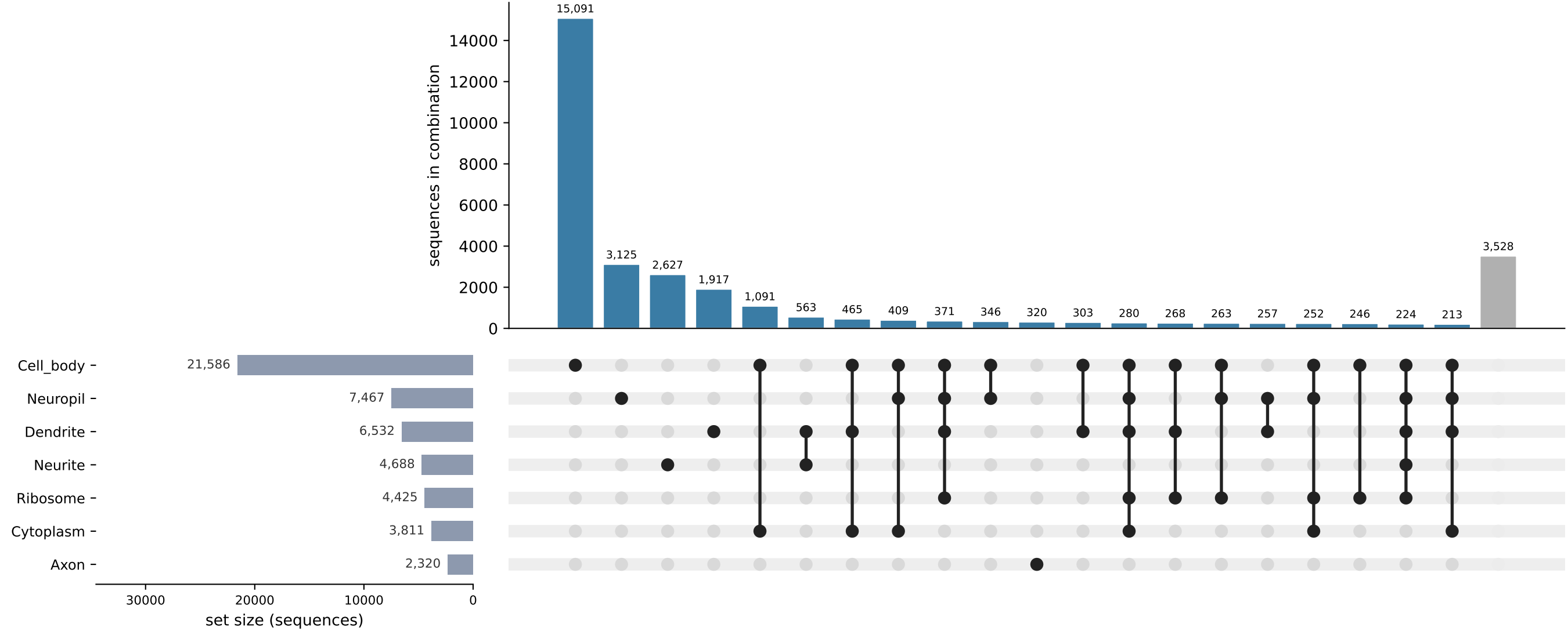
d Compartment co-occurrence (UpSet) — top 20 of 104 combinations (89%; grey = other 84)
