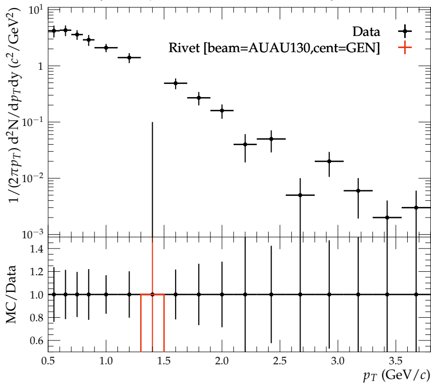
Invariant yields of \bar{p} in each event at 60-92% centrality
