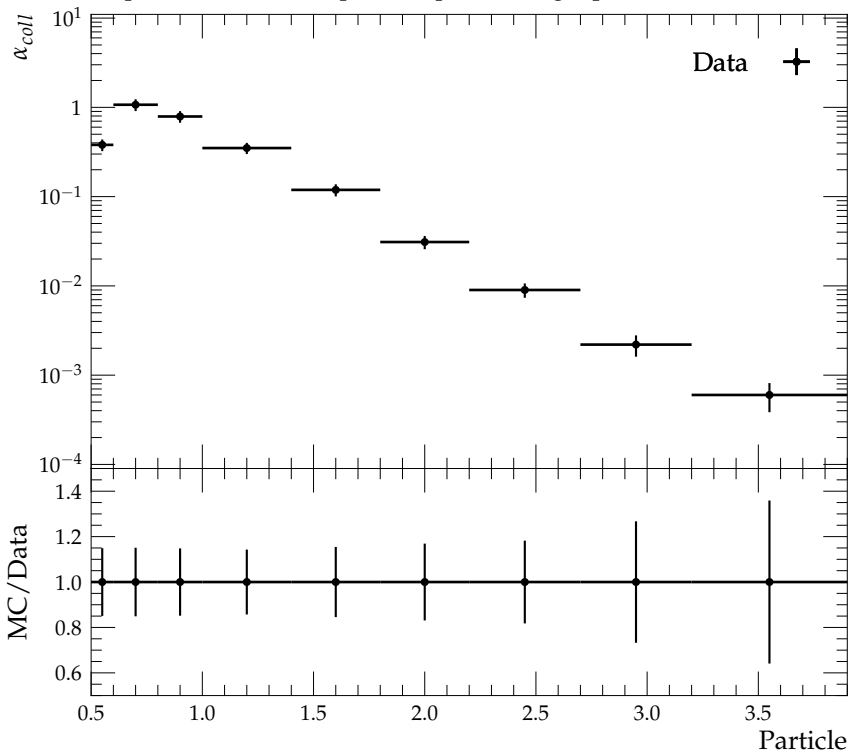
Fit parameters for each particle species using Eqs (19) and (20).
