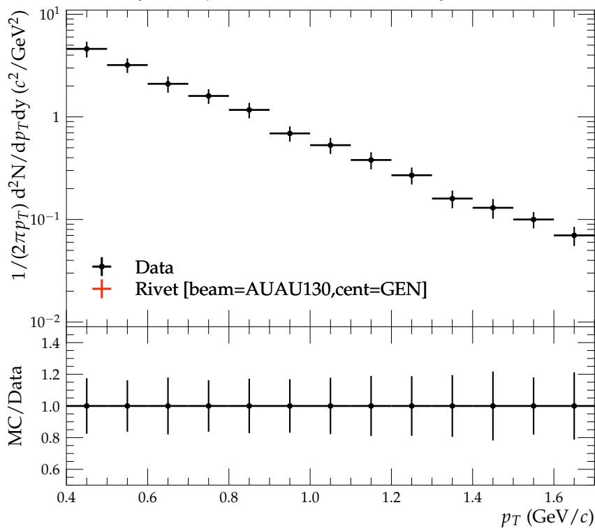
Invariant yields of \bar{p} in each event at 0-5% centrality
