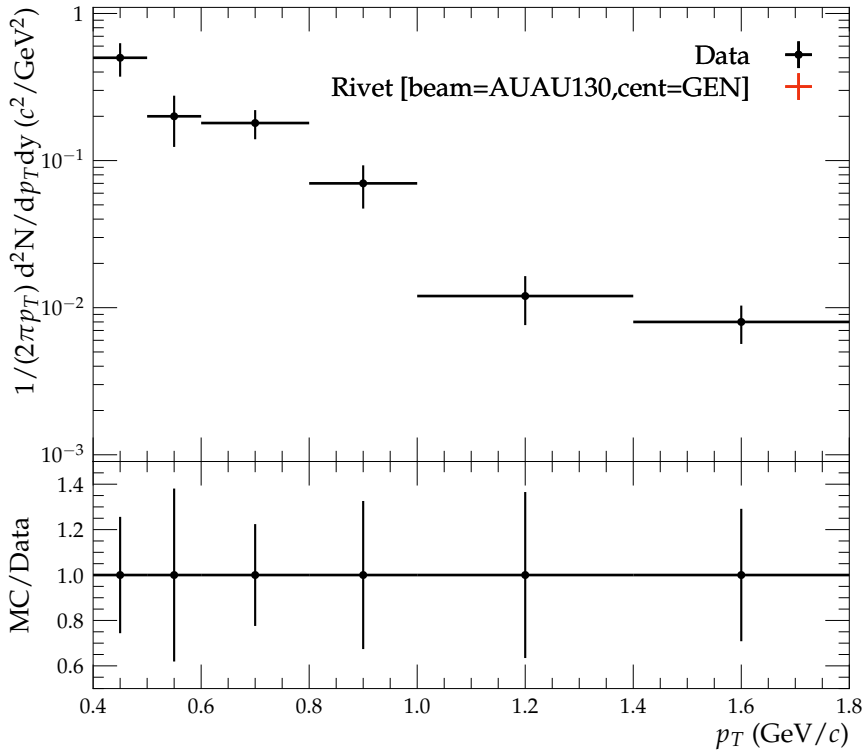
Invariant yields of \bar{p} in each event at 30-60% centrality
