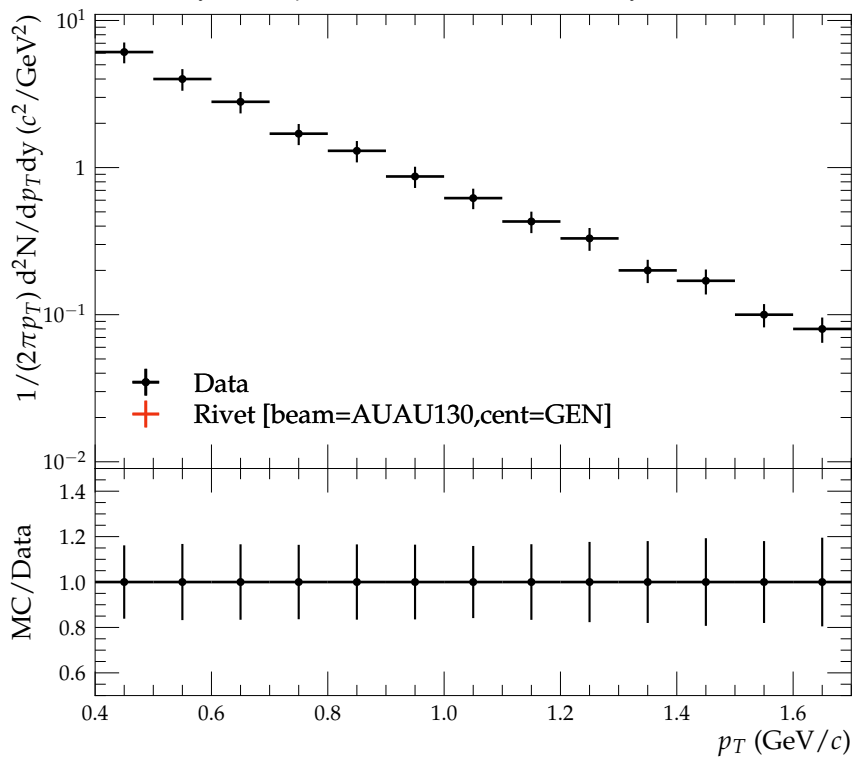
Invariant yields of p in each event at 0-5% centrality
