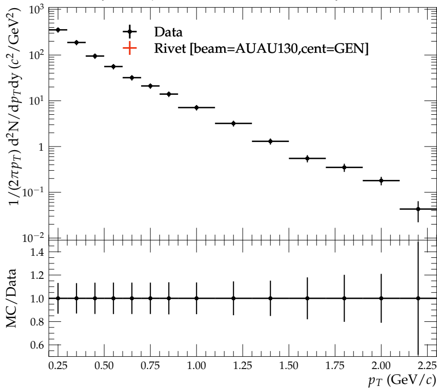
Invariant yields of p in each event at 15-30% centrality
