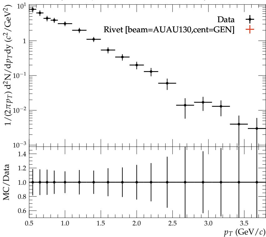
Invariant yields of p in each event at 60-92% centrality
