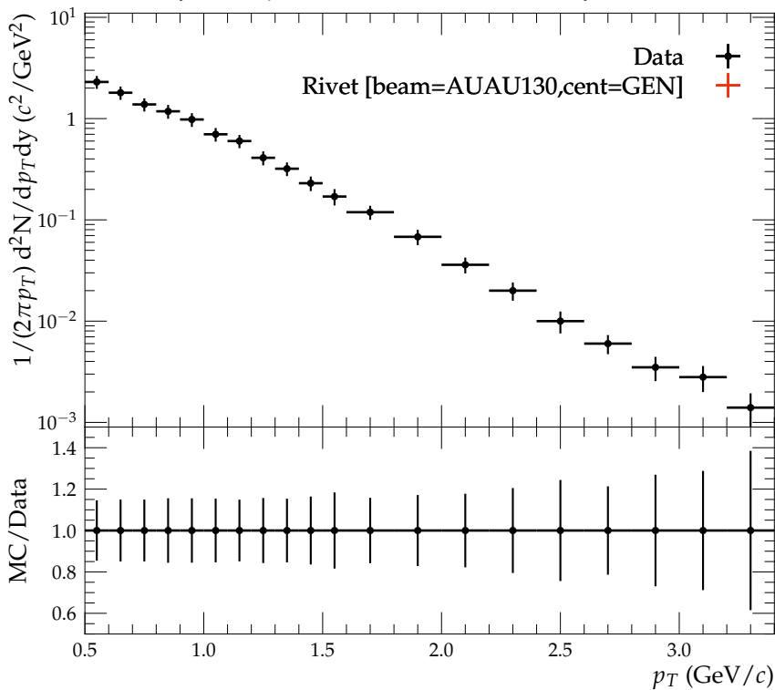
Invariant yields of p in each event at 5-15% centrality
