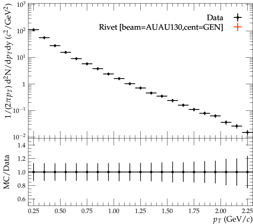
Invariant yields of K^+ in each event at 60-92% centrality
