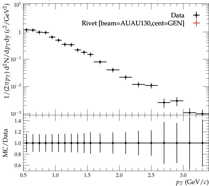
Invariant yields of \bar{p} in each event at 5-15% centrality
