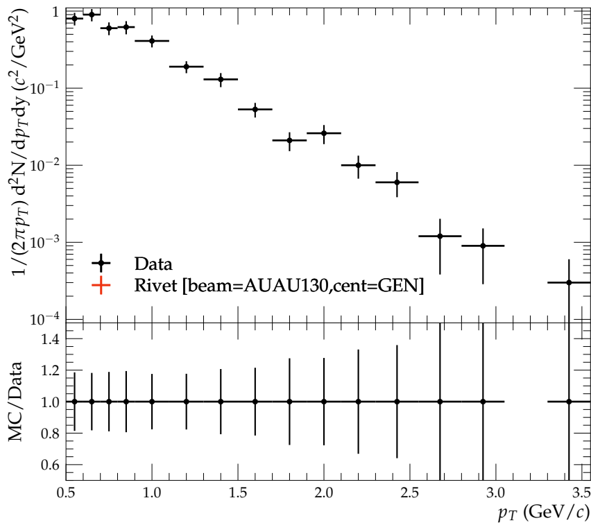
Invariant yields for \pi^+ at 60-92% centrality
