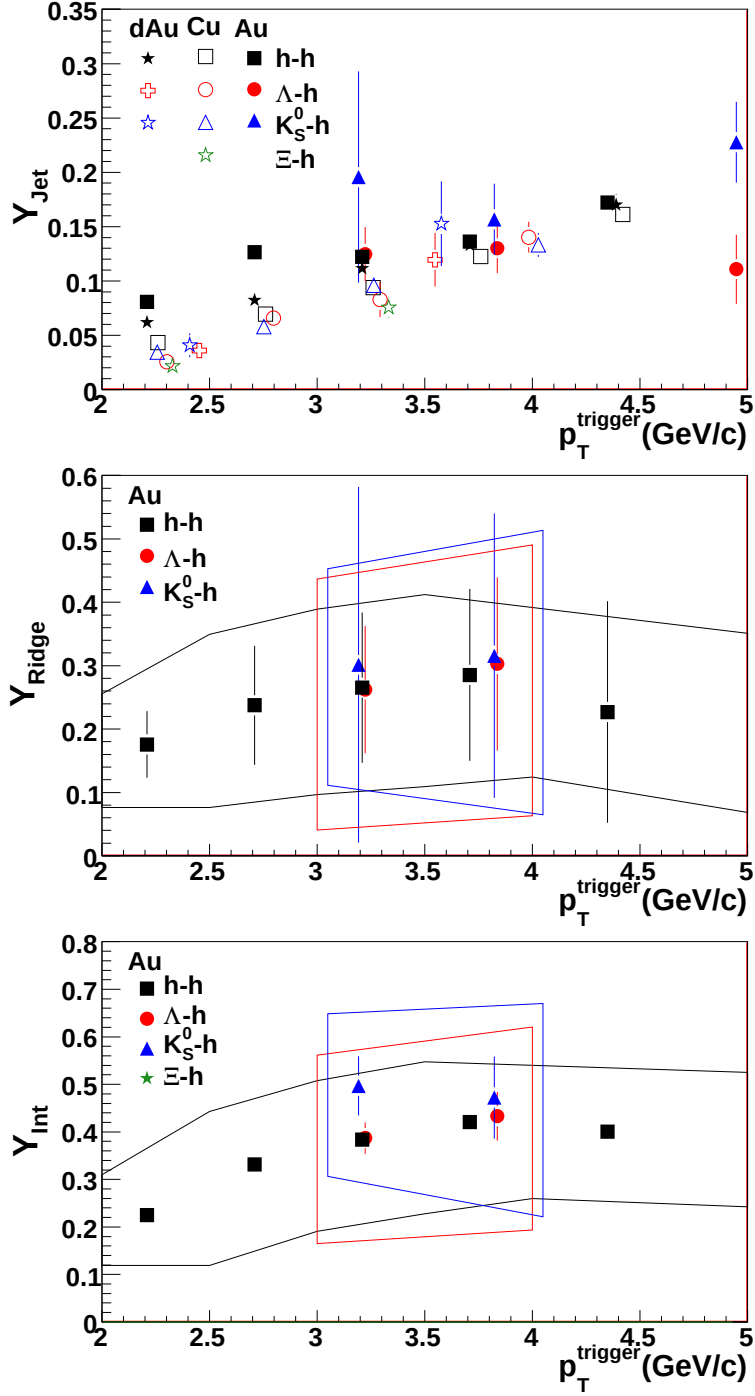
Figure F.1: p_T^{trigger} dependence of Y_{Jet} for 1.5 \text{ GeV/c} < p_T^{associated} < p_T^{trigger} in 0-60% central Cu + Cu and 0-12% central Au + Au collisions at \sqrt{s_{NN}} = 200 \text{ GeV} for unidentified hadrons, \Lambda , K_S^0 , and \Xi trigger particles. The identified trigger particle data have been horizontally offset for visibility.
