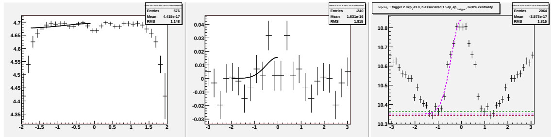
Figure F.34: Going left to right/top to bottom (a) jet-like correlation using \Delta\eta method (b) jet-like correlation using \Delta\phi method (c) correlation integrated over |\Delta\eta| < 0.75 (d) correlation integrated over 0.75 < |\Delta\eta| < 1.75 (e) correlation integrated over 0 < |\Delta\eta| < 1.75 (f) 1-D correlation for 2.0 < p_T^{trigger} < 3.0 GeV/c and 1.5 < p_T^{associated} < p_T^{trigger} GeV/c for \Xi^- and \Xi^+ trigger particles.
