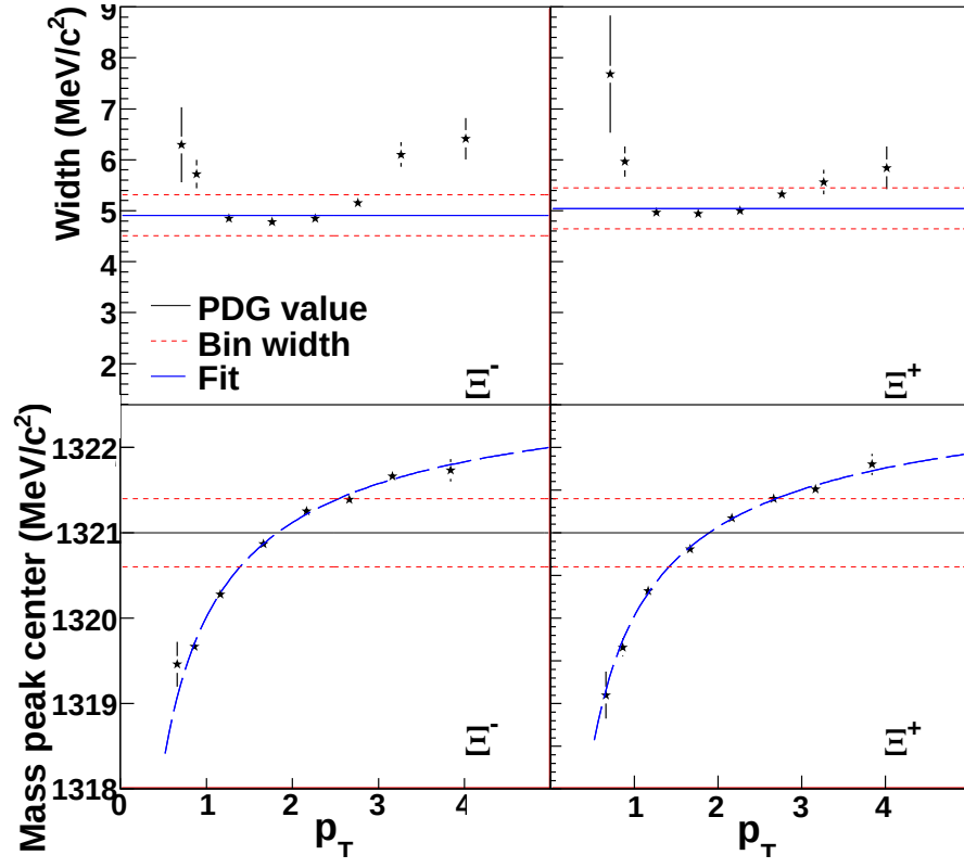
Figure 1.9: Centers of \Xi mass peaks as determined from fits of the mass peaks to a Breit-Wigner distribution
