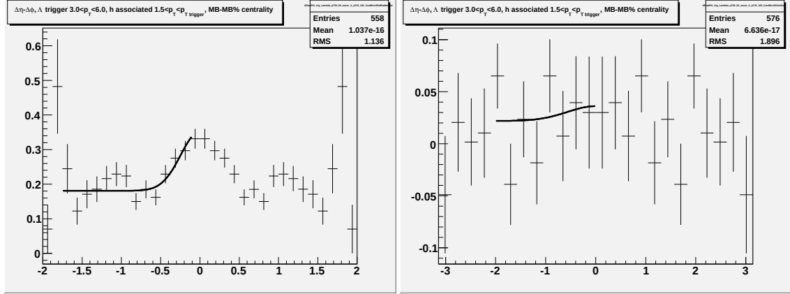
Figure G.31: Going left to right/top to bottom (a) jet-like correlation using \Delta\eta method (b) jet-like correlation using \Delta\phi method (c) correlation integrated over |\Delta\eta| < 0.75 (d) correlation integrated over 0.75 < |\Delta\eta| < 1.75 (e) correlation integrated over 0 < |\Delta\eta| < 1.75 (f) 1-D correlation for 3.0 < p_T^{trigger} < 6.0 GeV/c and 1.5 < p_T^{associated} < p_T^{trigger} GeV/c for \Lambda + \bar{\Lambda} triggers for minimum bias d + Au collisions at \sqrt{s_{NN}} = 200 GeV.
