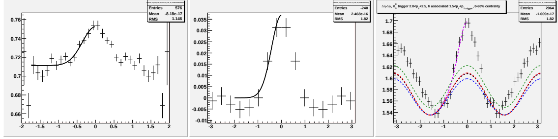
Figure F.20: Going left to right/top to bottom (a) jet-like correlation using \Delta\eta method (b) jet-like correlation using \Delta\phi method (c) correlation integrated over |\Delta\eta| < 0.75 (d) correlation integrated over 0.75 < |\Delta\eta| < 1.75 (e) correlation integrated over 0 < |\Delta\eta| < 1.75 (f) 1-D correlation for 2.0 < p_T^{trigger} < 2.5 GeV/c and 1.5 < p_T^{associated} < p_T^{trigger} GeV/c for K_S^0 trigger particles.
