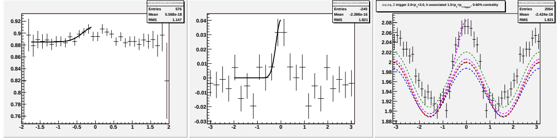
Figure F.24: Going left to right/top to bottom (a) jet-like correlation using \Delta\eta method (b) jet-like correlation using \Delta\phi method (c) correlation integrated over |\Delta\eta| < 0.75 (d) correlation integrated over 0.75 < |\Delta\eta| < 1.75 (e) correlation integrated over 0 < |\Delta\eta| < 1.75 (f) 1-D correlation for 2.0 < p_T^{trigger} < 3.0 GeV/c and 1.5 < p_T^{associated} < p_T^{trigger} GeV/c for \Xi^- and \Xi^+ trigger particles.
