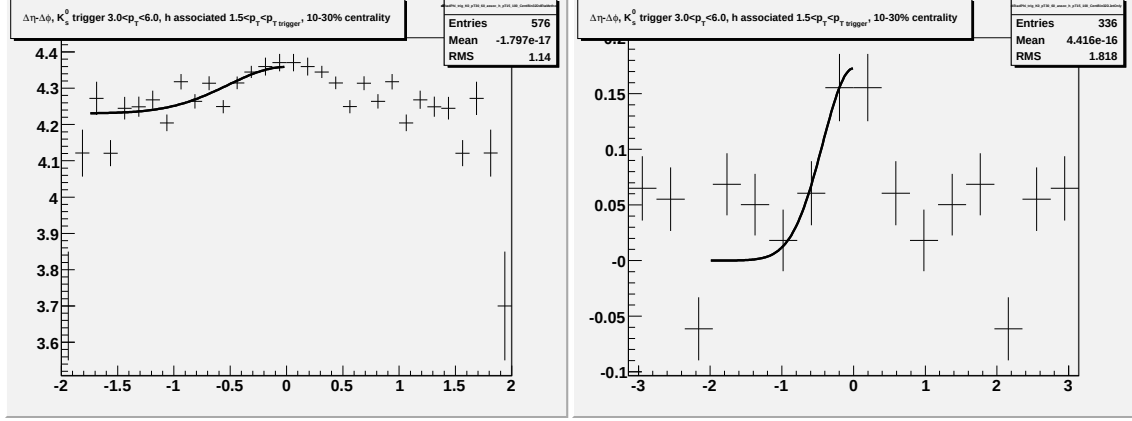
Figure G.27: Going left to right/top to bottom (a) jet-like correlation using \Delta\eta method (b) jet-like correlation using \Delta\phi method (c) correlation integrated over |\Delta\eta| < 0.75 (d) correlation integrated over 0.75 < |\Delta\eta| < 1.75 (e) correlation integrated over 0 < |\Delta\eta| < 1.75 (f) 1-D correlation for 2.0 < p_T^{trigger} < 2.5 GeV/c and 1.5 < p_T^{associated} < p_T^{trigger} GeV/c for K_S^0 and \bar{\Lambda} trigger particles.
