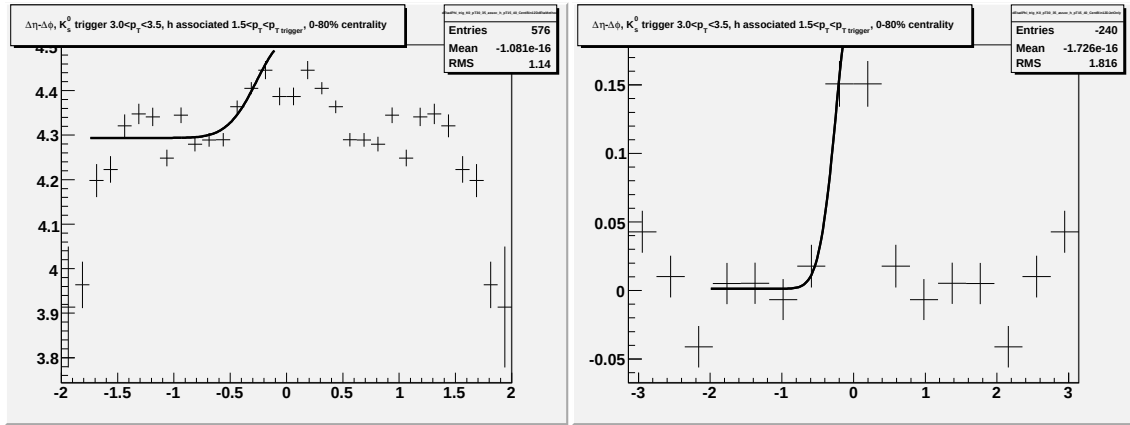
Figure F.46: Going left to right/top to bottom (a) jet-like correlation using \Delta\eta method (b) jet-like correlation using \Delta\phi method (c) correlation integrated over |\Delta\eta| < 0.75 (d) correlation integrated over 0.75 < |\Delta\eta| < 1.75 (e) correlation integrated over 0 < |\Delta\eta| < 1.75 (f) 1-D correlation for 3.0 < p_T^{trigger} < 3.5 GeV/c and 1.5 < p_T^{associated} < p_T^{trigger} GeV/c for K_S^0 trigger particles.
