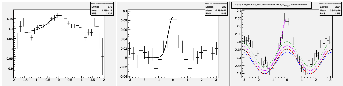
Figure F.25: Going left to right/top to bottom (a) jet-like correlation using \Delta\eta method (b) jet-like correlation using \Delta\phi method (c) correlation integrated over |\Delta\eta| < 0.75 (d) correlation integrated over 0.75 < |\Delta\eta| < 1.75 (e) correlation integrated over 0 < |\Delta\eta| < 1.75 (f) 1-D correlation for 3.0 < p_T^{trigger} < 5.0 GeV/c and 1.5 < p_T^{associated} < p_T^{trigger} GeV/c for \Xi^- and \Xi^+ trigger particles.
