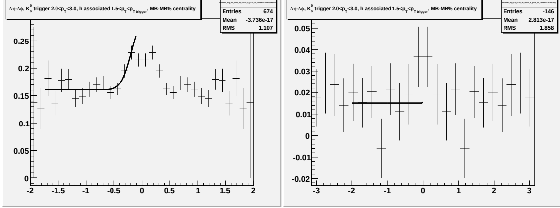
Figure F.57: Going left to right/top to bottom (a) jet-like correlation using \Delta\eta method (b) jet-like correlation using \Delta\phi method (c) correlation integrated over |\Delta\eta| < 0.75 (d) correlation integrated over 0.75 < |\Delta\eta| < 1.75 (e) correlation integrated over 0 < |\Delta\eta| < 1.75 (f) 1-D correlation for 2.0 < p_T^{\text{trigger}} < 2.5 GeV/c and 1.5 < p_T^{\text{associated}} < p_T^{\text{trigger}} GeV/c.
