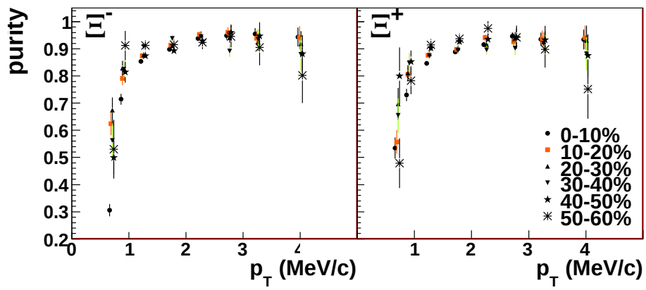
Figure 1.10: \Xi center
