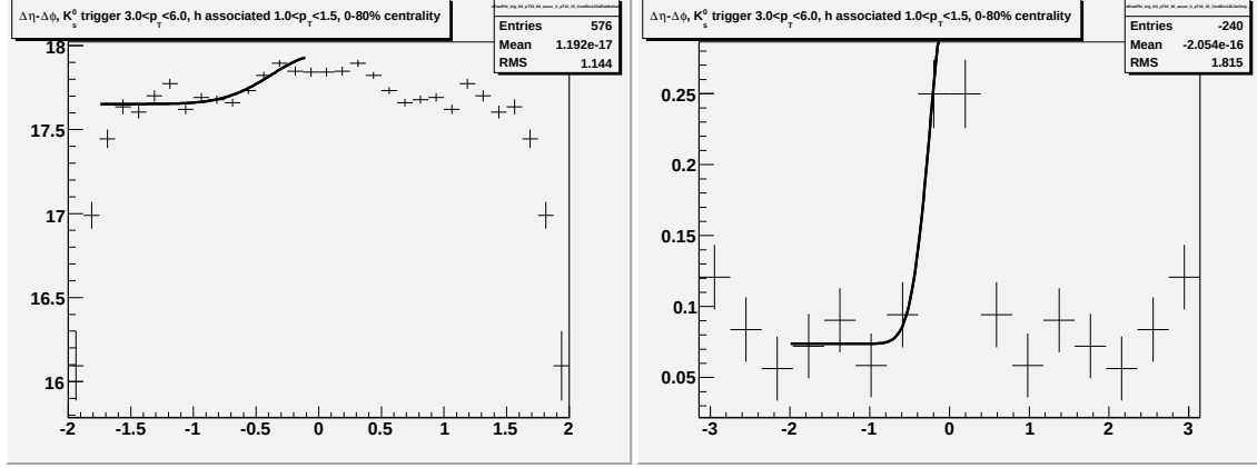
Figure H.14: Going left to right/top to bottom (a) jet-like correlation using \Delta\eta method (b) jet-like correlation using \Delta\phi method (c) correlation integrated over |\Delta\eta| < 0.75 (d) correlation integrated over 0.75 < |\Delta\eta| < 1.75 (e) correlation integrated over 0 < |\Delta\eta| < 1.75 (f) 1-D correlation for 3.0 < p_T^{trigger} < 6.0 GeV/c and 1.0 < p_T^{associated} < 1.5 GeV/c for K_S^0 trigger particles.
