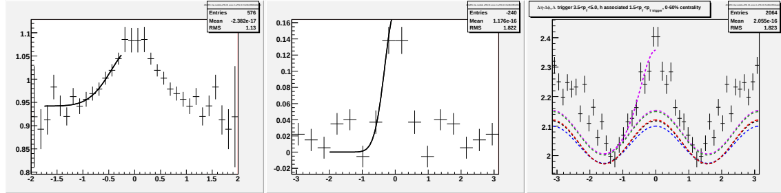
Figure F.19: Going left to right/top to bottom (a) jet-like correlation using \Delta\eta method (b) jet-like correlation using \Delta\phi method (c) correlation integrated over |\Delta\eta| < 0.75 (d) correlation integrated over 0.75 < |\Delta\eta| < 1.75 (e) correlation integrated over 0 < |\Delta\eta| < 1.75 (f) 1-D correlation for 3.5 < p_T^{trigger} < 5.0 GeV/c and 1.5 < p_T^{associated} < p_T^{trigger} GeV/c for \Lambda and \bar{\Lambda} trigger particles.
