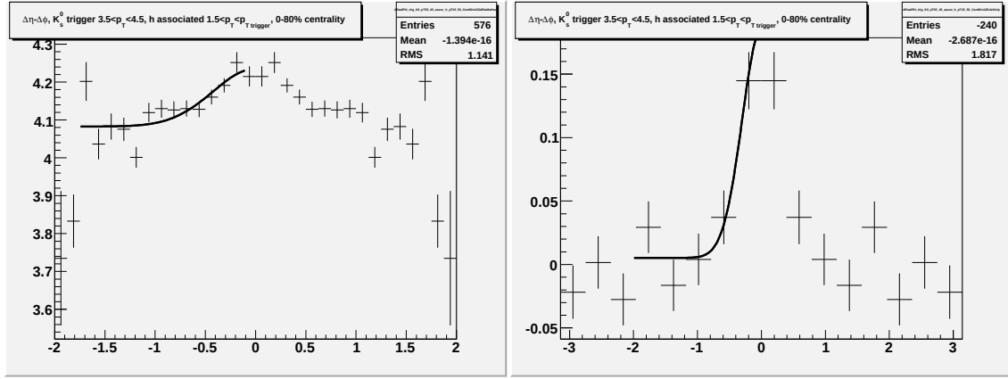
Figure F.47: Going left to right/top to bottom (a) jet-like correlation using \Delta\eta method (b) jet-like correlation using \Delta\phi method (c) correlation integrated over |\Delta\eta| < 0.75 (d) correlation integrated over 0.75 < |\Delta\eta| < 1.75 (e) correlation integrated over 0 < |\Delta\eta| < 1.75 (f) 1-D correlation for 3.5 < p_T^{trigger} < 4.5 GeV/c and 1.5 < p_T^{associated} < p_T^{trigger} GeV/c for K_S^0 trigger particles.
