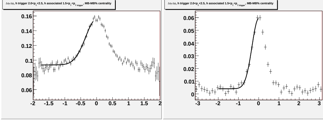
Figure F.48: Going left to right/top to bottom (a) jet-like correlation using \Delta\eta method (b) jet-like correlation using \Delta\phi method (c) correlation integrated over |\Delta\eta| < 0.75 (d) correlation integrated over 0.75 < |\Delta\eta| < 1.75 (e) correlation integrated over 0 < |\Delta\eta| < 1.75 (f) 1-D correlation for 2.0 < p_T^{trigger} < 2.5 GeV/c and 1.5 < p_T^{associated} < p_T^{trigger} GeV/c.
