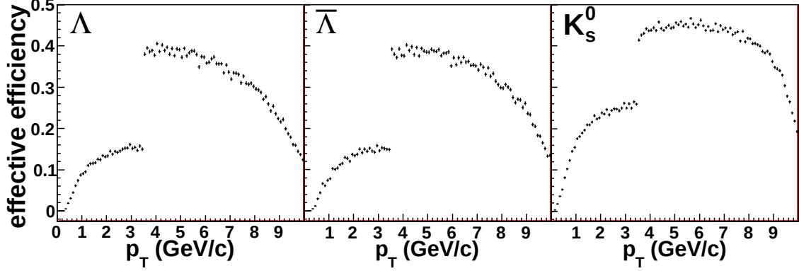
Figure 1.6: Sample effective V^0 reconstruction efficiency for the default cuts listed in Table 1.2.
