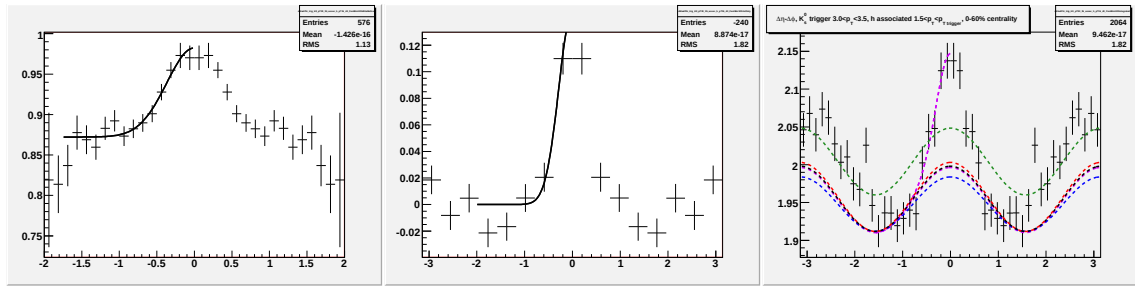
Figure F.22: Going left to right/top to bottom (a) jet-like correlation using \Delta\eta method (b) jet-like correlation using \Delta\phi method (c) correlation integrated over |\Delta\eta| < 0.75 (d) correlation integrated over 0.75 < |\Delta\eta| < 1.75 (e) correlation integrated over 0 < |\Delta\eta| < 1.75 (f) 1-D correlation for 2.0 < p_T^{trigger} < 2.5 GeV/c and 1.5 < p_T^{associated} < p_T^{trigger} GeV/c for K_S^0 trigger particles.
