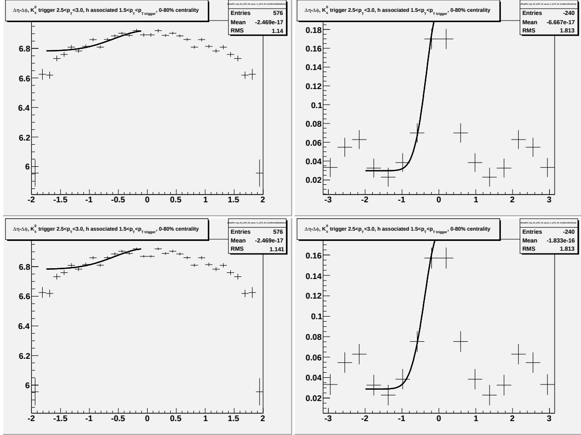
Figure F.41: Going left to right/top to bottom (a) jet-like correlation using \Delta\eta method (b) jet-like correlation using \Delta\phi method (c) correlation integrated over |\Delta\eta| < 0.75 (d) correlation integrated over 0.75 < |\Delta\eta| < 1.75 (e) correlation integrated over 1.75 < |\Delta\eta| < 2.75 (f) 1-D correlation for 2.5 < p_T^{\text{trigger}} < 3.0 GeV/c and 1.5 < p_T^{\text{associated}} < p_T^{\text{trigger}} GeV/c for K_S^0 trigger particles.
