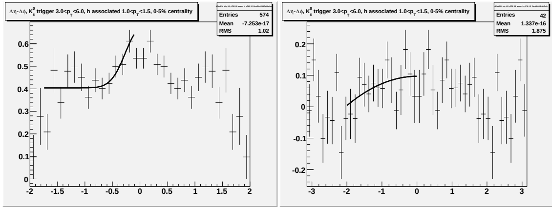
Figure H.23: Going left to right/top to bottom (a) jet-like correlation using \Delta\eta method (b) jet-like correlation using \Delta\phi method (c) correlation integrated over |\Delta\eta| < 0.75 (d) correlation integrated over 0.75 < |\Delta\eta| < 1.75 (e) correlation integrated over 0 < |\Delta\eta| < 1.75 (f) 1-D correlation for 3.0 < p_T^{trigger} < 6.0 GeV/c and 1.0 < p_T^{associated} < 1.5 GeV/c.
