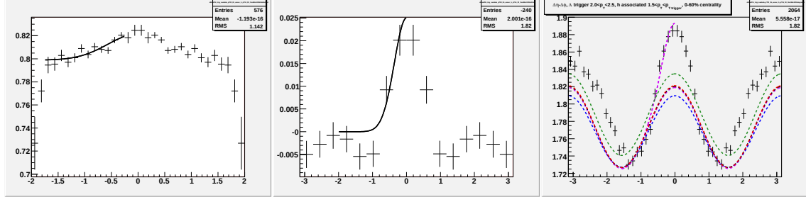
Figure F.16: Going left to right/top to bottom (a) jet-like correlation using \Delta\eta method (b) jet-like correlation using \Delta\phi method (c) correlation integrated over |\Delta\eta| < 0.75 (d) correlation integrated over 0.75 < |\Delta\eta| < 1.75 (e) correlation integrated over 0 < |\Delta\eta| < 1.75 (f) 1-D correlation for 2.0 < p_T^{trigger} < 2.5 GeV/c and 1.5 < p_T^{associated} < p_T^{trigger} GeV/c for \Lambda and \bar{\Lambda} trigger particles.
