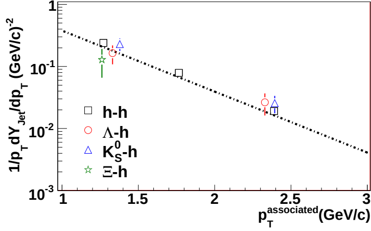
Figure 3.2: p_T^{associated} dependence of Y_{Jet} for 3.0 < p_T^{trigger} < 6.0 GeV/c in 0-60% central Cu + Cu collisions at \sqrt{s_{NN}} = 200 GeV for unidentified hadrons, \Lambda , K_S^0 , and \Xi trigger particles. The line is from a fit of the h-h data to Ae^{-p_T/k} . The identified trigger particle data have been horizontally offset for visibility.
