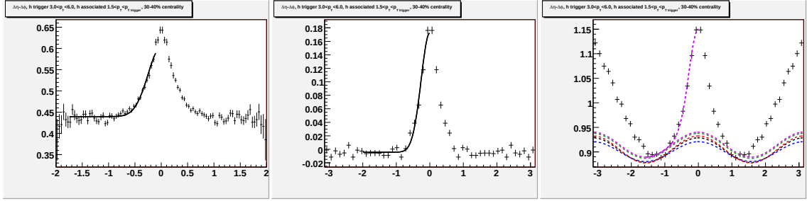
Figure G.5: Going left to right/top to bottom (a) jet-like correlation using \Delta\eta method (b) jet-like correlation using \Delta\phi method (c) correlation integrated over |\Delta\eta| < 0.75 (d) correlation integrated over 0.75 < |\Delta\eta| < 1.75 (e) correlation integrated over 0 < |\Delta\eta| < 1.75 (f) 1-D correlation for 3.0 < p_T^{trigger} < 6.0 GeV/c and 1.5 < p_T^{associated} < p_T^{trigger} GeV/c for 30-40% Cu + Cu collisions at \sqrt{s_{NN}} = 200 GeV.
