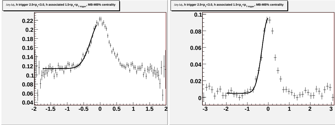
Figure F.49: Going left to right/top to bottom (a) jet-like correlation using \Delta\eta method (b) jet-like correlation using \Delta\phi method (c) correlation integrated over |\Delta\eta| < 0.75 (d) correlation integrated over 0.75 < |\Delta\eta| < 1.75 (e) correlation integrated over 0 < |\Delta\eta| < 1.75 (f) 1-D correlation for 2.5 < p_T^{trigger} < 3.0 GeV/c and 1.5 < p_T^{associated} < p_T^{trigger} GeV/c.
