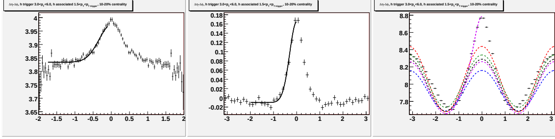
Figure G.9: Going left to right/top to bottom (a) jet-like correlation using \Delta\eta method (b) jet-like correlation using \Delta\phi method (c) correlation integrated over |\Delta\eta| < 0.75 (d) correlation integrated over 0.75 < |\Delta\eta| < 1.75 (e) correlation integrated over 0 < |\Delta\eta| < 1.75 (f) 1-D correlation for 3.0 < p_T^{trigger} < 6.0 GeV/c and 1.5 < p_T^{associated} < p_T^{trigger} GeV/c for 10-20% Au + Au collisions at \sqrt{s_{NN}} = 200 GeV.
