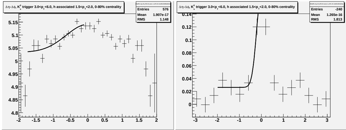
Figure H.15: Going left to right/top to bottom (a) jet-like correlation using \Delta\eta method (b) jet-like correlation using \Delta\phi method (c) correlation integrated over |\Delta\eta| < 0.75 (d) correlation integrated over 0.75 < |\Delta\eta| < 1.75 (e) correlation integrated over 0 < |\Delta\eta| < 1.75 (f) 1-D correlation for 3.0 < p_T^{trigger} < 6.0 GeV/c and 1.5 < p_T^{associated} < 2.0 GeV/c for K_S^0 trigger particles.
