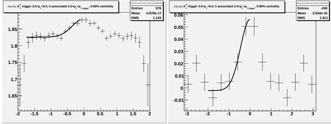
Figure H.16: Going left to right/top to bottom (a) jet-like correlation using \Delta\eta method (b) jet-like correlation using \Delta\phi method (c) correlation integrated over |\Delta\eta| < 0.75 (d) correlation integrated over 0.75 < |\Delta\eta| < 1.75 (e) correlation integrated over 0 < |\Delta\eta| < 1.75 (f) 1-D correlation for 3.0 < p_T^{trigger} < 6.0 GeV/c and 2.0 < p_T^{associated} < 3.0 GeV/c for K_S^0 trigger particles.
