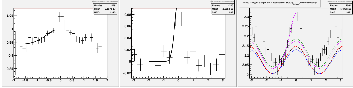
Figure F.18: Going left to right/top to bottom (a) jet-like correlation using \Delta\eta method (b) jet-like correlation using \Delta\phi method (c) correlation integrated over |\Delta\eta| < 0.75 (d) correlation integrated over 0.75 < |\Delta\eta| < 1.75 (e) correlation integrated over 0 < |\Delta\eta| < 1.75 (f) 1-D correlation for 2.0 < p_T^{trigger} < 2.5 GeV/c and 1.5 < p_T^{associated} < p_T^{trigger} GeV/c for \Lambda and \bar{\Lambda} trigger particles.
