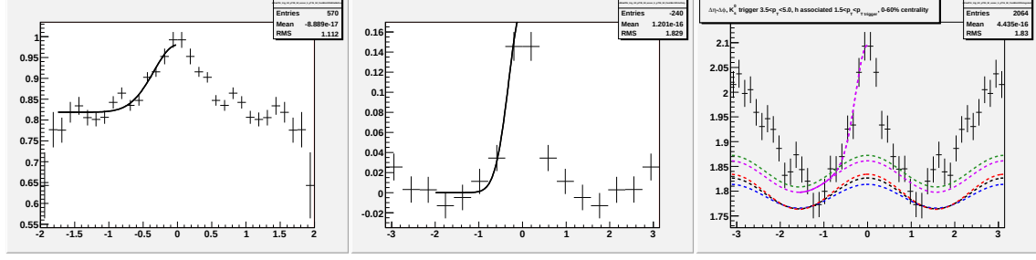
Figure F.23: Going left to right/top to bottom (a) jet-like correlation using \Delta\eta method (b) jet-like correlation using \Delta\phi method (c) correlation integrated over |\Delta\eta| < 0.75 (d) correlation integrated over 0.75 < |\Delta\eta| < 1.75 (e) correlation integrated over 0 < |\Delta\eta| < 1.75 (f) 1-D correlation for 3.5 < p_T^{trigger} < 5.0 GeV/c and 1.5 < p_T^{associated} < p_T^{trigger} GeV/c for K_S^0 trigger particles.
