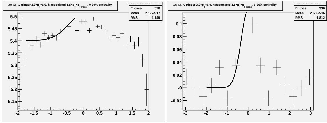
Figure G.22: Going left to right/top to bottom (a) jet-like correlation using \Delta\eta method (b) jet-like correlation using \Delta\phi method (c) correlation integrated over |\Delta\eta| < 0.75 (d) correlation integrated over 0.75 < |\Delta\eta| < 1.75 (e) correlation integrated over 0 < |\Delta\eta| < 1.75 (f) 1-D correlation for 2.0 < p_T^{trigger} < 2.5 GeV/c and 1.5 < p_T^{associated} < p_T^{trigger} GeV/c for \Lambda and \bar{\Lambda} trigger particles.
