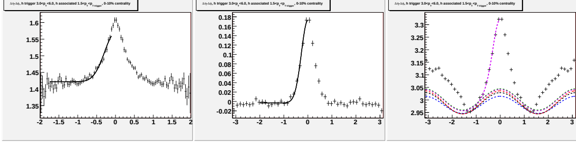
Figure G.2: Going left to right/top to bottom (a) jet-like correlation using \Delta\eta method (b) jet-like correlation using \Delta\phi method (c) correlation integrated over |\Delta\eta| < 0.75 (d) correlation integrated over 0.75 < |\Delta\eta| < 1.75 (e) correlation integrated over 0 < |\Delta\eta| < 1.75 (f) 1-D correlation for 3.0 < p_T^{trigger} < 6.0 GeV/c and 1.5 < p_T^{associated} < p_T^{trigger} GeV/c for 0-10% Cu + Cu collisions at \sqrt{s_{NN}} = 200 GeV.
