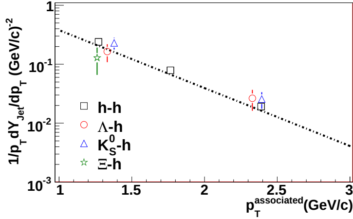
Figure H.1: p_T^{associated} dependence of Y_{Jet} for 3.0 < p_T^{trigger} < 6.0 GeV/c in 0-60% central Cu + Cu collisions at \sqrt{s_{NN}} = 200 GeV for unidentified hadrons, \Lambda , K_S^0 , and \Xi trigger particles. The line is from a fit of the h-h data to Ae^{-p_T/k} . The identified trigger particle data have been horizontally offset for visibility.
