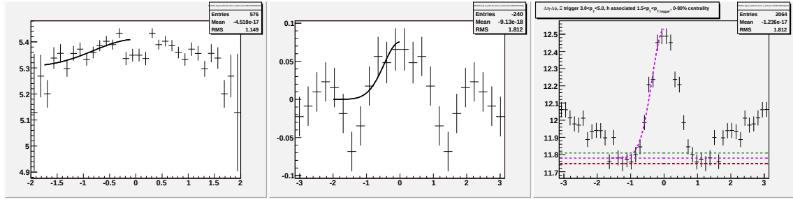
Figure F.35: Going left to right/top to bottom (a) jet-like correlation using \Delta\eta method (b) jet-like correlation using \Delta\phi method (c) correlation integrated over |\Delta\eta| < 0.75 (d) correlation integrated over 0.75 < |\Delta\eta| < 1.75 (e) correlation integrated over 0 < |\Delta\eta| < 1.75 (f) 1-D correlation for 3.0 < p_T^{trigger} < 5.0 GeV/c and 1.5 < p_T^{associated} < p_T^{trigger} GeV/c for \Xi^- and \Xi^+ trigger particles.
