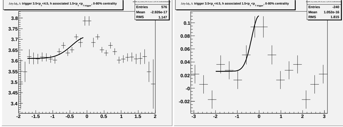
Figure F.45: Going left to right/top to bottom (a) jet-like correlation using \Delta\eta method (b) jet-like correlation using \Delta\phi method (c) correlation integrated over |\Delta\eta| < 0.75 (d) correlation integrated over 0.75 < |\Delta\eta| < 1.75 (e) correlation integrated over 0 < |\Delta\eta| < 1.75 (f) 1-D correlation for 3.5 < p_T^{trigger} < 4.5 GeV/c and 1.5 < p_T^{associated} < p_T^{trigger} GeV/c for \Lambda and \bar{\Lambda} trigger particles.
