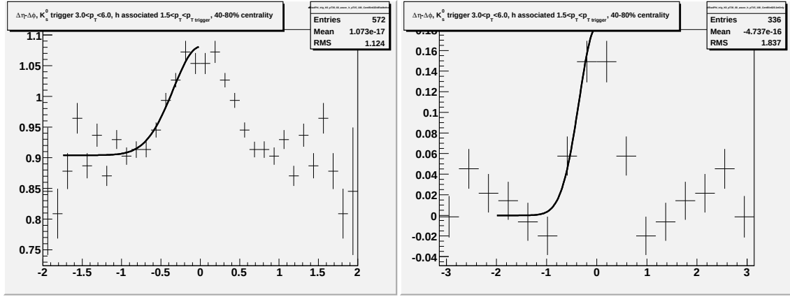
Figure G.29: Going left to right/top to bottom (a) jet-like correlation using \Delta\eta method (b) jet-like correlation using \Delta\phi method (c) correlation integrated over |\Delta\eta| < 0.75 (d) correlation integrated over 0.75 < |\Delta\eta| < 1.75 (e) correlation integrated over 0 < |\Delta\eta| < 1.75 (f) 1-D correlation for 2.0 < p_T^{trigger} < 2.5 GeV/c and 1.5 < p_T^{associated} < p_T^{trigger} GeV/c for K_S^0 and \Lambda trigger particles.
