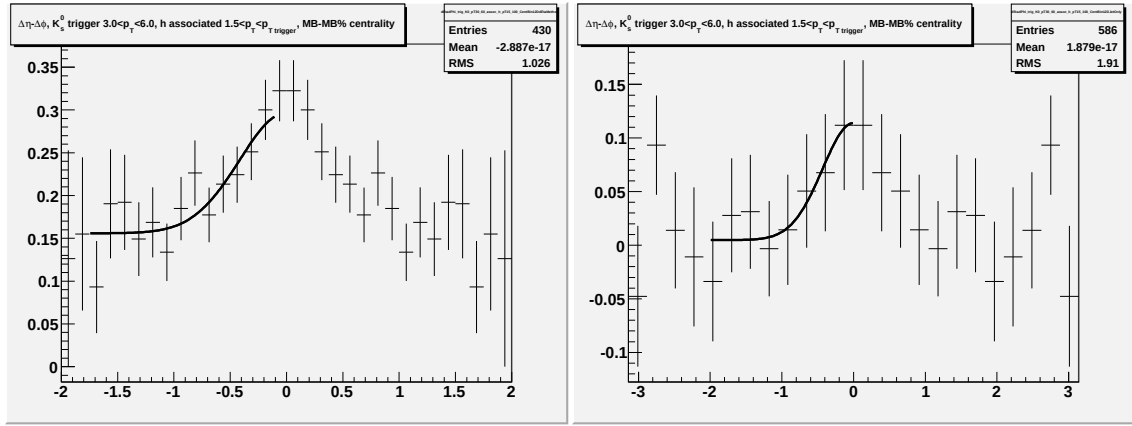
Figure G.32: Going left to right/top to bottom (a) jet-like correlation using \Delta\eta method (b) jet-like correlation using \Delta\phi method (c) correlation integrated over |\Delta\eta| < 0.75 (d) correlation integrated over 0.75 < |\Delta\eta| < 1.75 (e) correlation integrated over 0 < |\Delta\eta| < 1.75 (f) 1-D correlation for 3.0 < p_T^{trigger} < 6.0 GeV/c and 1.5 < p_T^{associated} < p_T^{trigger} GeV/c for K_S^0 triggers for minimum bias d + Au collisions at \sqrt{s_{NN}} = 200 GeV.
