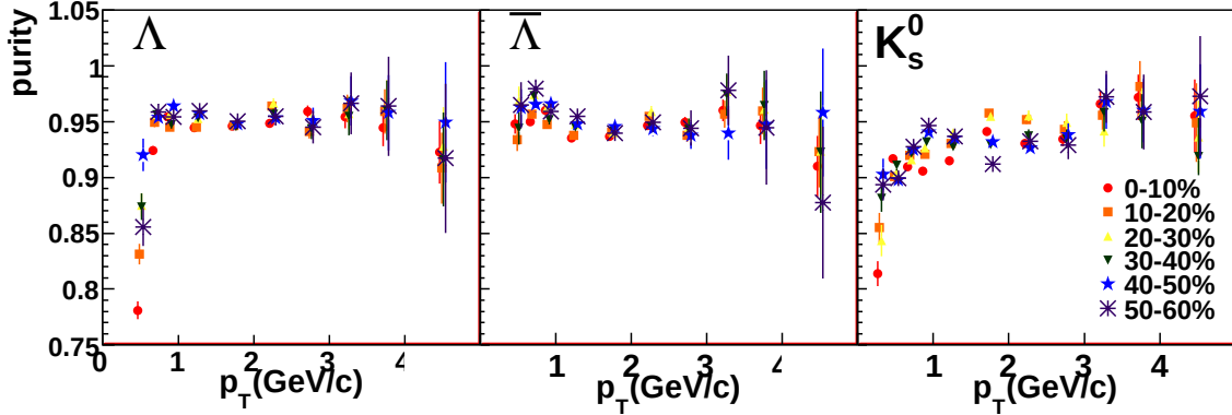
Figure 1.5: V^0 purity as a function of p_T after tuning the geometric cuts.
