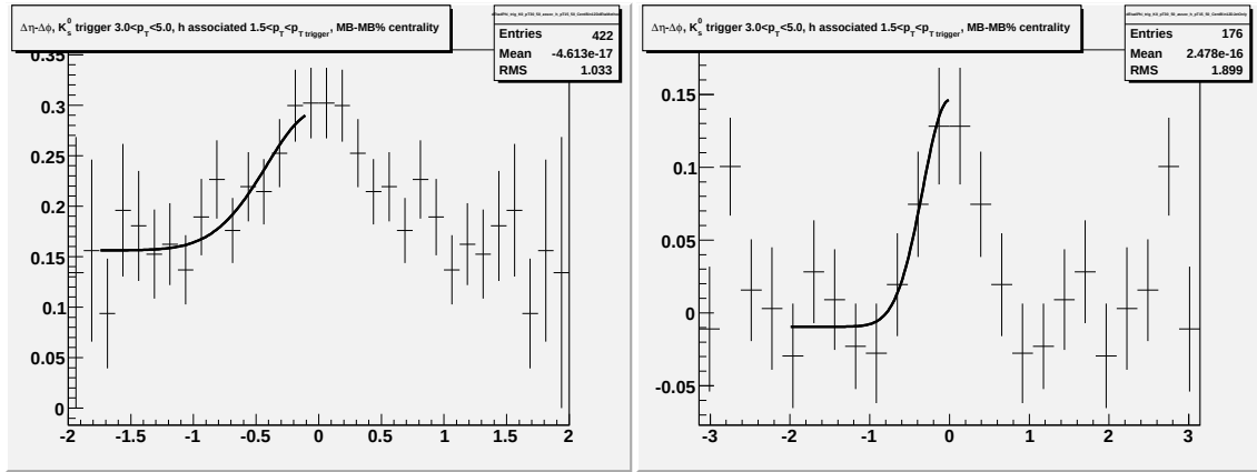
Figure F.58: Going left to right/top to bottom (a) jet-like correlation using \Delta\eta method (b) jet-like correlation using \Delta\phi method (c) correlation integrated over |\Delta\eta| < 0.75 (d) correlation integrated over 0.75 < |\Delta\eta| < 1.75 (e) correlation integrated over 0 < |\Delta\eta| < 1.75 (f) 1-D correlation for 4.0 < p_T^{\text{trigger}} < 5.0 GeV/c and 1.5 < p_T^{\text{associated}} < p_T^{\text{trigger}} GeV/c.
