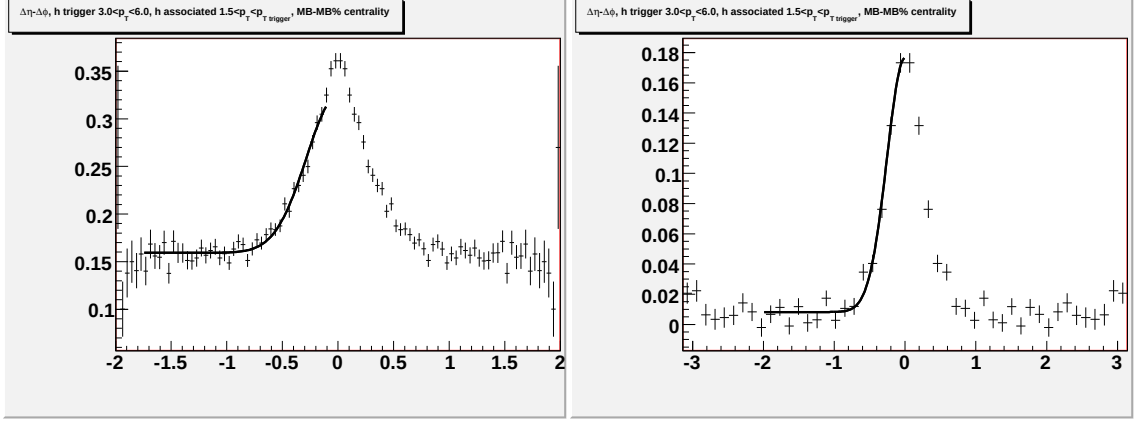
Figure G.30: Going left to right/top to bottom (a) jet-like correlation using \Delta\eta method (b) jet-like correlation using \Delta\phi method (c) correlation integrated over |\Delta\eta| < 0.75 (d) correlation integrated over 0.75 < |\Delta\eta| < 1.75 (e) correlation integrated over 0 < |\Delta\eta| < 1.75 (f) 1-D correlation for 3.0 < p_T^{trigger} < 6.0 GeV/c and 1.5 < p_T^{associated} < p_T^{trigger} GeV/c for minimum bias d + Au collisions at \sqrt{s_{NN}} = 200 GeV.
