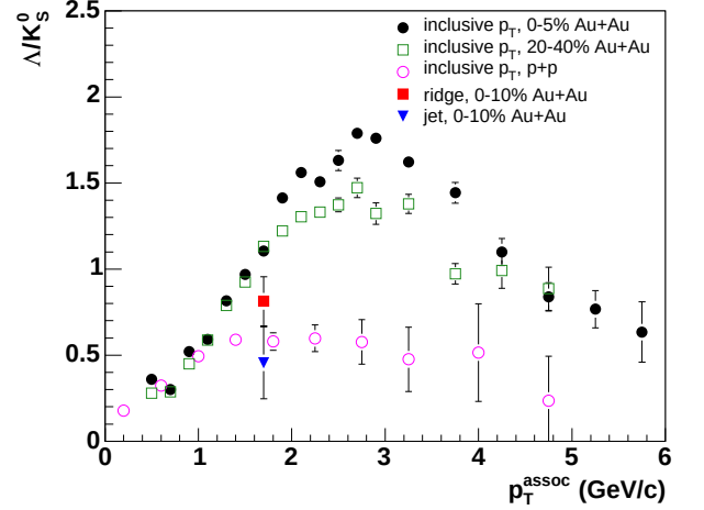
FIG. 8: \Lambda/K_S^0 ratio measured in inclusive p_T distributions, near-side jet-like and ridge-like correlation peaks in Au+Au collisions together with this ratio obtained from inclusive p_T spectra in p+p collisions.
