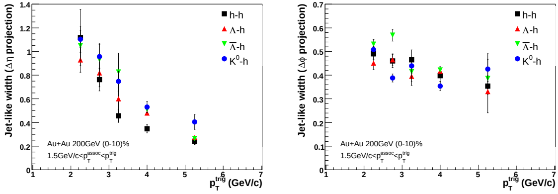
FIG. 5: Dependence of the jet-like peak Gaussian width on p_T^{trig} determined from (a) \Delta\eta and (b) \Delta\phi projections in central Au+Au collisions. Various trigger particle species are described in the legend. Remark: \Lambda and \bar{\Lambda} will be summed together...
