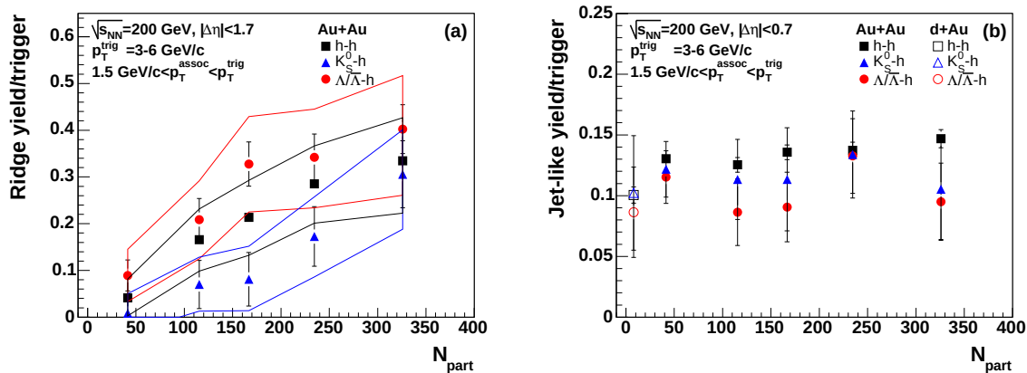
FIG. 4: Centrality dependence of the ridge yield (a) and jet-like yield (b) of associated charged particles for various trigger species in d+Au and Au+Au collisions. The error bands indicate systematic errors on the ridge yield due to the v_2 subtraction.
