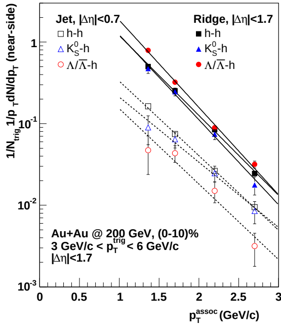
FIG. 7: Invariant p_T distribution of associated charged particles in the jet-like peak and ridge in central Au+Au collisions for various trigger species indicated by the legend. The lines are exponential fits to the data.
