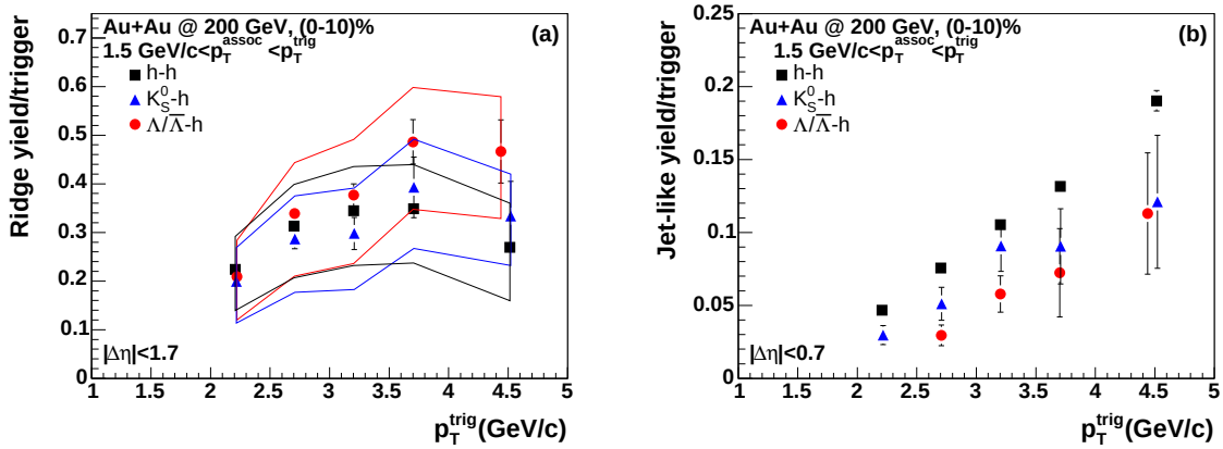
FIG. 6: Dependence of the ridge yield (a) and jet-like yield (b) on p_T^{trig} for various trigger species in central (0-10%) Au+Au collisions. The bands indicate systematic errors on the ridge yield due to the v_2 subtraction.
