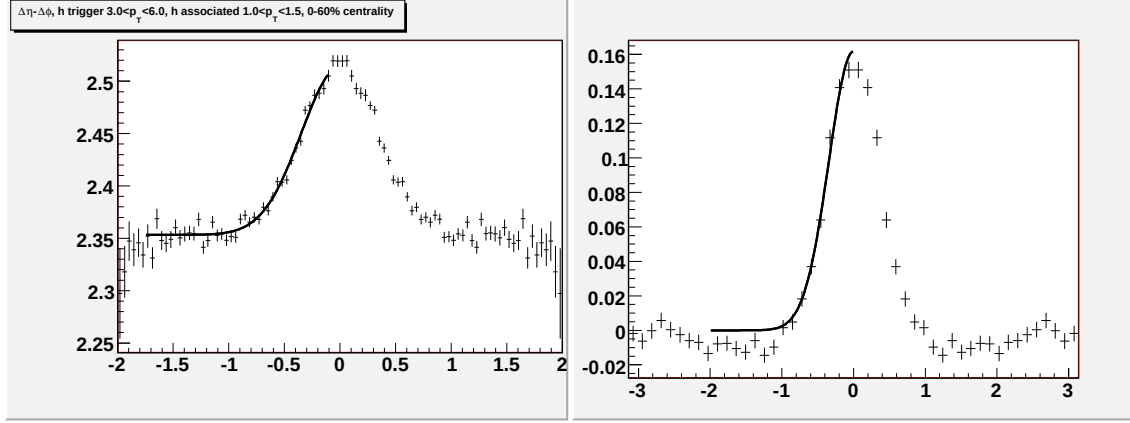
Figure O.4: Going left to right/top to bottom (a) jet-like correlation using \Delta\eta method (b) jet-like correlation using \Delta\phi method (c) correlation integrated over |\Delta\eta| < 0.75 (d) correlation integrated over 0.75 < |\Delta\eta| < 1.75 (e) correlation integrated over 0 < |\Delta\eta| < 1.75 (f) 1-D correlation for 3.0 < p_T^{trigger} < 6.0 GeV/c and 1.0 < p_T^{associated} < 1.5 GeV/c.
