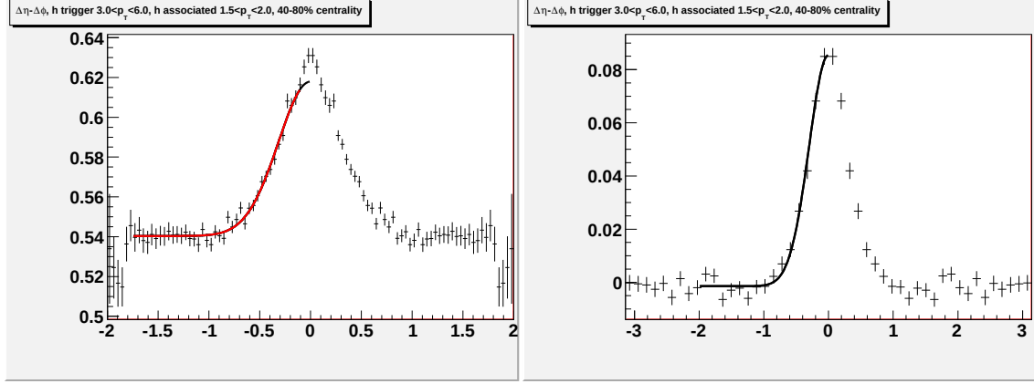
Figure P.2: Going left to right/top to bottom (a) jet-like correlation using \Delta\eta method (b) jet-like correlation using \Delta\phi method (c) correlation integrated over |\Delta\eta| < 0.75 (d) correlation integrated over 0.75 < |\Delta\eta| < 1.75 (e) correlation integrated over 0 < |\Delta\eta| < 1.75 (f) 1-D correlation for 3.0 < p_T^{trigger} < 6.0 GeV/c and 1.5 < p_T^{associated} < 2.0 GeV/c.
