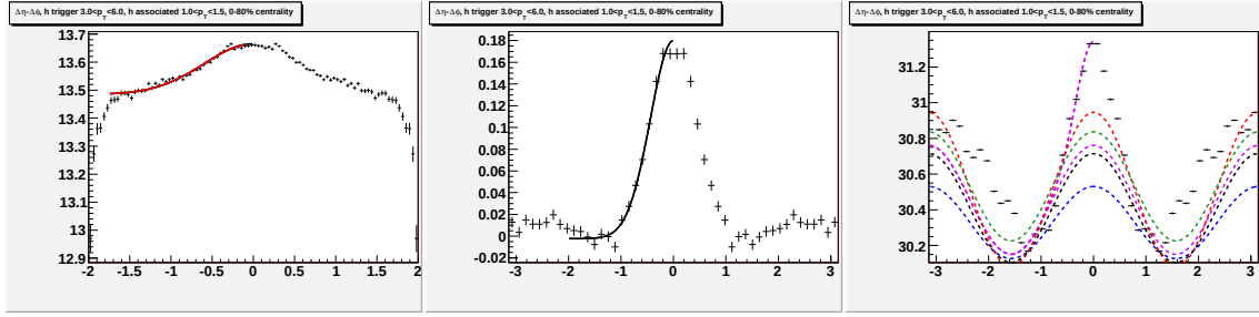
Figure P.4: Going left to right/top to bottom (a) jet-like correlation using \Delta\eta method (b) jet-like correlation using \Delta\phi method (c) correlation integrated over |\Delta\eta| < 0.75 (d) correlation integrated over 0.75 < |\Delta\eta| < 1.75 (e) correlation integrated over 0 < |\Delta\eta| < 1.75 (f) 1-D correlation for 3.0 < p_T^{trigger} < 6.0 GeV/c and 1.0 < p_T^{associated} < 1.5 GeV/c.
