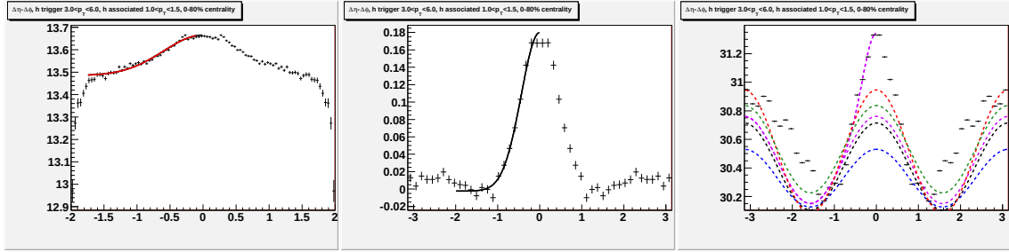
Figure P.10: Going left to right/top to bottom (a) jet-like correlation using \Delta\eta method (b) jet-like correlation using \Delta\phi method (c) correlation integrated over |\Delta\eta| < 0.75 (d) correlation integrated over 0.75 < |\Delta\eta| < 1.75 (e) correlation integrated over 0 < |\Delta\eta| < 1.75 (f) 1-D correlation for 3.0 < p_T^{trigger} < 6.0 GeV/c and 1.0 < p_T^{associated} < 1.5 GeV/c.
