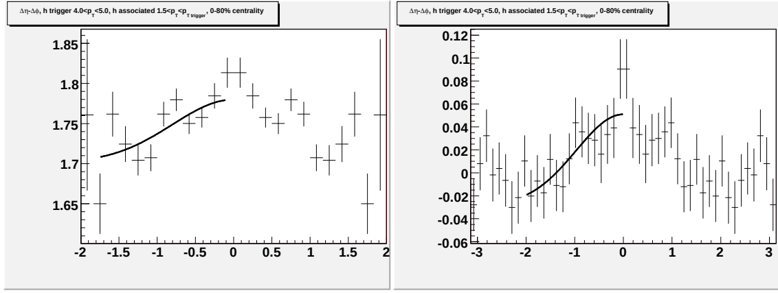
Figure H.4: Going left to right/top to bottom (a) jet-like correlation using \Delta\eta method (b) jet-like correlation using \Delta\phi method (c) correlation integrated over |\Delta\eta| < 0.75 (d) correlation integrated over 0.75 < |\Delta\eta| < 1.75 (e) correlation integrated over 0 < |\Delta\eta| < 1.75 (f) 1-D correlation for 4.0 < p_T^{\text{trigger}} < 5.0 GeV/c and 1.5 < p_T^{\text{associated}} < p_T^{\text{trigger}} GeV/c.
