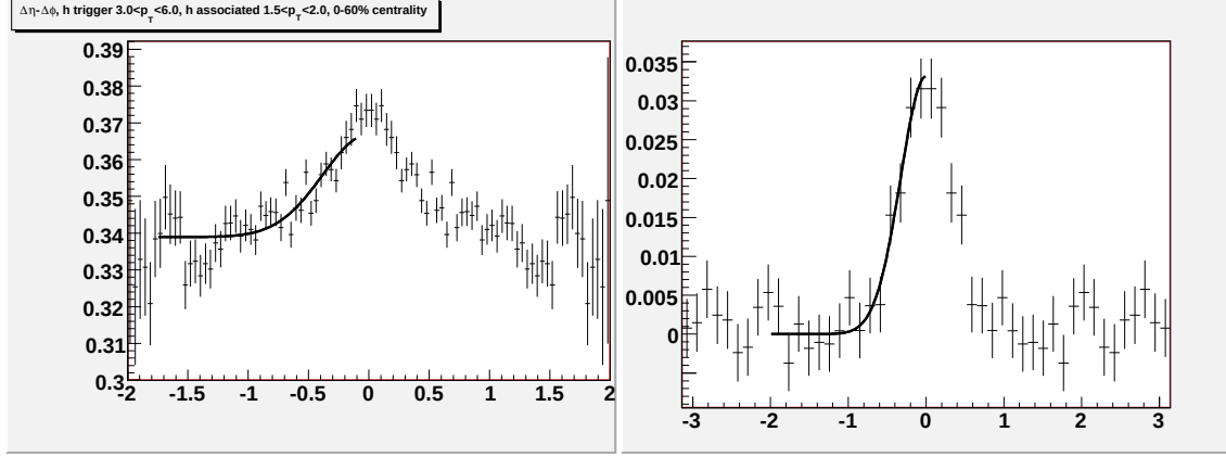
Figure N.2: Going left to right/top to bottom (a) jet-like correlation using \Delta\eta method (b) jet-like correlation using \Delta\phi method (c) correlation integrated over |\Delta\eta| < 0.75 (d) correlation integrated over 0.75 < |\Delta\eta| < 1.75 (e) correlation integrated over 0 < |\Delta\eta| < 1.75 (f) 1-D correlation for 3.0 < p_T^{trigger} < 6.0 GeV/c and 1.5 < p_T^{associated} < 2.0 GeV/c.
