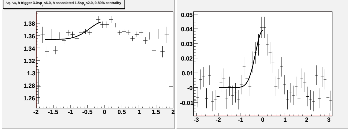
Figure O.2: Going left to right/top to bottom (a) jet-like correlation using \Delta\eta method (b) jet-like correlation using \Delta\phi method (c) correlation integrated over |\Delta\eta| < 0.75 (d) correlation integrated over 0.75 < |\Delta\eta| < 1.75 (e) correlation integrated over 0 < |\Delta\eta| < 1.75 (f) 1-D correlation for 3.0 < p_T^{trigger} < 6.0 GeV/c and 1.5 < p_T^{associated} < 2.0 GeV/c.
