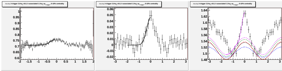
Figure K.1: Going left to right/top to bottom (a) jet-like correlation using \Delta\eta method (b) jet-like correlation using \Delta\phi method (c) correlation integrated over |\Delta\eta| < 0.75 (d) correlation integrated over 0.75 < |\Delta\eta| < 1.75 (e) correlation integrated over 0 < |\Delta\eta| < 1.75 (f) 1-D correlation for 3.0 < p_T^{trigger} < 6.0 GeV/c and 1.5 < p_T^{associated} < p_T^{trigger} GeV/c for 0-10% Cu + Cu collisions at \sqrt{s_{NN}} = 62 GeV.
