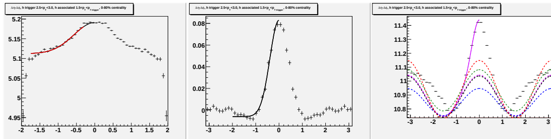
Figure I.9: Going left to right/top to bottom (a) jet-like correlation using \Delta\eta method (b) jet-like correlation using \Delta\phi method (c) correlation integrated over |\Delta\eta| < 0.75 (d) correlation integrated over 0.75 < |\Delta\eta| < 1.75 (e) correlation integrated over 0 < |\Delta\eta| < 1.75 (f) 1-D correlation for 2.5 < p_T^{trigger} < 3.0 GeV/c and 1.5 < p_T^{associated} < p_T^{trigger} GeV/c.
