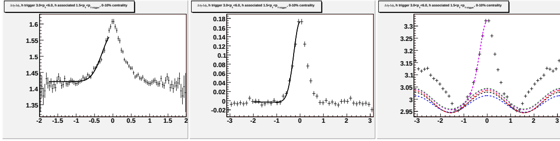
Figure L.4: Going left to right/top to bottom (a) jet-like correlation using \Delta\eta method (b) jet-like correlation using \Delta\phi method (c) correlation integrated over |\Delta\eta| < 0.75 (d) correlation integrated over 0.75 < |\Delta\eta| < 1.75 (e) correlation integrated over 0 < |\Delta\eta| < 1.75 (f) 1-D correlation for 3.0 < p_T^{trigger} < 6.0 GeV/c and 1.5 < p_T^{associated} < p_T^{trigger} GeV/c for 0-10% Cu + Cu collisions at \sqrt{s_{NN}} = 200 GeV.
