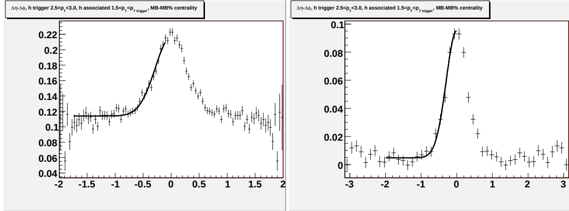
Figure I.16: Going left to right/top to bottom (a) jet-like correlation using \Delta\eta method (b) jet-like correlation using \Delta\phi method (c) correlation integrated over |\Delta\eta| < 0.75 (d) correlation integrated over 0.75 < |\Delta\eta| < 1.75 (e) correlation integrated over 0 < |\Delta\eta| < 1.75 (f) 1-D correlation for 2.5 < p_T^{trigger} < 3.0 GeV/c and 1.5 < p_T^{associated} < p_T^{trigger} GeV/c.
