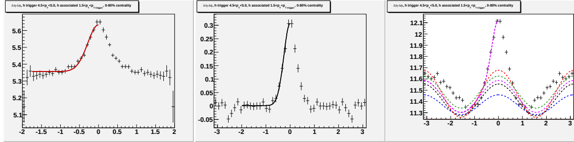
Figure I.13: Going left to right/top to bottom (a) jet-like correlation using \Delta\eta method (b) jet-like correlation using \Delta\phi method (c) correlation integrated over |\Delta\eta| < 0.75 (d) correlation integrated over 0.75 < |\Delta\eta| < 1.75 (e) correlation integrated over 0 < |\Delta\eta| < 1.75 (f) 1-D correlation for 4.5 < p_T^{trigger} < 5.0 GeV/c and 1.5 < p_T^{associated} < p_T^{trigger} GeV/c.
