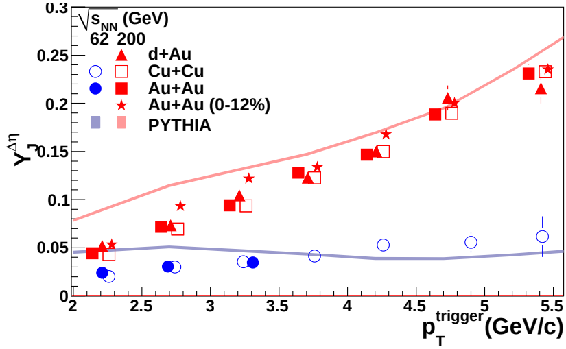
Figure F.1: p_T^{trigger} dependence of Y_{Jet} for unidentified hadrons for 1.5 \text{ GeV/c} < p_T^{associated} < p_T^{trigger} for 0-60% central Cu + Cu and 0-80% central Au + Au collisions at \sqrt{s_{NN}} = 62 \text{ GeV} and minimum bias d + Au , 0-60% central Cu + Cu and 40-80% central Au + Au collisions at \sqrt{s_{NN}} = 200 \text{ GeV} .
