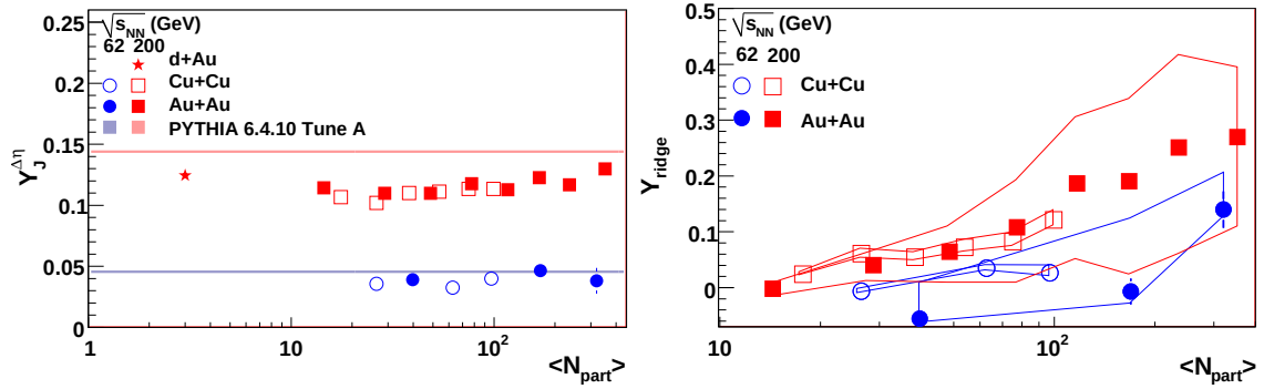
Figure J.1: N_{part} dependence of Y_{Jet} for unidentified hadrons for 3.0 < p_T^{trigger} < 6.0 GeV/c and 1.5 \text{ GeV/c} < p_T^{associated} < p_T^{trigger} for unidentified hadrons for Cu+Cu and Au+Au collisions at \sqrt{s_{NN}} = 62 GeV and d+Au , Cu+Cu and Au+Au collisions at \sqrt{s_{NN}} = 200 GeV.
