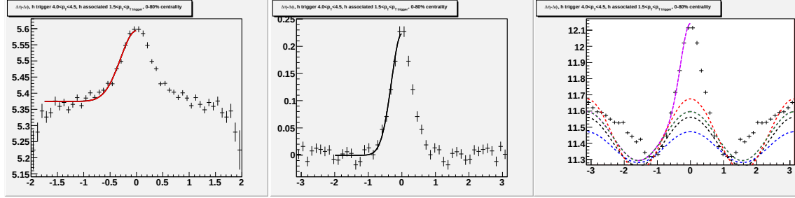
Figure I.12: Going left to right/top to bottom (a) jet-like correlation using \Delta\eta method (b) jet-like correlation using \Delta\phi method (c) correlation integrated over |\Delta\eta| < 0.75 (d) correlation integrated over 0.75 < |\Delta\eta| < 1.75 (e) correlation integrated over 0 < |\Delta\eta| < 1.75 (f) 1-D correlation for 4.0 < p_T^{trigger} < 4.5 GeV/c and 1.5 < p_T^{associated} < p_T^{trigger} GeV/c.
