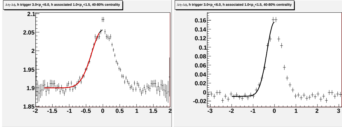
Figure P.1: Going left to right/top to bottom (a) jet-like correlation using \Delta\eta method (b) jet-like correlation using \Delta\phi method (c) correlation integrated over |\Delta\eta| < 0.75 (d) correlation integrated over 0.75 < |\Delta\eta| < 1.75 (e) correlation integrated over 0 < |\Delta\eta| < 1.75 (f) 1-D correlation for 3.0 < p_T^{trigger} < 6.0 \text{ GeV/c} and 1.0 < p_T^{associated} < 1.5 \text{ GeV/c} .
