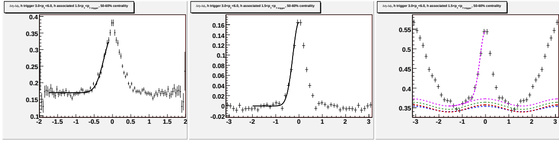
Figure L.9: Going left to right/top to bottom (a) jet-like correlation using \Delta\eta method (b) jet-like correlation using \Delta\phi method (c) correlation integrated over |\Delta\eta| < 0.75 (d) correlation integrated over 0.75 < |\Delta\eta| < 1.75 (e) correlation integrated over 0 < |\Delta\eta| < 1.75 (f) 1-D correlation for 3.0 < p_T^{trigger} < 6.0 GeV/c and 1.5 < p_T^{associated} < p_T^{trigger} GeV/c for 50-60% Cu + Cu collisions at \sqrt{s_{NN}} = 200 GeV.
