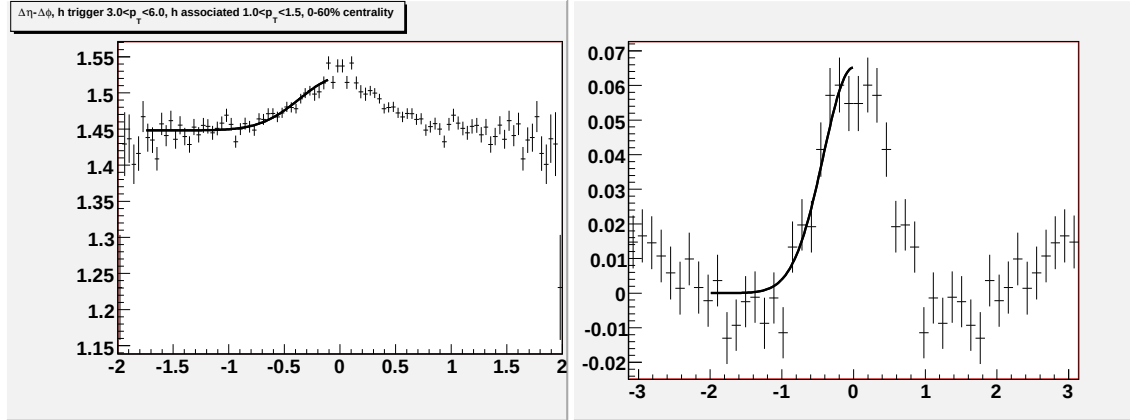
Figure N.1: Going left to right/top to bottom (a) jet-like correlation using \Delta\eta method (b) jet-like correlation using \Delta\phi method (c) correlation integrated over |\Delta\eta| < 0.75 (d) correlation integrated over 0.75 < |\Delta\eta| < 1.75 (e) correlation integrated over 0 < |\Delta\eta| < 1.75 (f) 1-D correlation for 3.0 < p_T^{trigger} < 6.0 GeV/c and 1.0 < p_T^{associated} < 1.5 GeV/c.
