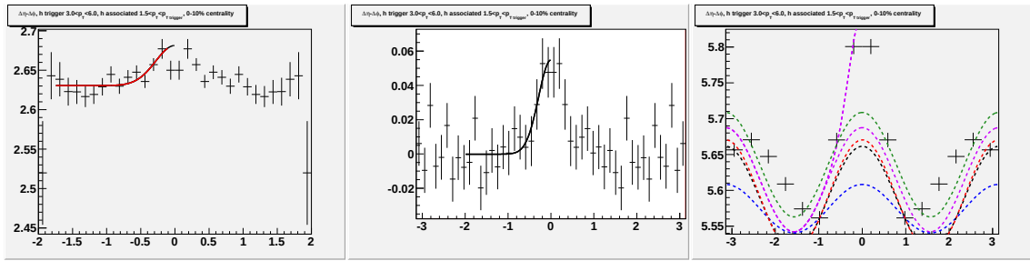
Figure L.1: Going left to right/top to bottom (a) jet-like correlation using \Delta\eta method (b) jet-like correlation using \Delta\phi method (c) correlation integrated over |\Delta\eta| < 0.75 (d) correlation integrated over 0.75 < |\Delta\eta| < 1.75 (e) correlation integrated over 0 < |\Delta\eta| < 1.75 (f) 1-D correlation for 3.0 < p_T^{trigger} < 6.0 GeV/c and 1.5 < p_T^{associated} < p_T^{trigger} GeV/c for 0-10% Au + Au collisions at \sqrt{s_{NN}} = 62 GeV.
