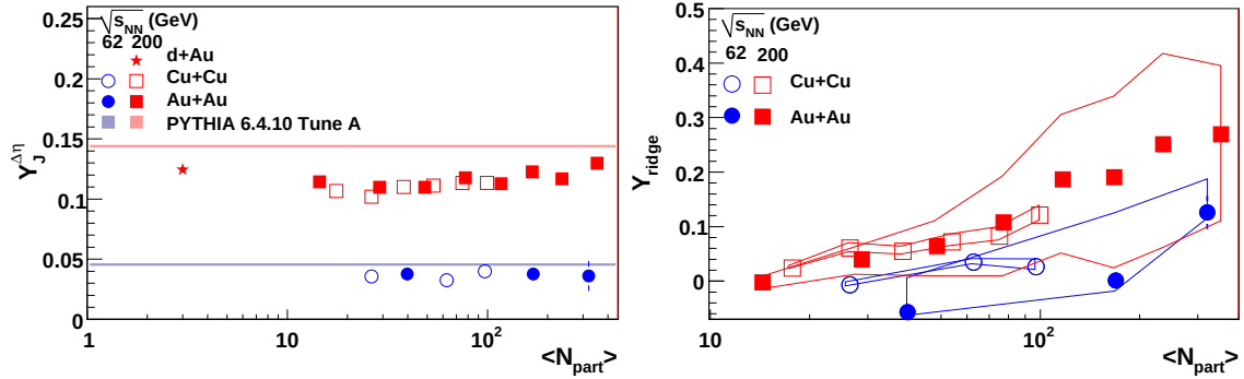
Figure G.1: N_{part} dependence of Y_{Jet} for unidentified hadrons for 3.0 < p_T^{trigger} < 6.0 GeV/c and 1.5 \text{ GeV/c} < p_T^{associated} < p_T^{trigger} for unidentified hadrons for Cu+Cu and Au+Au collisions at \sqrt{s_{NN}} = 62 GeV and d+Au , Cu+Cu and Au+Au collisions at \sqrt{s_{NN}} = 200 GeV.
