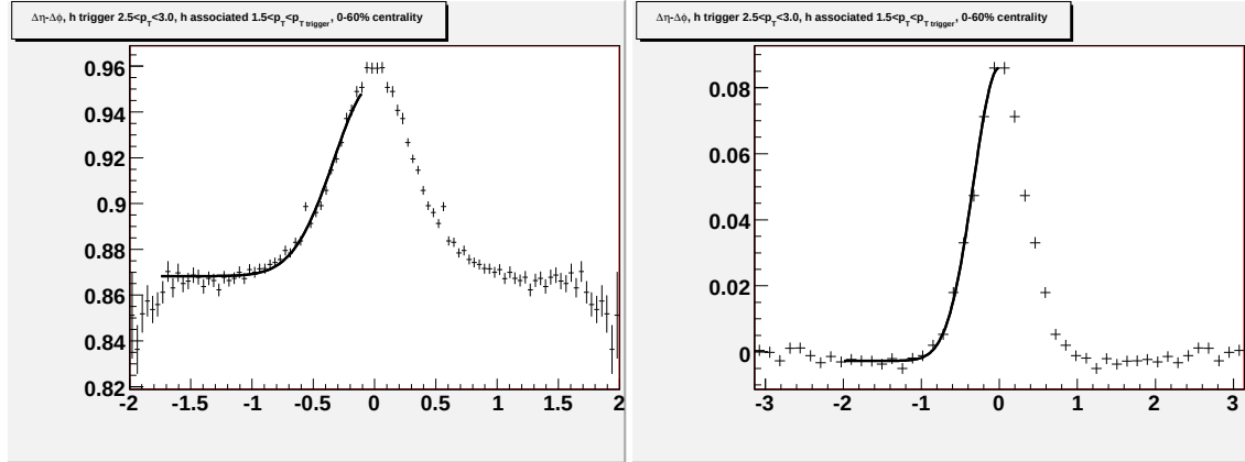
Figure F.14: Going left to right/top to bottom (a) jet-like correlation using \Delta\eta method (b) jet-like correlation using \Delta\phi method (c) correlation integrated over |\Delta\eta| < 0.75 (d) correlation integrated over 0.75 < |\Delta\eta| < 1.75 (e) correlation integrated over 0 < |\Delta\eta| < 1.75 (f) 1-D correlation for 2.5 < p_T^{trigger} < 3.0 GeV/c and 1.5 < p_T^{associated} < p_T^{trigger} GeV/c.
