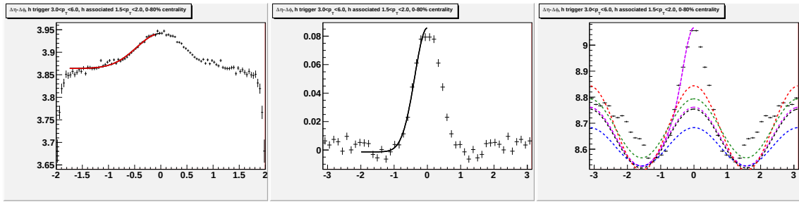
Figure H.21: Going left to right/top to bottom (a) jet-like correlation using \Delta\eta method (b) jet-like correlation using \Delta\phi method (c) correlation integrated over |\Delta\eta| < 0.75 (d) correlation integrated over 0.75 < |\Delta\eta| < 1.75 (e) correlation integrated over 0 < |\Delta\eta| < 1.75 (f) 1-D correlation for 3.0 < p_T^{trigger} < 6.0 GeV/c and 1.0 < p_T^{associated} < 1.5 GeV/c.
