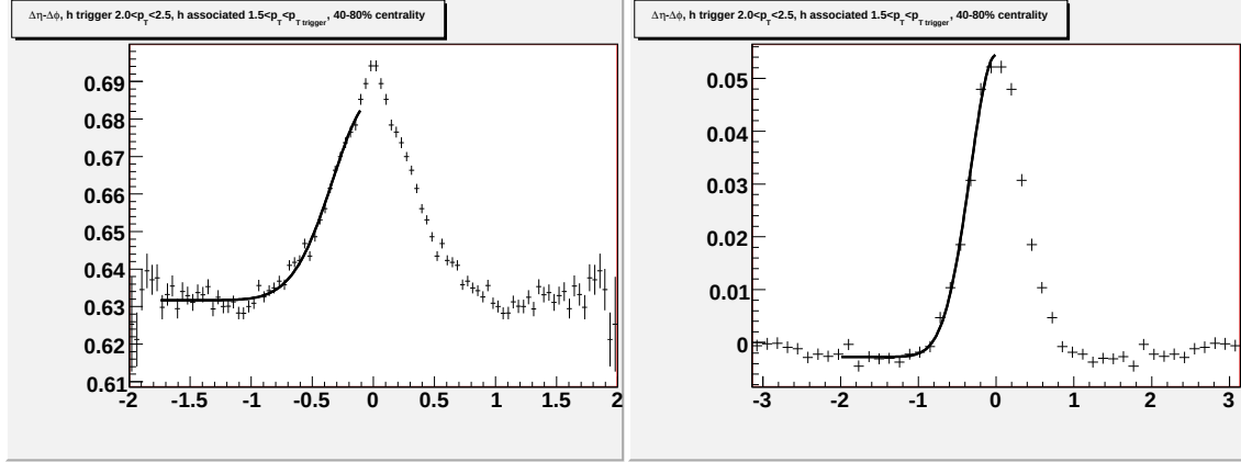
Figure F.20: Going left to right/top to bottom (a) jet-like correlation using \Delta\eta method (b) jet-like correlation using \Delta\phi method (c) correlation integrated over |\Delta\eta| < 0.75 (d) correlation integrated over 0.75 < |\Delta\eta| < 1.75 (e) correlation integrated over 0 < |\Delta\eta| < 1.75 (f) 1-D correlation for 2.0 < p_T^{trigger} < 2.5 GeV/c and 1.5 < p_T^{associated} < p_T^{trigger} GeV/c.
