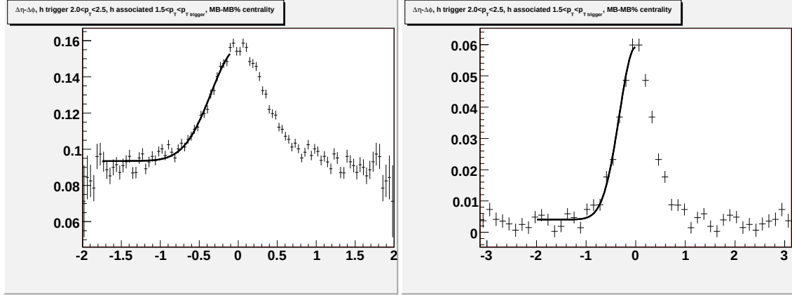
Figure F.34: Going left to right/top to bottom (a) jet-like correlation using \Delta\eta method (b) jet-like correlation using \Delta\phi method (c) correlation integrated over |\Delta\eta| < 0.75 (d) correlation integrated over 0.75 < |\Delta\eta| < 1.75 (e) correlation integrated over 0 < |\Delta\eta| < 1.75 (f) 1-D correlation for 2.0 < p_T^{trigger} < 2.5 GeV/c and 1.5 < p_T^{associated} < p_T^{trigger} GeV/c.
