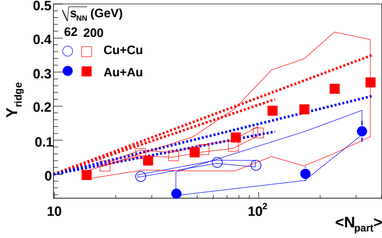
Figure 3.5: N_{part} dependence of Y_{Ridge} for unidentified hadrons for 3.0 < p_T^{trigger} < 6.0 GeV/c and 1.5 GeV/c < p_T^{associated} < p_T^{trigger} for Cu + Cu and Au + Au collisions at \sqrt{s_{NN}} = 62 GeV and Cu + Cu and Au + Au collisions at \sqrt{s_{NN}} = 200 GeV. Data from Au + Au collisions at \sqrt{s_{NN}} = 200 GeV are from [13, 14, 15, 16, 17, 18]. Lines indicate systematic errors due to v_2 .
