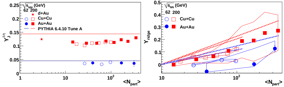
Figure H.1: N_{part} dependence of Y_{Jet} for unidentified hadrons for 3.0 < p_T^{trigger} < 6.0 GeV/c and 1.5 \text{ GeV/c} < p_T^{associated} < p_T^{trigger} for unidentified hadrons for Cu+Cu and Au+Au collisions at \sqrt{s_{NN}} = 62 GeV and d+Au , Cu+Cu and Au+Au collisions at \sqrt{s_{NN}} = 200 GeV.
