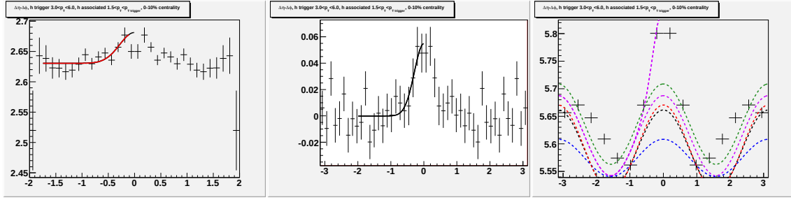
Figure H.5: Going left to right/top to bottom (a) jet-like correlation using \Delta\eta method (b) jet-like correlation using \Delta\phi method (c) correlation integrated over |\Delta\eta| < 0.75 (d) correlation integrated over 0.75 < |\Delta\eta| < 1.75 (e) correlation integrated over 0 < |\Delta\eta| < 1.75 (f) 1-D correlation for 3.0 < p_T^{trigger} < 6.0 GeV/c and 1.5 < p_T^{associated} < p_T^{trigger} GeV/c for 0-10% Au + Au collisions at \sqrt{s_{NN}} = 62 GeV.
