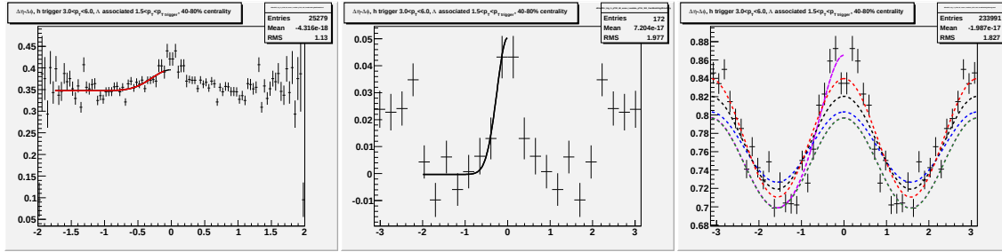
Figure K.9: Going left to right/top to bottom (a) jet-like correlation using \Delta\eta method (b) jet-like correlation using \Delta\phi method (c) correlation integrated over |\Delta\eta| < 0.75 (d) correlation integrated over 0.75 < |\Delta\eta| < 1.75 (e) correlation integrated over 0 < |\Delta\eta| < 1.75 (f) 1-D correlation for 4.0 < p_T^{trigger} < 6.0 GeV/c and 1.5 < p_T^{associated} < p_T^{trigger} GeV/c.
