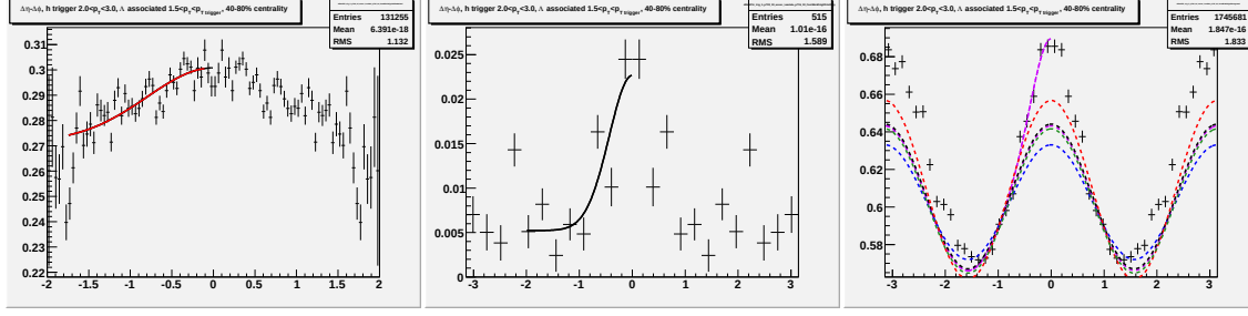
Figure K.8: Going left to right/top to bottom (a) jet-like correlation using \Delta\eta method (b) jet-like correlation using \Delta\phi method (c) correlation integrated over |\Delta\eta| < 0.75 (d) correlation integrated over 0.75 < |\Delta\eta| < 1.75 (e) correlation integrated over 0 < |\Delta\eta| < 1.75 (f) 1-D correlation for 2.0 < p_T^{trigger} < 3.0 GeV/c and 1.5 < p_T^{associated} < p_T^{trigger} GeV/c.
