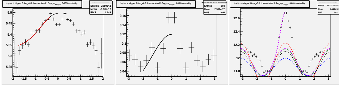
Figure F.10: Going left to right/top to bottom (a) jet-like correlation using \Delta\eta method (b) jet-like correlation using \Delta\phi method (c) correlation integrated over |\Delta\eta| < 0.75 (d) correlation integrated over 0.75 < |\Delta\eta| < 1.75 (e) correlation integrated over 0 < |\Delta\eta| < 1.75 (f) 1-D correlation for 3.0 < p_T^{trigger} < 6.0 GeV/c and 1.5 < p_T^{associated} < p_T^{trigger} GeV/c for \Lambda and \bar{\Lambda} trigger particles. 0-12% data
