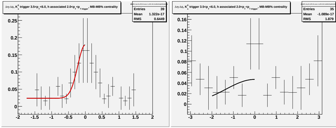
Figure I.3: Going left to right/top to bottom (a) jet-like correlation using \Delta\eta method (b) jet-like correlation using \Delta\phi method (c) correlation integrated over |\Delta\eta| < 0.75 (d) correlation integrated over 0.75 < |\Delta\eta| < 1.75 (e) correlation integrated over 0 < |\Delta\eta| < 1.75 (f) 1-D correlation for 3.5 < p_T^{trigger} < 6.0 GeV/c and 2.0 < p_T^{associated} < p_T^{trigger} GeV/c for K_S^0 triggers for minimum bias d + Au collisions at \sqrt{s_{NN}} = 200 GeV.
