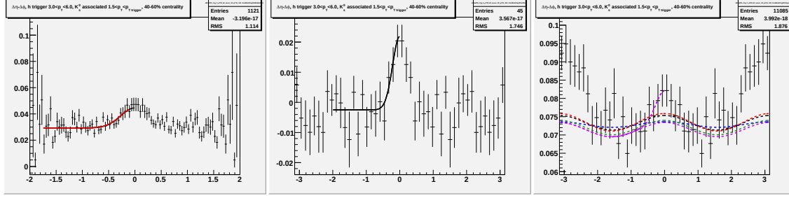
Figure L.4: Going left to right/top to bottom (a) jet-like correlation using \Delta\eta method (b) jet-like correlation using \Delta\phi method (c) correlation integrated over |\Delta\eta| < 0.75 (d) correlation integrated over 0.75 < |\Delta\eta| < 1.75 (e) correlation integrated over 0 < |\Delta\eta| < 1.75 (f) 1-D correlation for 3.0 < p_T^{trigger} < 6.0 GeV/c and 1.5 < p_T^{associated} < p_T^{trigger} GeV/c for 20-60% Cu + Cu collisions at \sqrt{s_{NN}} = 200 GeV for identified K_S^0 associated particles.
