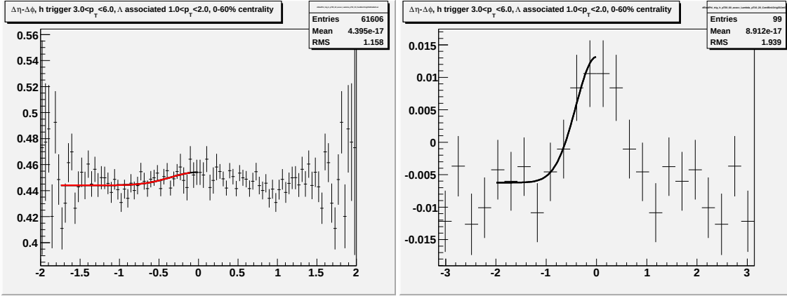
Figure M.4: Going left to right/top to bottom (a) jet-like correlation using \Delta\eta method (b) jet-like correlation using \Delta\phi method (c) correlation integrated over |\Delta\eta| < 0.75 (d) correlation integrated over 0.75 < |\Delta\eta| < 1.75 (e) correlation integrated over 0 < |\Delta\eta| < 1.75 (f) 1-D correlation for 3.0 < p_T^{trigger} < 6.0 GeV/c and 1.0 < p_T^{associated} < 2.0 GeV/c.
