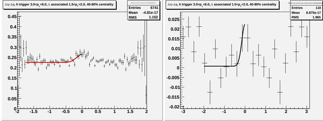
Figure M.14: Going left to right/top to bottom (a) jet-like correlation using \Delta\eta method (b) jet-like correlation using \Delta\phi method (c) correlation integrated over |\Delta\eta| < 0.75 (d) correlation integrated over 0.75 < |\Delta\eta| < 1.75 (e) correlation integrated over 0 < |\Delta\eta| < 1.75 (f) 1-D correlation for 3.0 < p_T^{trigger} < 6.0 GeV/c and 1.5 < p_T^{associated} < 2.0 GeV/c.
