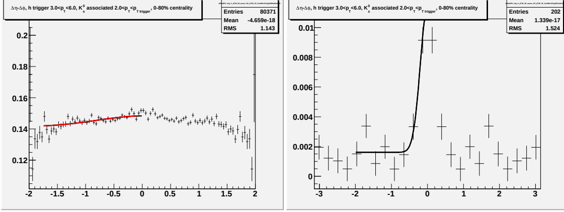
Figure M.7: Going left to right/top to bottom (a) jet-like correlation using \Delta\eta method (b) jet-like correlation using \Delta\phi method (c) correlation integrated over |\Delta\eta| < 0.75 (d) correlation integrated over 0.75 < |\Delta\eta| < 1.75 (e) correlation integrated over 0 < |\Delta\eta| < 1.75 (f) 1-D correlation for 3.0 < p_T^{trigger} < 6.0 GeV/c and 2.0 < p_T^{associated} < 3.0 GeV/c.
