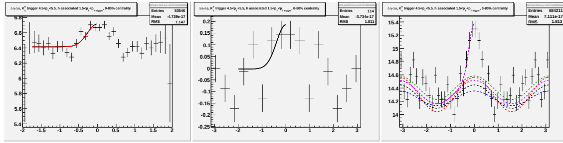
Figure E.19: Going left to right/top to bottom (a) jet-like correlation using \Delta\eta method (b) jet-like correlation using \Delta\phi method (c) correlation integrated over |\Delta\eta| < 0.75 (d) correlation integrated over 0.75 < |\Delta\eta| < 1.75 (e) correlation integrated over 0 < |\Delta\eta| < 1.75 (f) 1-D correlation for 4.5 < p_T^{trigger} < 5.5 GeV/c and 1.5 < p_T^{associated} < p_T^{trigger} GeV/c for K_S^0 trigger particles.
