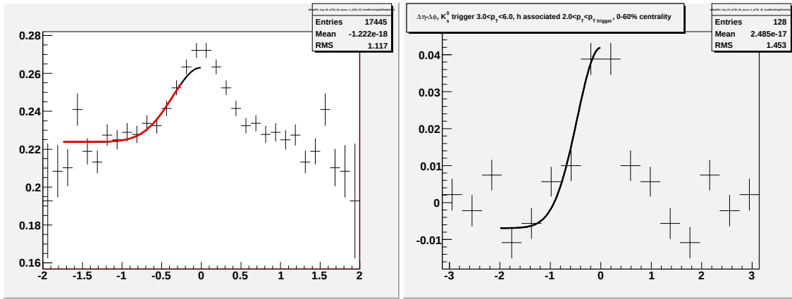
Figure J.10: Going left to right/top to bottom (a) jet-like correlation using \Delta\eta method (b) jet-like correlation using \Delta\phi method (c) correlation integrated over |\Delta\eta| < 0.75 (d) correlation integrated over 0.75 < |\Delta\eta| < 1.75 (e) correlation integrated over 0 < |\Delta\eta| < 1.75 (f) 1-D correlation for 3.0 < p_T^{\text{trigger}} < 6.0 GeV/c and 2.0 < p_T^{\text{associated}} < 3.0 GeV/c for K_S^0 trigger particles.
