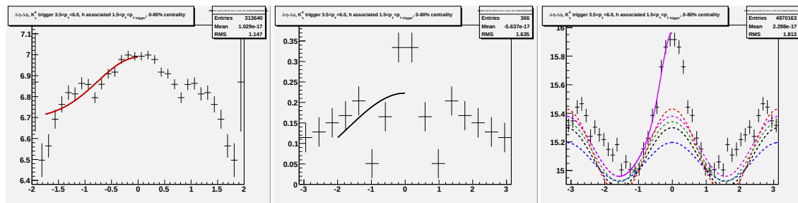
Figure H.13: Going left to right/top to bottom (a) jet-like correlation using \Delta\eta method (b) jet-like correlation using \Delta\phi method (c) correlation integrated over |\Delta\eta| < 0.75 (d) correlation integrated over 0.75 < |\Delta\eta| < 1.75 (e) correlation integrated over 0 < |\Delta\eta| < 1.75 (f) 1-D correlation for 3.5 < p_T^{trigger} < 6.0 GeV/c and 1.5 < p_T^{associated} < p_T^{trigger} GeV/c for K_S^0 trigger particles. 0-12% data
