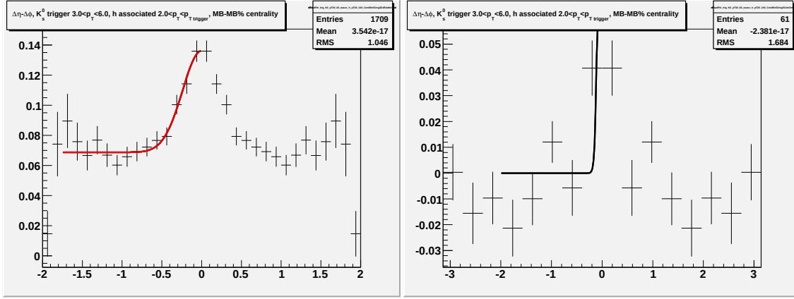
Figure G.8: Going left to right/top to bottom (a) jet-like correlation using \Delta\eta method (b) jet-like correlation using \Delta\phi method (c) correlation integrated over |\Delta\eta| < 0.75 (d) correlation integrated over 0.75 < |\Delta\eta| < 1.75 (e) correlation integrated over 0 < |\Delta\eta| < 1.75 (f) 1-D correlation for 3.0 < p_T^{trigger} < 6.0 GeV/c and 2.0 < p_T^{associated} < p_T^{trigger} GeV/c for K_S^0 trigger particles.
