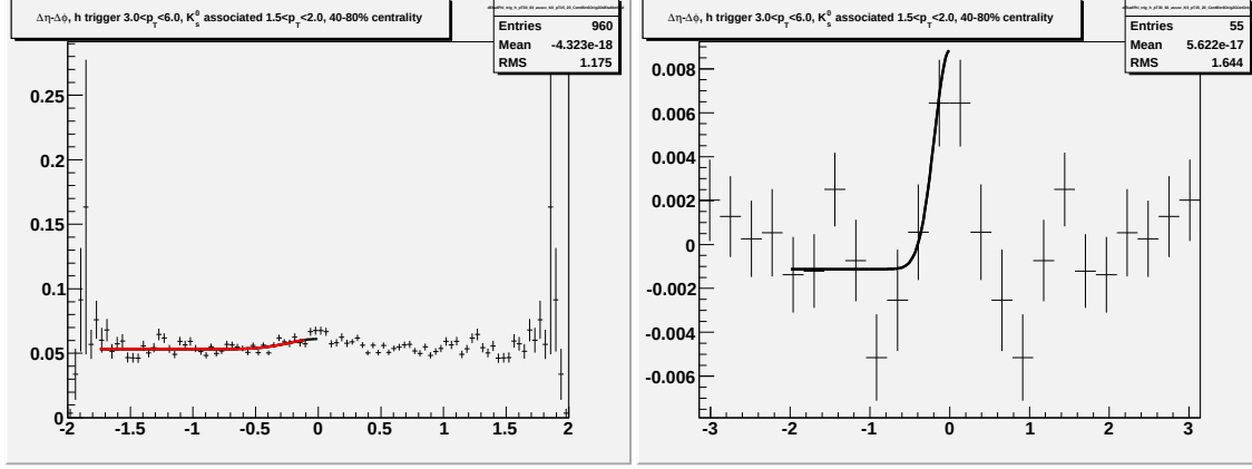
Figure M.11: Going left to right/top to bottom (a) jet-like correlation using \Delta\eta method (b) jet-like correlation using \Delta\phi method (c) correlation integrated over |\Delta\eta| < 0.75 (d) correlation integrated over 0.75 < |\Delta\eta| < 1.75 (e) correlation integrated over 0 < |\Delta\eta| < 1.75 (f) 1-D correlation for 3.0 < p_T^{trigger} < 6.0 GeV/c and 1.5 < p_T^{associated} < 2.0 GeV/c.
