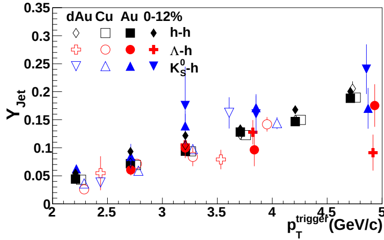
Figure E.1: p_T^{trigger} dependence of Y_{Jet} for 1.5 GeV/c < p_T^{associated} < p_T^{trigger} in 0-60% central Cu + Cu and 0-12% central Au + Au collisions at \sqrt{s_{NN}} = 200 GeV for unidentified hadrons, \Lambda , K_S^0 , and \Xi trigger particles. The identified trigger particle data have been horizontally offset for visibility.
