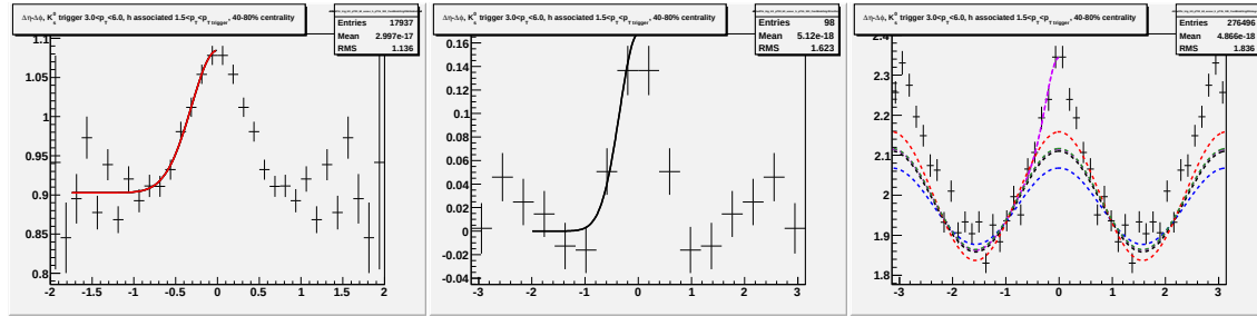
Figure F.17: Going left to right/top to bottom (a) jet-like correlation using \Delta\eta method (b) jet-like correlation using \Delta\phi method (c) correlation integrated over |\Delta\eta| < 0.75 (d) correlation integrated over 0.75 < |\Delta\eta| < 1.75 (e) correlation integrated over 0 < |\Delta\eta| < 1.75 (f) 1-D correlation for 3.0 < p_T^{trigger} < 6.0 GeV/c and 1.5 < p_T^{associated} < p_T^{trigger} GeV/c for K_S^0 trigger particles.
