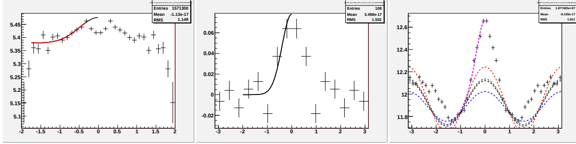
Figure E.14: Going left to right/top to bottom (a) jet-like correlation using \Delta\eta method (b) jet-like correlation using \Delta\phi method (c) correlation integrated over |\Delta\eta| < 0.75 (d) correlation integrated over 0.75 < |\Delta\eta| < 1.75 (e) correlation integrated over 0 < |\Delta\eta| < 1.75 (f) 1-D correlation for 3.0 < p_T^{trigger} < 3.5 GeV/c and 1.5 < p_T^{associated} < p_T^{trigger} GeV/c for \Lambda and \bar{\Lambda} trigger particles.
