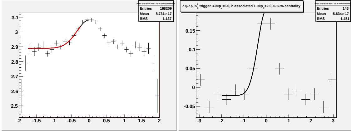
Figure J.9: Going left to right/top to bottom (a) jet-like correlation using \Delta\eta method (b) jet-like correlation using \Delta\phi method (c) correlation integrated over |\Delta\eta| < 0.75 (d) correlation integrated over 0.75 < |\Delta\eta| < 1.75 (e) correlation integrated over 0 < |\Delta\eta| < 1.75 (f) 1-D correlation for 3.0 < p_T^{trigger} < 6.0 GeV/c and 1.0 < p_T^{associated} < 2.0 GeV/c for K_S^0 trigger particles.
