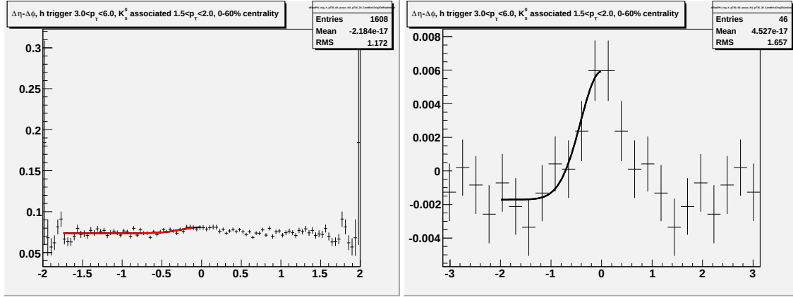
Figure M.2: Going left to right/top to bottom (a) jet-like correlation using \Delta\eta method (b) jet-like correlation using \Delta\phi method (c) correlation integrated over |\Delta\eta| < 0.75 (d) correlation integrated over 0.75 < |\Delta\eta| < 1.75 (e) correlation integrated over 0 < |\Delta\eta| < 1.75 (f) 1-D correlation for 3.0 < p_T^{trigger} < 6.0 GeV/c and 1.5 < p_T^{associated} < 2.0 GeV/c.
