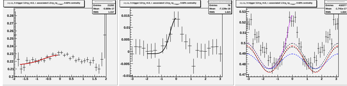
Figure K.4: Going left to right/top to bottom (a) jet-like correlation using \Delta\eta method (b) jet-like correlation using \Delta\phi method (c) correlation integrated over |\Delta\eta| < 0.75 (d) correlation integrated over 0.75 < |\Delta\eta| < 1.75 (e) correlation integrated over 0 < |\Delta\eta| < 1.75 (f) 1-D correlation for 3.0 < p_T^{trigger} < 4.0 GeV/c and 1.5 < p_T^{associated} < p_T^{trigger} GeV/c.
