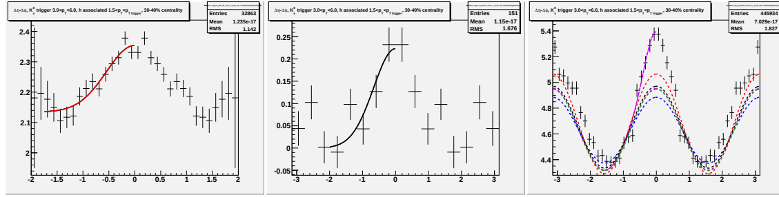
Figure F.16: Going left to right/top to bottom (a) jet-like correlation using \Delta\eta method (b) jet-like correlation using \Delta\phi method (c) correlation integrated over |\Delta\eta| < 0.75 (d) correlation integrated over 0.75 < |\Delta\eta| < 1.75 (e) correlation integrated over 0 < |\Delta\eta| < 1.75 (f) 1-D correlation for 3.0 < p_T^{trigger} < 6.0 GeV/c and 1.5 < p_T^{associated} < p_T^{trigger} GeV/c for K_S^0 trigger particles.
