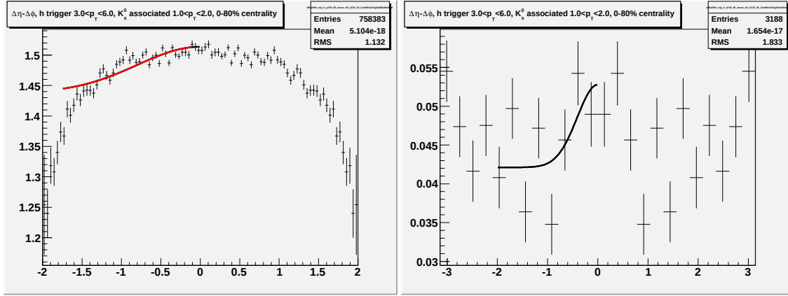
Figure M.6: Going left to right/top to bottom (a) jet-like correlation using \Delta\eta method (b) jet-like correlation using \Delta\phi method (c) correlation integrated over |\Delta\eta| < 0.75 (d) correlation integrated over 0.75 < |\Delta\eta| < 1.75 (e) correlation integrated over 0 < |\Delta\eta| < 1.75 (f) 1-D correlation for 3.0 < p_T^{trigger} < 6.0 GeV/c and 1.0 < p_T^{associated} < 20 GeV/c.
