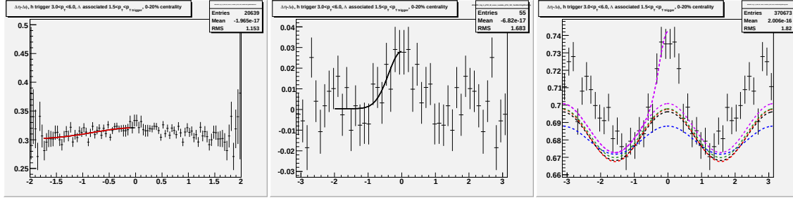
Figure L.5: Going left to right/top to bottom (a) jet-like correlation using \Delta\eta method (b) jet-like correlation using \Delta\phi method (c) correlation integrated over |\Delta\eta| < 0.75 (d) correlation integrated over 0.75 < |\Delta\eta| < 1.75 (e) correlation integrated over 0 < |\Delta\eta| < 1.75 (f) 1-D correlation for 3.0 < p_T^{trigger} < 6.0 GeV/c and 1.5 < p_T^{associated} < p_T^{trigger} GeV/c for 0-30% Cu + Cu collisions at \sqrt{s_{NN}} = 200 GeV for identified \Lambda associated particles.
