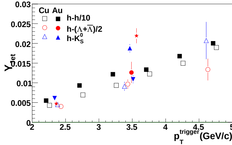
Figure K.1: p_T^{trigger} dependence of Y_{Jet} for 1.5 \text{ GeV/c} < p_T^{associated} < p_T^{trigger} in 0-60% central Cu + Cu and 0-12% central Au + Au collisions at \sqrt{s_{NN}} = 200 \text{ GeV} for unidentified hadrons, \Lambda and K_S^0 associated particles. The identified associated particle data have been horizontally offset for visibility.
