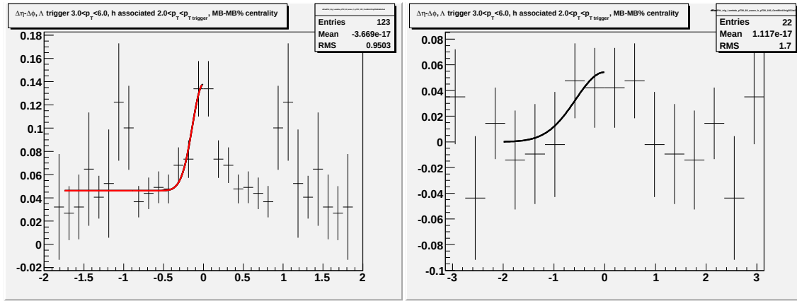
Figure G.2: Going left to right/top to bottom (a) jet-like correlation using \Delta\eta method (b) jet-like correlation using \Delta\phi method (c) correlation integrated over |\Delta\eta| < 0.75 (d) correlation integrated over 0.75 < |\Delta\eta| < 1.75 (e) correlation integrated over 0 < |\Delta\eta| < 1.75 (f) 1-D correlation for 3.0 < p_T^{trigger} < 6.0 GeV/c and 2.0 < p_T^{associated} < p_T^{trigger} GeV/c for \Lambda + \bar{\Lambda} triggers for minimum bias d + Au collisions at \sqrt{s_{NN}} = 200 GeV.
