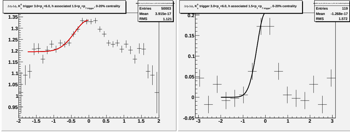
Figure F.6: Going left to right/top to bottom (a) jet-like correlation using \Delta\eta method (b) jet-like correlation using \Delta\phi method (c) correlation integrated over |\Delta\eta| < 0.75 (d) correlation integrated over 0.75 < |\Delta\eta| < 1.75 (e) correlation integrated over 0 < |\Delta\eta| < 1.75 (f) 1-D correlation for 3.0 < p_T^{trigger} < 6.0 GeV/c and 1.5 < p_T^{associated} < p_T^{trigger} GeV/c for K_S^0 trigger particles.
