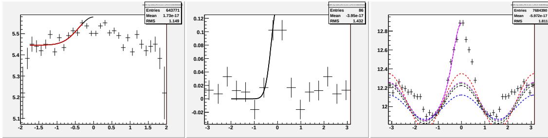
Figure E.15: Going left to right/top to bottom (a) jet-like correlation using \Delta\eta method (b) jet-like correlation using \Delta\phi method (c) correlation integrated over |\Delta\eta| < 0.75 (d) correlation integrated over 0.75 < |\Delta\eta| < 1.75 (e) correlation integrated over 0 < |\Delta\eta| < 1.75 (f) 1-D correlation for 3.5 < p_T^{trigger} < 4.5 GeV/c and 1.5 < p_T^{associated} < p_T^{trigger} GeV/c for \Lambda and \bar{\Lambda} trigger particles.
