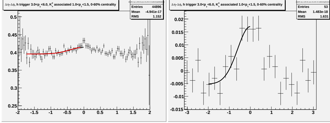
Figure M.1: Going left to right/top to bottom (a) jet-like correlation using \Delta\eta method (b) jet-like correlation using \Delta\phi method (c) correlation integrated over |\Delta\eta| < 0.75 (d) correlation integrated over 0.75 < |\Delta\eta| < 1.75 (e) correlation integrated over 0 < |\Delta\eta| < 1.75 (f) 1-D correlation for 3.0 < p_T^{trigger} < 6.0 GeV/c and 1.0 < p_T^{associated} < 1.5 GeV/c.
