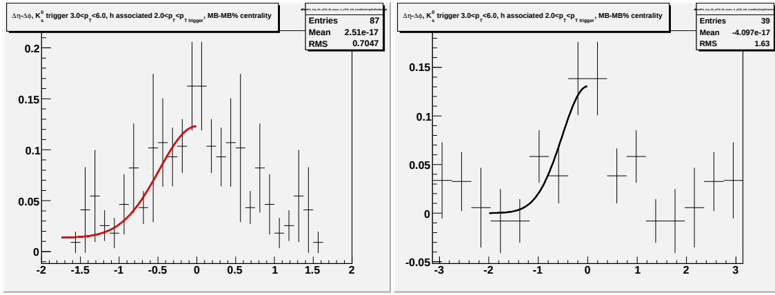
Figure G.3: Going left to right/top to bottom (a) jet-like correlation using \Delta\eta method (b) jet-like correlation using \Delta\phi method (c) correlation integrated over |\Delta\eta| < 0.75 (d) correlation integrated over 0.75 < |\Delta\eta| < 1.75 (e) correlation integrated over 0 < |\Delta\eta| < 1.75 (f) 1-D correlation for 3.0 < p_T^{trigger} < 6.0 GeV/c and 2.0 < p_T^{associated} < p_T^{trigger} GeV/c for K_S^0 triggers for minimum bias d + Au collisions at \sqrt{s_{NN}} = 200 GeV.
