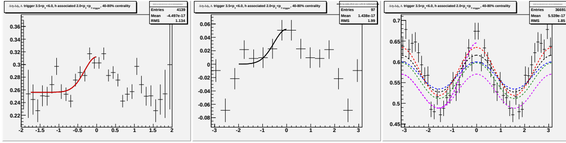
Figure I.12: Going left to right/top to bottom (a) jet-like correlation using \Delta\eta method (b) jet-like correlation using \Delta\phi method (c) correlation integrated over |\Delta\eta| < 0.75 (d) correlation integrated over 0.75 < |\Delta\eta| < 1.75 (e) correlation integrated over 0 < |\Delta\eta| < 1.75 (f) 1-D correlation for 3.5 < p_T^{trigger} < 6.0 GeV/c and 2.0 < p_T^{associated} < p_T^{trigger} GeV/c for \Lambda and \bar{\Lambda} trigger particles.
