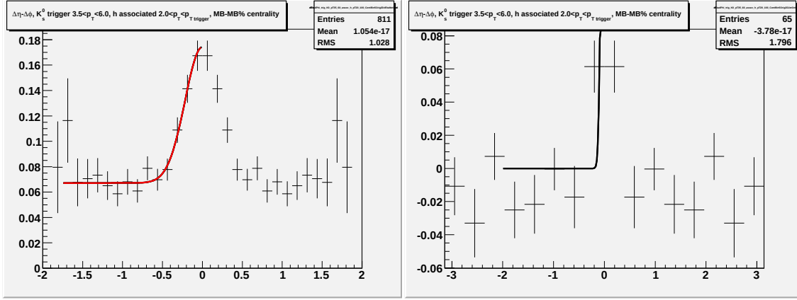
Figure I.8: Going left to right/top to bottom (a) jet-like correlation using \Delta\eta method (b) jet-like correlation using \Delta\phi method (c) correlation integrated over |\Delta\eta| < 0.75 (d) correlation integrated over 0.75 < |\Delta\eta| < 1.75 (e) correlation integrated over 0 < |\Delta\eta| < 1.75 (f) 1-D correlation for 3.5 < p_T^{trigger} < 6.0 GeV/c and 2.0 < p_T^{associated} < p_T^{trigger} GeV/c for K_S^0 trigger particles.
