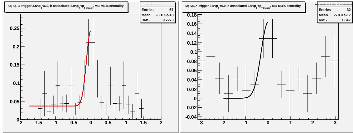
Figure I.2: Going left to right/top to bottom (a) jet-like correlation using \Delta\eta method (b) jet-like correlation using \Delta\phi method (c) correlation integrated over |\Delta\eta| < 0.75 (d) correlation integrated over 0.75 < |\Delta\eta| < 1.75 (e) correlation integrated over 0 < |\Delta\eta| < 1.75 (f) 1-D correlation for 3.5 < p_T^{trigger} < 6.0 GeV/c and 2.0 < p_T^{associated} < p_T^{trigger} GeV/c for \Lambda + \bar{\Lambda} triggers for minimum bias d + Au collisions at \sqrt{s_{NN}} = 200 GeV.
