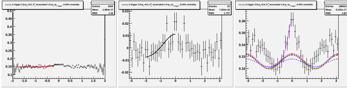
Figure L.2: Going left to right/top to bottom (a) jet-like correlation using \Delta\eta method (b) jet-like correlation using \Delta\phi method (c) correlation integrated over |\Delta\eta| < 0.75 (d) correlation integrated over 0.75 < |\Delta\eta| < 1.75 (e) correlation integrated over 0 < |\Delta\eta| < 1.75 (f) 1-D correlation for 3.0 < p_T^{trigger} < 6.0 GeV/c and 1.5 < p_T^{associated} < p_T^{trigger} GeV/c for 0-20% Cu + Cu collisions at \sqrt{s_{NN}} = 200 GeV for identified K_S^0 associated particles.
