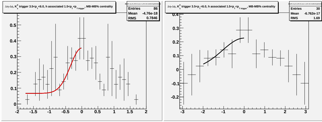
Figure H.3: Going left to right/top to bottom (a) jet-like correlation using \Delta\eta method (b) jet-like correlation using \Delta\phi method (c) correlation integrated over |\Delta\eta| < 0.75 (d) correlation integrated over 0.75 < |\Delta\eta| < 1.75 (e) correlation integrated over 0 < |\Delta\eta| < 1.75 (f) 1-D correlation for 3.5 < p_T^{trigger} < 6.0 GeV/c and 1.5 < p_T^{associated} < p_T^{trigger} GeV/c for K_S^0 triggers for minimum bias d + Au collisions at \sqrt{s_{NN}} = 200 GeV.
