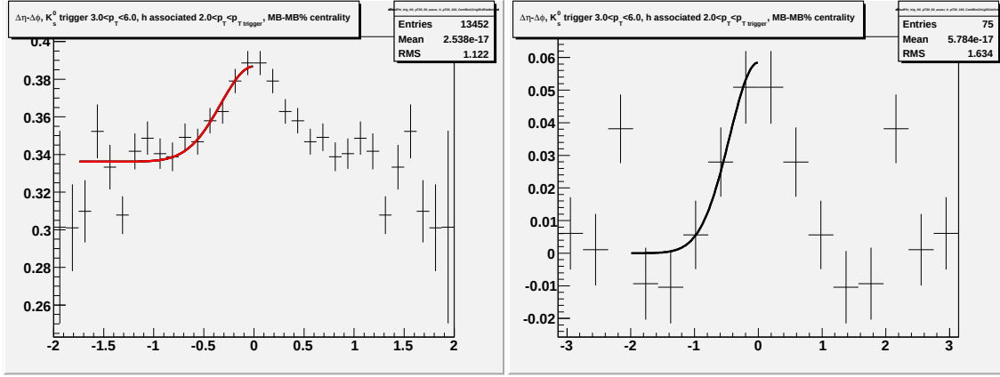
Figure G.6: Going left to right/top to bottom (a) jet-like correlation using \Delta\eta method (b) jet-like correlation using \Delta\phi method (c) correlation integrated over |\Delta\eta| < 0.75 (d) correlation integrated over 0.75 < |\Delta\eta| < 1.75 (e) correlation integrated over 0 < |\Delta\eta| < 1.75 (f) 1-D correlation for 3.0 < p_T^{trigger} < 6.0 GeV/c and 2.0 < p_T^{associated} < p_T^{trigger} GeV/c for K_S^0 trigger particles.
