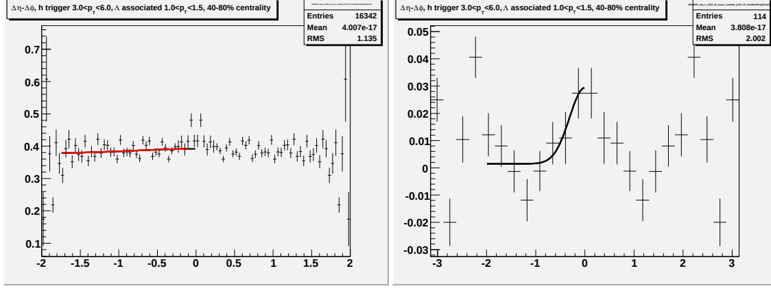
Figure M.13: Going left to right/top to bottom (a) jet-like correlation using \Delta\eta method (b) jet-like correlation using \Delta\phi method (c) correlation integrated over |\Delta\eta| < 0.75 (d) correlation integrated over 0.75 < |\Delta\eta| < 1.75 (e) correlation integrated over 0 < |\Delta\eta| < 1.75 (f) 1-D correlation for 3.0 < p_T^{trigger} < 6.0 GeV/c and 1.0 < p_T^{associated} < 1.5 GeV/c.
