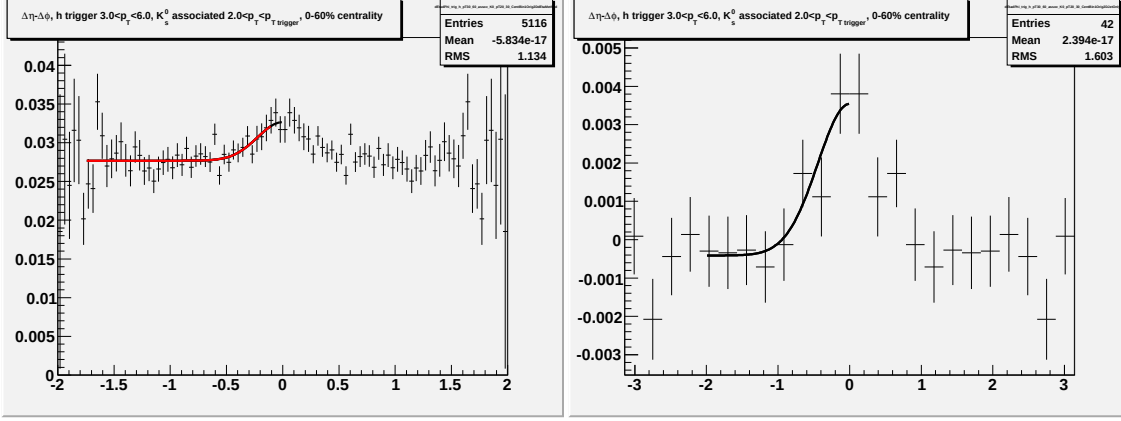
Figure M.3: Going left to right/top to bottom (a) jet-like correlation using \Delta\eta method (b) jet-like correlation using \Delta\phi method (c) correlation integrated over |\Delta\eta| < 0.75 (d) correlation integrated over 0.75 < |\Delta\eta| < 1.75 (e) correlation integrated over 0 < |\Delta\eta| < 1.75 (f) 1-D correlation for 3.0 < p_T^{trigger} < 6.0 GeV/c and 2.0 < p_T^{associated} < 3.0 GeV/c.
