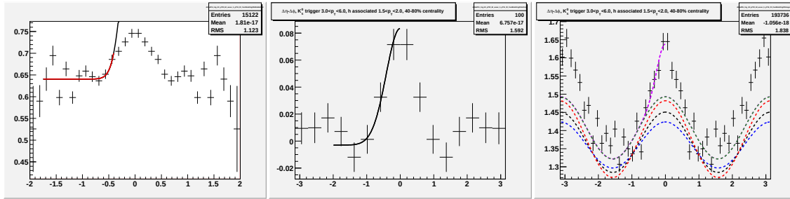
Figure J.15: Going left to right/top to bottom (a) jet-like correlation using \Delta\eta method (b) jet-like correlation using \Delta\phi method (c) correlation integrated over |\Delta\eta| < 0.75 (d) correlation integrated over 0.75 < |\Delta\eta| < 1.75 (e) correlation integrated over 0 < |\Delta\eta| < 1.75 (f) 1-D correlation for 3.0 < p_T^{trigger} < 6.0 GeV/c and 1.5 < p_T^{associated} < 2.0 GeV/c for K_S^0 trigger particles.
