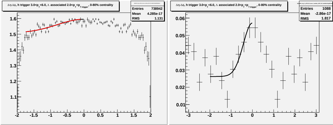
Figure M.9: Going left to right/top to bottom (a) jet-like correlation using \Delta\eta method (b) jet-like correlation using \Delta\phi method (c) correlation integrated over |\Delta\eta| < 0.75 (d) correlation integrated over 0.75 < |\Delta\eta| < 1.75 (e) correlation integrated over 0 < |\Delta\eta| < 1.75 (f) 1-D correlation for 3.0 < p_T^{trigger} < 6.0 GeV/c and 2.0 < p_T^{associated} < 3.0 GeV/c.
