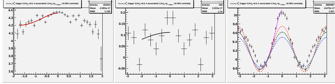
Figure F.15: Going left to right/top to bottom (a) jet-like correlation using \Delta\eta method (b) jet-like correlation using \Delta\phi method (c) correlation integrated over |\Delta\eta| < 0.75 (d) correlation integrated over 0.75 < |\Delta\eta| < 1.75 (e) correlation integrated over 0 < |\Delta\eta| < 1.75 (f) 1-D correlation for 3.0 < p_T^{trigger} < 6.0 GeV/c and 1.5 < p_T^{associated} < p_T^{trigger} GeV/c for K_S^0 trigger particles.
