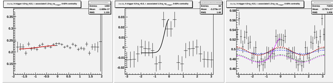
Figure K.5: Going left to right/top to bottom (a) jet-like correlation using \Delta\eta method (b) jet-like correlation using \Delta\phi method (c) correlation integrated over |\Delta\eta| < 0.75 (d) correlation integrated over 0.75 < |\Delta\eta| < 1.75 (e) correlation integrated over 0 < |\Delta\eta| < 1.75 (f) 1-D correlation for 4.0 < p_T^{trigger} < 6.0 GeV/c and 1.5 < p_T^{associated} < p_T^{trigger} GeV/c.
