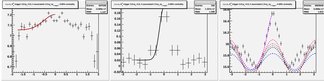
Figure E.17: Going left to right/top to bottom (a) jet-like correlation using \Delta\eta method (b) jet-like correlation using \Delta\phi method (c) correlation integrated over |\Delta\eta| < 0.75 (d) correlation integrated over 0.75 < |\Delta\eta| < 1.75 (e) correlation integrated over 0 < |\Delta\eta| < 1.75 (f) 1-D correlation for 3.0 < p_T^{trigger} < 3.5 GeV/c and 1.5 < p_T^{associated} < p_T^{trigger} GeV/c for K_S^0 trigger particles.
