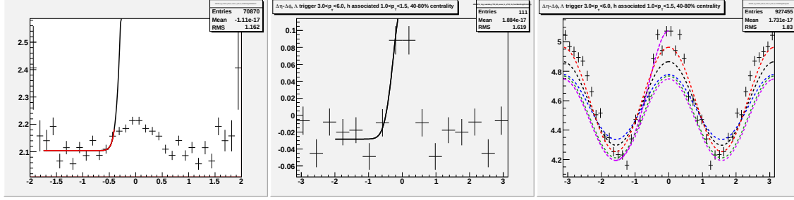
Going left to right/top to bottom (a) jet-like correlation using \Delta\eta method (b) jet-like correlation using \Delta\phi method (c) correlation integrated over |\Delta\eta| < 0.75 (d) correlation integrated over 0.75 < |\Delta\eta| < 1.75 (e) correlation integrated over 0 < |\Delta\eta| < 1.75 (f) 1-D correlation for 3.0 < p_T^{trigger} < 6.0 GeV/c and 1.0 < p_T^{associated} < 1.5 GeV/c for \Lambda and \bar{\Lambda} trigger particles.
