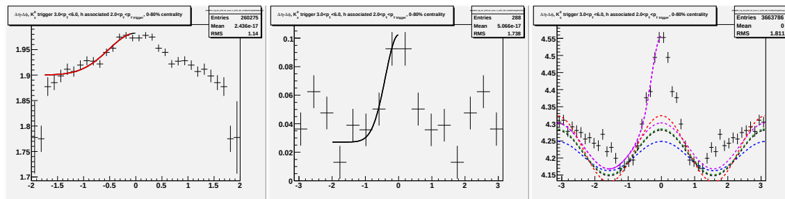
Figure G.13: Going left to right/top to bottom (a) jet-like correlation using \Delta\eta method (b) jet-like correlation using \Delta\phi method (c) correlation integrated over |\Delta\eta| < 0.75 (d) correlation integrated over 0.75 < |\Delta\eta| < 1.75 (e) correlation integrated over 0 < |\Delta\eta| < 1.75 (f) 1-D correlation for 3.0 < p_T^{trigger} < 6.0 GeV/c and 2.0 < p_T^{associated} < p_T^{trigger} GeV/c for K_S^0 trigger particles. 0-12% data
