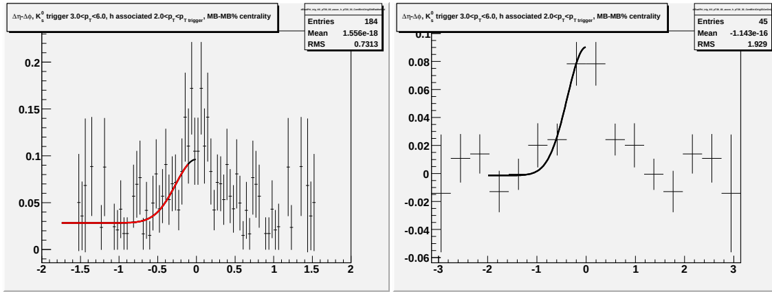
Figure J.7: Going left to right/top to bottom (a) jet-like correlation using \Delta\eta method (b) jet-like correlation using \Delta\phi method (c) correlation integrated over |\Delta\eta| < 0.75 (d) correlation integrated over 0.75 < |\Delta\eta| < 1.75 (e) correlation integrated over 0 < |\Delta\eta| < 1.75 (f) 1-D correlation for 3.0 < p_T^{\text{trigger}} < 6.0 GeV/c and 2.0 < p_T^{\text{associated}} < 3.0 GeV/c for identified K_S^0 triggers.
