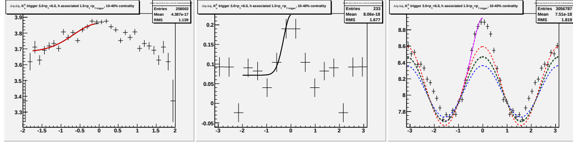
Figure F.14: Going left to right/top to bottom (a) jet-like correlation using \Delta\eta method (b) jet-like correlation using \Delta\phi method (c) correlation integrated over |\Delta\eta| < 0.75 (d) correlation integrated over 0.75 < |\Delta\eta| < 1.75 (e) correlation integrated over 0 < |\Delta\eta| < 1.75 (f) 1-D correlation for 3.0 < p_T^{trigger} < 6.0 GeV/c and 1.5 < p_T^{associated} < p_T^{trigger} GeV/c for K_S^0 trigger particles.
