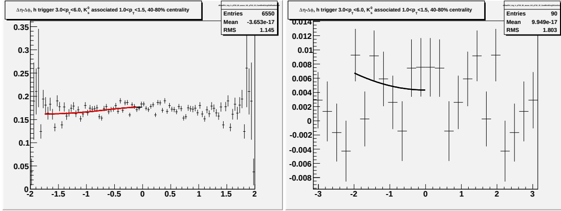
Figure P.10: Going left to right/top to bottom (a) jet-like correlation using \Delta\eta method (b) jet-like correlation using \Delta\phi method (c) correlation integrated over |\Delta\eta| < 0.75 (d) correlation integrated over 0.75 < |\Delta\eta| < 1.75 (e) correlation integrated over 0 < |\Delta\eta| < 1.75 (f) 1-D correlation for 3.0 < p_T^{trigger} < 6.0 GeV/c and 1.0 < p_T^{associated} < 1.5 GeV/c.
