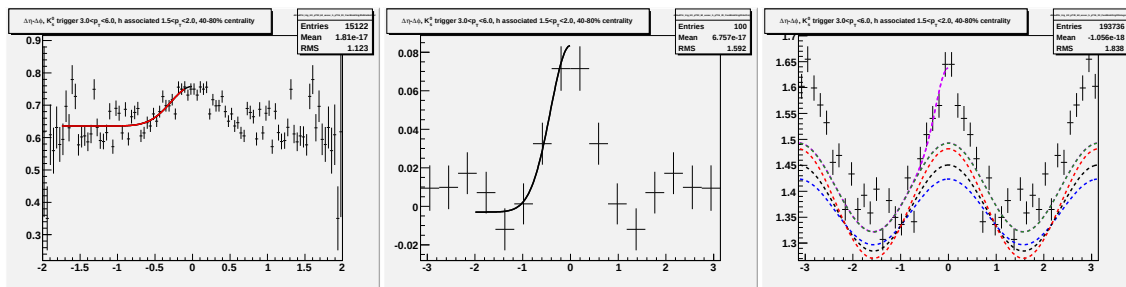
Figure J.15: Going left to right/top to bottom (a) jet-like correlation using \Delta\eta method (b) jet-like correlation using \Delta\phi method (c) correlation integrated over |\Delta\eta| < 0.75 (d) correlation integrated over 0.75 < |\Delta\eta| < 1.75 (e) correlation integrated over 0 < |\Delta\eta| < 1.75 (f) 1-D correlation for 3.0 < p_T^{trigger} < 6.0 GeV/c and 1.5 < p_T^{associated} < 2.0 GeV/c for K_S^0 trigger particles.
