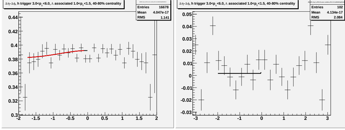
Figure P.13: Going left to right/top to bottom (a) jet-like correlation using \Delta\eta method (b) jet-like correlation using \Delta\phi method (c) correlation integrated over |\Delta\eta| < 0.75 (d) correlation integrated over 0.75 < |\Delta\eta| < 1.75 (e) correlation integrated over 0 < |\Delta\eta| < 1.75 (f) 1-D correlation for 3.0 < p_T^{trigger} < 6.0 GeV/c and 1.0 < p_T^{associated} < 1.5 GeV/c.
