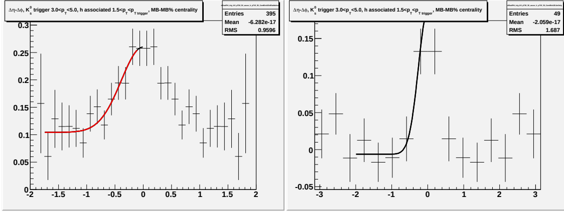
Figure E.5: Going left to right/top to bottom (a) jet-like correlation using \Delta\eta method (b) jet-like correlation using \Delta\phi method (c) correlation integrated over |\Delta\eta| < 0.75 (d) correlation integrated over 0.75 < |\Delta\eta| < 1.75 (e) correlation integrated over 0 < |\Delta\eta| < 1.75 (f) 1-D correlation for 3.0 < p_T^{trigger} < 5.0 GeV/c and 1.5 < p_T^{associated} < p_T^{trigger} GeV/c.
