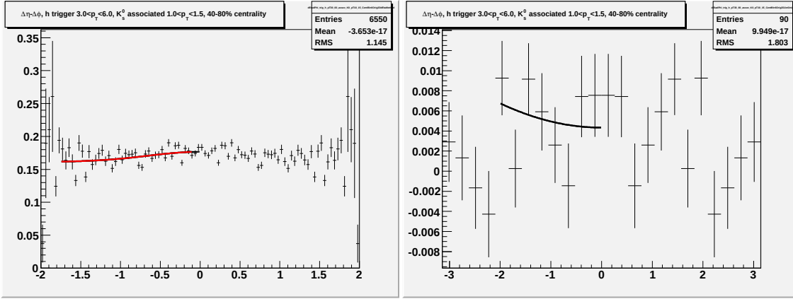
Figure P.10: Going left to right/top to bottom (a) jet-like correlation using \Delta\eta method (b) jet-like correlation using \Delta\phi method (c) correlation integrated over |\Delta\eta| < 0.75 (d) correlation integrated over 0.75 < |\Delta\eta| < 1.75 (e) correlation integrated over 0 < |\Delta\eta| < 1.75 (f) 1-D correlation for 3.0 < p_T^{trigger} < 6.0 GeV/c and 1.0 < p_T^{associated} < 1.5 GeV/c.
