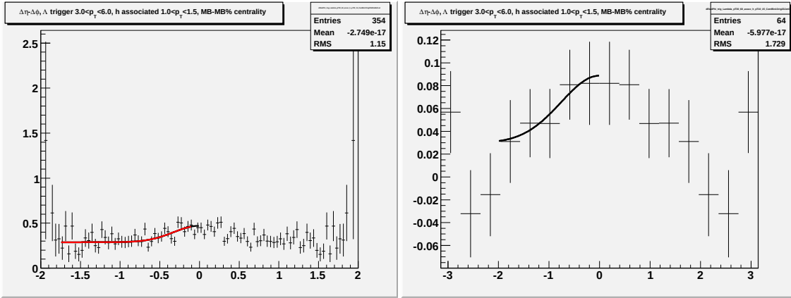
Figure J.2: Going left to right/top to bottom (a) jet-like correlation using \Delta\eta method (b) jet-like correlation using \Delta\phi method (c) correlation integrated over |\Delta\eta| < 0.75 (d) correlation integrated over 0.75 < |\Delta\eta| < 1.75 (e) correlation integrated over 0 < |\Delta\eta| < 1.75 (f) 1-D correlation for 3.0 < p_T^{trigger} < 6.0 GeV/c and 1.0 < p_T^{associated} < 1.5 GeV/c for identified \Lambda triggers.
