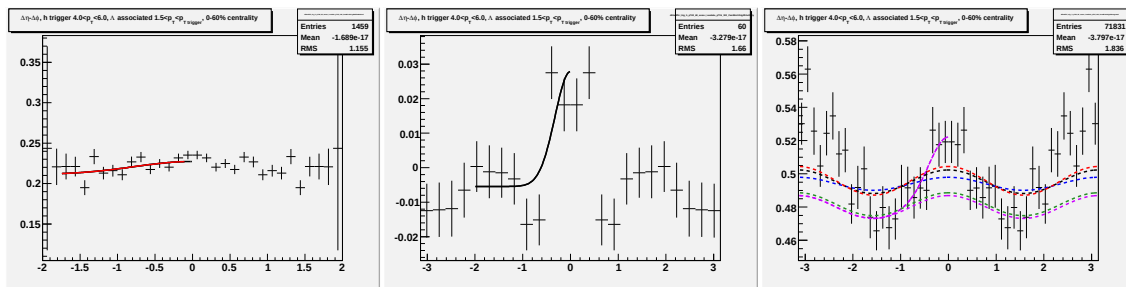
Figure H.4: Going left to right/top to bottom (a) jet-like correlation using \Delta\eta method (b) jet-like correlation using \Delta\phi method (c) correlation integrated over |\Delta\eta| < 0.75 (d) correlation integrated over 0.75 < |\Delta\eta| < 1.75 (e) correlation integrated over 0 < |\Delta\eta| < 1.75 (f) 1-D correlation for 4.0 < p_T^{trigger} < 6.0 GeV/c and 1.5 < p_T^{associated} < p_T^{trigger} GeV/c.
