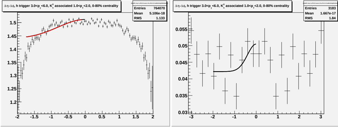
Figure M.6: Going left to right/top to bottom (a) jet-like correlation using \Delta\eta method (b) jet-like correlation using \Delta\phi method (c) correlation integrated over |\Delta\eta| < 0.75 (d) correlation integrated over 0.75 < |\Delta\eta| < 1.75 (e) correlation integrated over 0 < |\Delta\eta| < 1.75 (f) 1-D correlation for 3.0 < p_T^{trigger} < 6.0 GeV/c and 1.0 < p_T^{associated} < 20 GeV/c.
