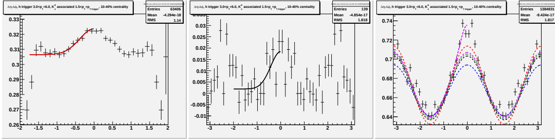
Figure I.4: Going left to right/top to bottom (a) jet-like correlation using \Delta\eta method (b) jet-like correlation using \Delta\phi method (c) correlation integrated over |\Delta\eta| < 0.75 (d) correlation integrated over 0.75 < |\Delta\eta| < 1.75 (e) correlation integrated over 0 < |\Delta\eta| < 1.75 (f) 1-D correlation for 3.0 < p_T^{trigger} < 6.0 GeV/c and 1.5 < p_T^{associated} < p_T^{trigger} GeV/c for 10-40% Au + Au collisions at \sqrt{s_{NN}} = 200 GeV for identified K_S^0 associated particles.
