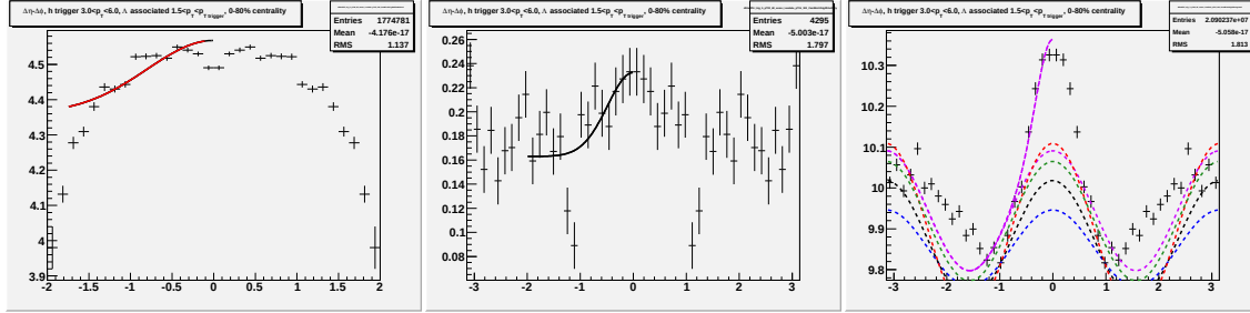
Figure I.6: Going left to right/top to bottom (a) jet-like correlation using \Delta\eta method (b) jet-like correlation using \Delta\phi method (c) correlation integrated over |\Delta\eta| < 0.75 (d) correlation integrated over 0.75 < |\Delta\eta| < 1.75 (e) correlation integrated over 0 < |\Delta\eta| < 1.75 (f) 1-D correlation for 3.0 < p_T^{trigger} < 6.0 GeV/c and 1.5 < p_T^{associated} < p_T^{trigger} GeV/c for 0-12% Au + Au collisions at \sqrt{s_{NN}} = 200 GeV for identified \Lambda associated particles.
