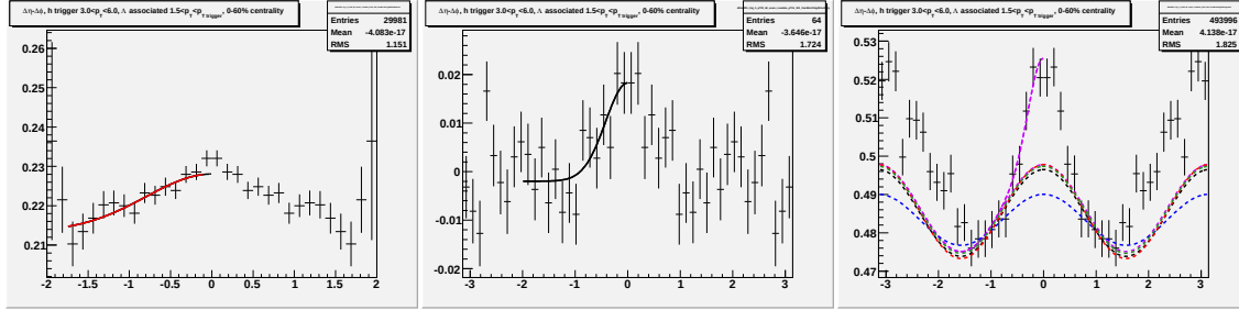
Figure I.2: Going left to right/top to bottom (a) jet-like correlation using \Delta\eta method (b) jet-like correlation using \Delta\phi method (c) correlation integrated over |\Delta\eta| < 0.75 (d) correlation integrated over 0.75 < |\Delta\eta| < 1.75 (e) correlation integrated over 0 < |\Delta\eta| < 1.75 (f) 1-D correlation for 3.0 < p_T^{trigger} < 6.0 GeV/c and 1.5 < p_T^{associated} < p_T^{trigger} GeV/c for 0-60% Cu + Cu collisions at \sqrt{s_{NN}} = 200 GeV for identified \Lambda associated particles.
