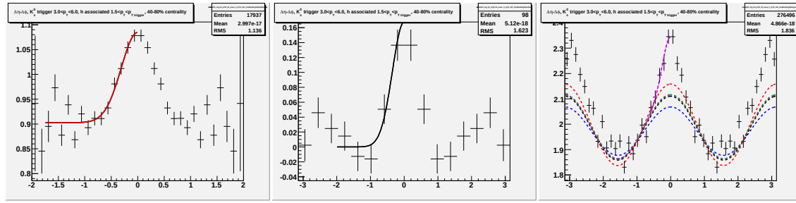
Figure F.17: Going left to right/top to bottom (a) jet-like correlation using \Delta\eta method (b) jet-like correlation using \Delta\phi method (c) correlation integrated over |\Delta\eta| < 0.75 (d) correlation integrated over 0.75 < |\Delta\eta| < 1.75 (e) correlation integrated over 0 < |\Delta\eta| < 1.75 (f) 1-D correlation for 3.0 < p_T^{trigger} < 6.0 GeV/c and 1.5 < p_T^{associated} < p_T^{trigger} GeV/c for K_S^0 trigger particles.
