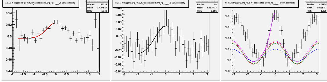
Figure J.1: Going left to right/top to bottom (a) jet-like correlation using \Delta\eta method (b) jet-like correlation using \Delta\phi method (c) correlation integrated over |\Delta\eta| < 0.75 (d) correlation integrated over 0.75 < |\Delta\eta| < 1.75 (e) correlation integrated over 0 < |\Delta\eta| < 1.75 (f) 1-D correlation for 3.0 < p_T^{trigger} < 6.0 GeV/c and 1.5 < p_T^{associated} < p_T^{trigger} GeV/c for 0-60% Cu + Cu collisions at \sqrt{s_{NN}} = 200 GeV for identified K_S^0 associated particles.
