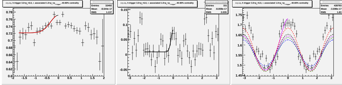
Figure J.8: Going left to right/top to bottom (a) jet-like correlation using \Delta\eta method (b) jet-like correlation using \Delta\phi method (c) correlation integrated over |\Delta\eta| < 0.75 (d) correlation integrated over 0.75 < |\Delta\eta| < 1.75 (e) correlation integrated over 0 < |\Delta\eta| < 1.75 (f) 1-D correlation for 3.0 < p_T^{trigger} < 6.0 GeV/c and 1.5 < p_T^{associated} < p_T^{trigger} GeV/c for 40-80% Au + Au collisions at \sqrt{s_{NN}} = 200 GeV for identified \Lambda associated particles.
