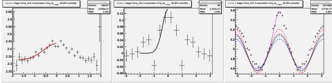
Figure F.10: Going left to right/top to bottom (a) jet-like correlation using \Delta\eta method (b) jet-like correlation using \Delta\phi method (c) correlation integrated over |\Delta\eta| < 0.75 (d) correlation integrated over 0.75 < |\Delta\eta| < 1.75 (e) correlation integrated over 0 < |\Delta\eta| < 1.75 (f) 1-D correlation for 3.0 < p_T^{trigger} < 6.0 GeV/c and 1.5 < p_T^{associated} < p_T^{trigger} GeV/c for \Lambda and \bar{\Lambda} trigger particles.
