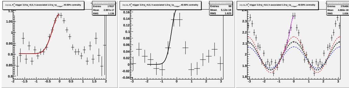
Figure F.13: Going left to right/top to bottom (a) jet-like correlation using \Delta\eta method (b) jet-like correlation using \Delta\phi method (c) correlation integrated over |\Delta\eta| < 0.75 (d) correlation integrated over 0.75 < |\Delta\eta| < 1.75 (e) correlation integrated over 0 < |\Delta\eta| < 1.75 (f) 1-D correlation for 3.0 < p_T^{trigger} < 6.0 GeV/c and 1.5 < p_T^{associated} < p_T^{trigger} GeV/c for K_S^0 trigger particles.
