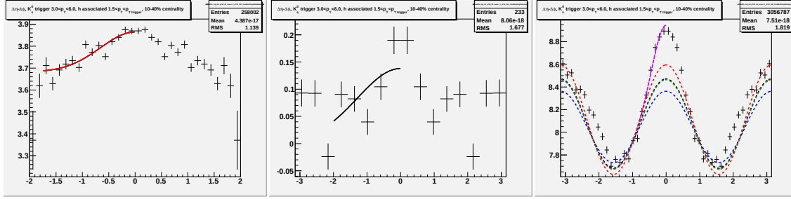
Figure F.12: Going left to right/top to bottom (a) jet-like correlation using \Delta\eta method (b) jet-like correlation using \Delta\phi method (c) correlation integrated over |\Delta\eta| < 0.75 (d) correlation integrated over 0.75 < |\Delta\eta| < 1.75 (e) correlation integrated over 0 < |\Delta\eta| < 1.75 (f) 1-D correlation for 3.0 < p_T^{trigger} < 6.0 GeV/c and 1.5 < p_T^{associated} < p_T^{trigger} GeV/c for K_S^0 trigger particles.
