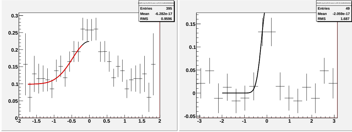
Figure E.3: Going left to right/top to bottom (a) jet-like correlation using \Delta\eta method (b) jet-like correlation using \Delta\phi method (c) correlation integrated over |\Delta\eta| < 0.75 (d) correlation integrated over 0.75 < |\Delta\eta| < 1.75 (e) correlation integrated over 0 < |\Delta\eta| < 1.75 (f) 1-D correlation for 3.0 < p_T^{trigger} < 5.0 GeV/c and 1.5 < p_T^{associated} < p_T^{trigger} GeV/c.
