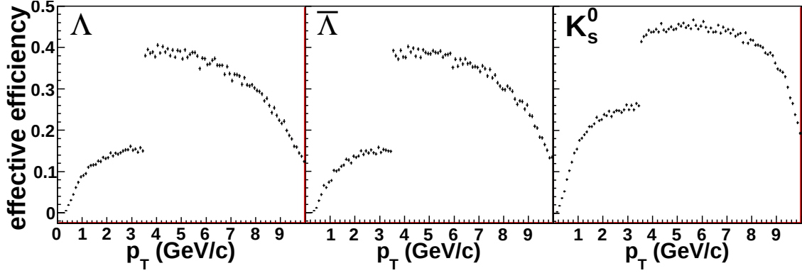
Figure 1.6: Sample effective V^0 reconstruction efficiency in Cu + Cu collisions at \sqrt{s_{NN}} = 200 GeV for the default cuts listed in Table 1.2.
