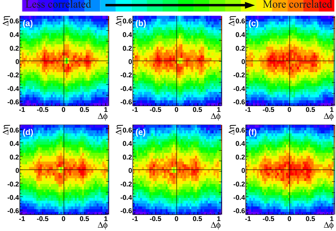
Figure 2.5: The location of the track merging dip in V^0 triggered correlations for a (a) \Lambda trigger with an associated particle with helicity 1 (b) \bar{\Lambda} trigger with an associated particle with helicity 1 (c) K_S^0 trigger with an associated particle with helicity 1 (d) \Lambda trigger with an associated particle with helicity -1 (e) \bar{\Lambda} trigger with an associated particle with helicity -1 (f) K_S^0 trigger with an associated particle with helicity -1 in 0-80% central Au + Au collisions at \sqrt{s_{NN}} = 200 GeV.
