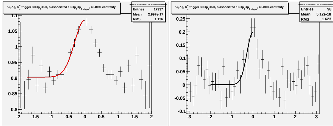
Figure F.13: Going left to right/top to bottom (a) jet-like correlation using \Delta\eta method (b) jet-like correlation using \Delta\phi method (c) correlation integrated over |\Delta\eta| < 0.75 (d) correlation integrated over 0.75 < |\Delta\eta| < 1.75 (e) correlation integrated over 0 < |\Delta\eta| < 1.75 (f) 1-D correlation for 3.0 < p_T^{\text{trigger}} < 6.0 GeV/c and 1.5 < p_T^{\text{associated}} < p_T^{\text{trigger}} GeV/c for K_S^0 trigger particles.
