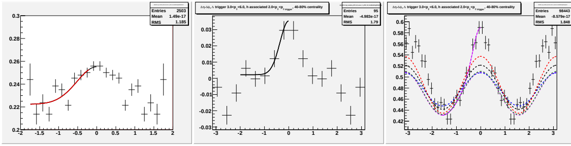
Figure G.16: Going left to right/top to bottom (a) jet-like correlation using \Delta\eta method (b) jet-like correlation using \Delta\phi method (c) correlation integrated over |\Delta\eta| < 0.75 (d) correlation integrated over 0.75 < |\Delta\eta| < 1.75 (e) correlation integrated over 0 < |\Delta\eta| < 1.75 (f) 1-D correlation for 3.0 < p_T^{trigger} < 6.0 GeV/c and 2.0 < p_T^{associated} < 3.0 GeV/c for \Lambda and \bar{\Lambda} trigger particles.
