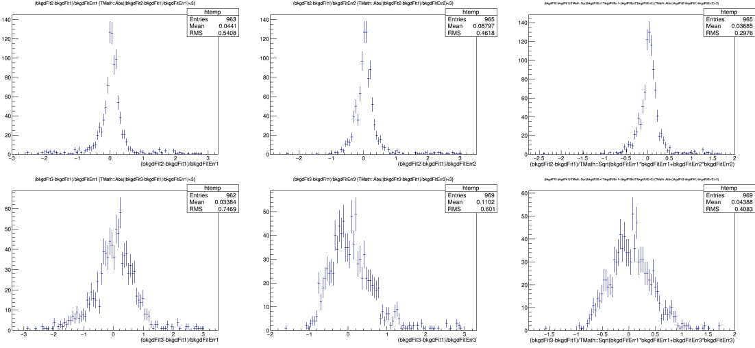
Figure J.4: Fits
