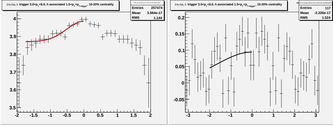
Figure F.9: Going left to right/top to bottom (a) jet-like correlation using \Delta\eta method (b) jet-like correlation using \Delta\phi method (c) correlation integrated over |\Delta\eta| < 0.75 (d) correlation integrated over 0.75 < |\Delta\eta| < 1.75 (e) correlation integrated over 0 < |\Delta\eta| < 1.75 (f) 1-D correlation for 3.0 < p_T^{trigger} < 6.0 GeV/c and 1.5 < p_T^{associated} < 6.0 GeV/c for \Lambda and \bar{\Lambda} trigger particles.
