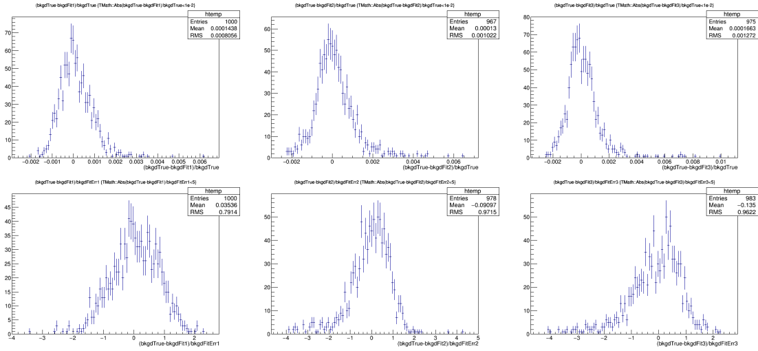
Figure J.3: Fits
