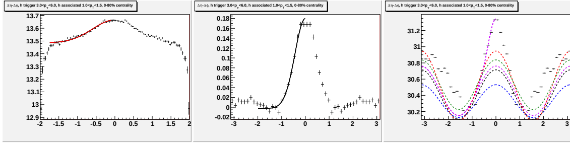
Figure I.14: Going left to right/top to bottom (a) jet-like correlation using \Delta\eta method (b) jet-like correlation using \Delta\phi method (c) correlation integrated over |\Delta\eta| < 0.75 (d) correlation integrated over 0.75 < |\Delta\eta| < 1.75 (e) correlation integrated over 0 < |\Delta\eta| < 1.75 (f) 1-D correlation for 3.0 < p_T^{trigger} < 6.0 GeV/c and 1.0 < p_T^{associated} < 1.5 GeV/c.
