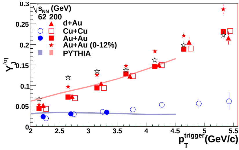
Figure G.2: p_T^{trigger} dependence of Y_{Jet} for unidentified hadrons for 1.5 \text{ GeV/c} < p_T^{associated} < p_T^{trigger} for 0-60% central Cu + Cu and 0-80% central Au + Au collisions at \sqrt{s_{NN}} = 62 \text{ GeV} and minimum bias d + Au , 0-60% central Cu + Cu and 40-80% central Au + Au collisions at \sqrt{s_{NN}} = 200 \text{ GeV} . Red solid stars show Y_{Jet} for the \Delta\eta method using bin counting and open black stars show Y_{Jet} for the \Delta\eta method using a Gaussian fit in \Delta\eta .
