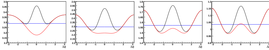
Figure F.2: Projections of ridge, \cos(\Delta\phi) , and v_2 modulated background terms from fits from left to right for 0-12%, 10-20%, 20-30%, and 30-40% Au + Au \sqrt{s_{NN}} = 200 GeV. The black line shows the total, the blue line shows the v_2 modulated background, and the red line shows the v_2 modulated background plus the \cos(\Delta\phi) term. Note that the jet-like correlation has been omitted from these projections.
