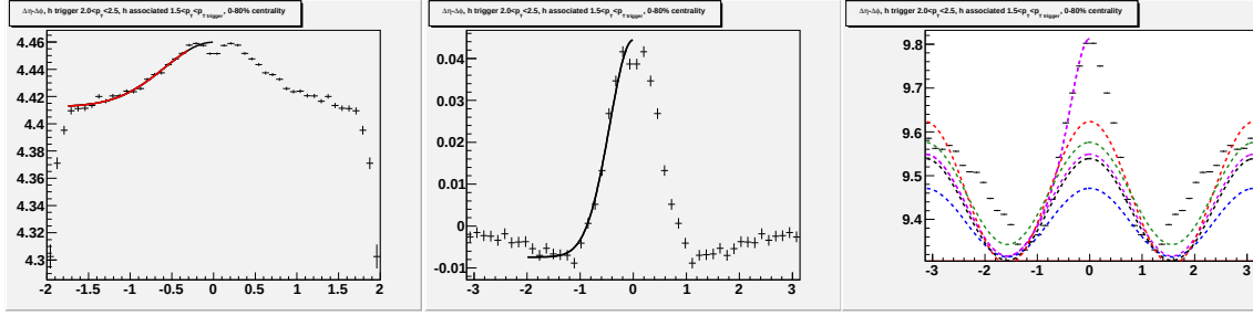
Figure G.27: Going left to right/top to bottom (a) jet-like correlation using \Delta\eta method (b) jet-like correlation using \Delta\phi method (c) correlation integrated over |\Delta\eta| < 0.75 (d) correlation integrated over 0.75 < |\Delta\eta| < 1.75 (e) correlation integrated over 0 < |\Delta\eta| < 1.75 (f) 1-D correlation for 2.0 < p_T^{trigger} < 2.5 GeV/c and 1.5 < p_T^{associated} < p_T^{trigger} GeV/c.
