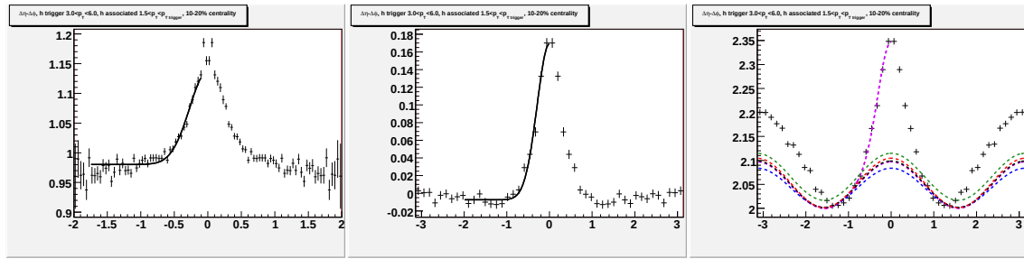
Figure H.9: Going left to right/top to bottom (a) jet-like correlation using \Delta\eta method (b) jet-like correlation using \Delta\phi method (c) correlation integrated over |\Delta\eta| < 0.75 (d) correlation integrated over 0.75 < |\Delta\eta| < 1.75 (e) correlation integrated over 0 < |\Delta\eta| < 1.75 (f) 1-D correlation for 3.0 < p_T^{trigger} < 6.0 GeV/c and 1.5 < p_T^{associated} < p_T^{trigger} GeV/c for 10-20% Cu + Cu collisions at \sqrt{s_{NN}} = 200 GeV.
