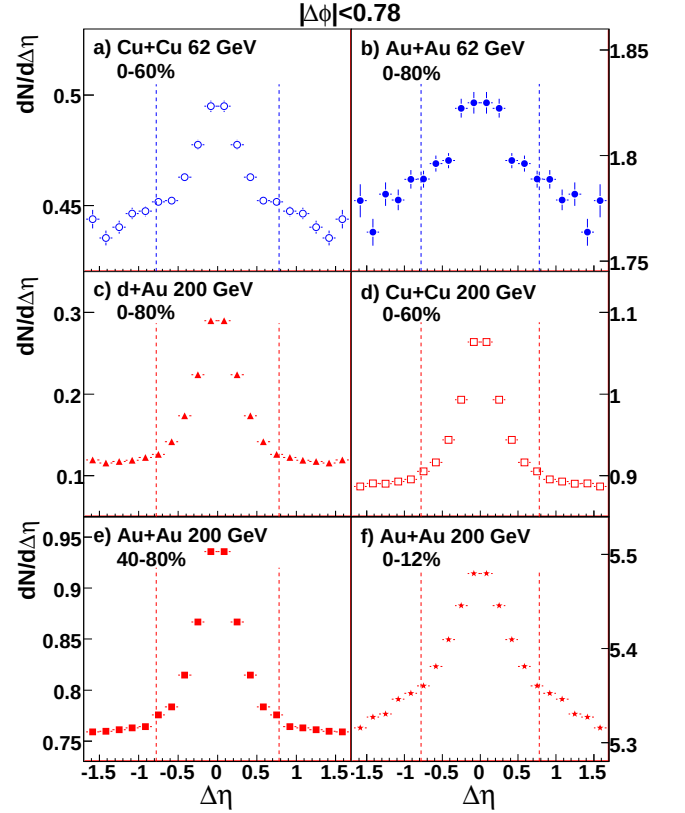
FIG. 5: Sample correlations in \Delta\eta for 3 < p_T^{trigger} < 6 GeV/c and 1.5 GeV/c < p_T^{associated} < p_T^{trigger} for (a) 0-60% central Cu + Cu at \sqrt{s_{NN}} = 62 GeV (b) 0-80% central Au + Au at \sqrt{s_{NN}} = 62 GeV, (c) minimum bias d+Au at \sqrt{s_{NN}} = 200 GeV, (d) 0-60% central Cu + Cu at \sqrt{s_{NN}} = 200 GeV, (e) 40-80% Au + Au at \sqrt{s_{NN}} = 200 GeV, and (f) 0-12% central Au + Au at \sqrt{s_{NN}} = 200 GeV. Lines show the \Delta\eta range where the jet-like yield is determined. Color online.
