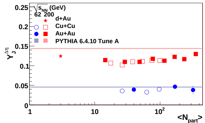
FIG. 8: Dependence of jet-like correlation yields on N_{part} for minimum bias d + Au , 0-60% Cu + Cu at \sqrt{s_{NN}} = 62 GeV and \sqrt{s_{NN}} = 200 GeV, 0-80% Au + Au at \sqrt{s_{NN}} = 62 GeV, and 0-12% and 40-80% Au + Au at \sqrt{s_{NN}} = 200 GeV. Comparisons to PYTHIA, N_{part} = 2 , are shown as shaded bands. Color online.
