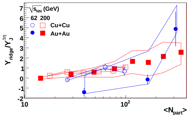
FIG. 13: Ratio of ridge and jet-like yields as a function of N_{part} . Color online.
