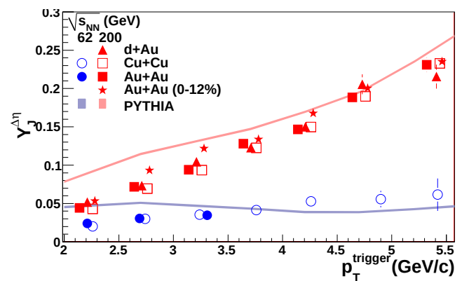
FIG. 9: Dependence of jet-like correlation yield on p_T^{trigger} for minimum bias d + Au , 0-60% Cu + Cu at \sqrt{s_{NN}} = 62 GeV and \sqrt{s_{NN}} = 200 GeV, 0-80% Au + Au at \sqrt{s_{NN}} = 62 GeV, and 0-12% and 40-80% Au + Au at \sqrt{s_{NN}} = 200 GeV. Comparisons to PYTHIA are shown as shaded bands. Color online.
