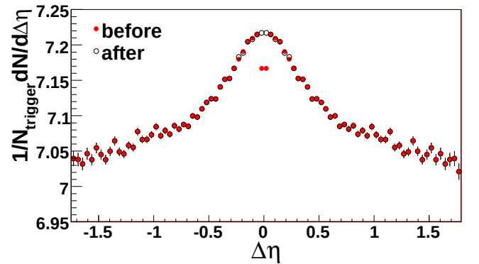
FIG. 4: The raw correlation in \Delta\eta for charged-charged correlations for 3 \text{ GeV}/c < p_T^{trig} < 6 \text{ GeV}/c and 1.5 \text{ GeV}/c < p_T^{assoc} < p_T^{trig} for 0-12% central Au+Au collisions before and after the track merging correction is applied
