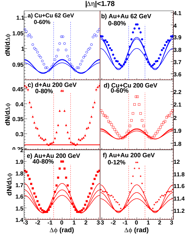
FIG. 6: Sample correlations in \Delta\phi for 3 < p_T^{trigger} < 6 GeV/ c and 1.5 GeV/ c < p_T^{associated} < p_T^{trigger} for (a) 0-60% central Cu + Cu at \sqrt{s_{NN}} = 62 GeV (b) 0-80% central Au + Au at \sqrt{s_{NN}} = 62 GeV, (c) minimum bias d+Au at \sqrt{s_{NN}} = 200 GeV, (d) 0-60% central Cu + Cu at \sqrt{s_{NN}} = 200 GeV, (e) 40-80% Au + Au at \sqrt{s_{NN}} = 200 GeV, and (f) 0-12% central Au + Au at \sqrt{s_{NN}} = 200 GeV. Lines show the estimated background using the ZYAM method with the range of v_2 used for the determination of the systematic errors.
