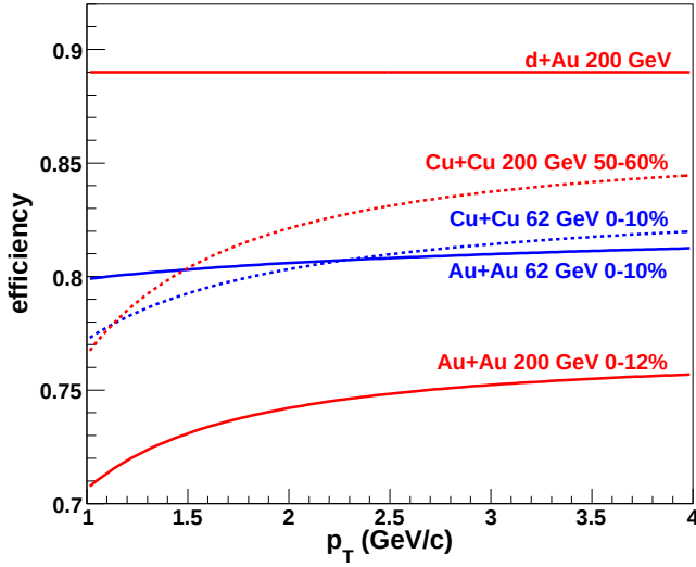
FIG. 1: Transverse momentum dependence of the reconstruction efficiency of charged particles in the TPC in various collision systems, energies and centrality bins. Note the zero suppression of the axes.
