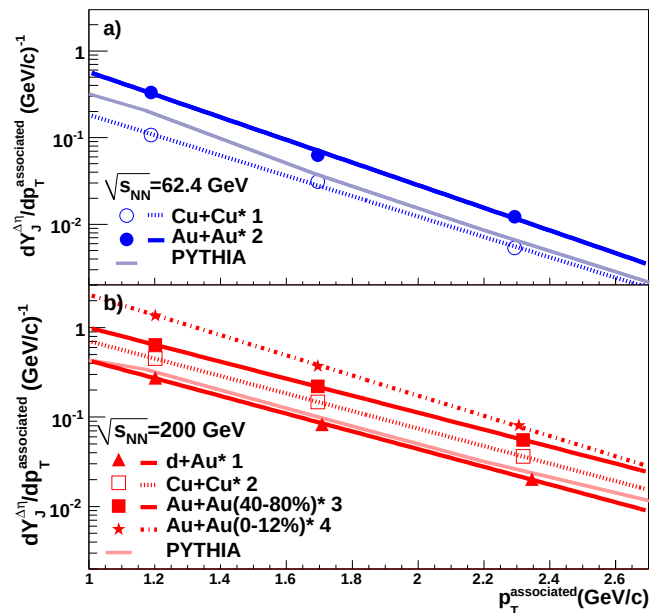
FIG. 10: Dependence of jet-like correlation yield on p_T^{associated} for (a) 0-60% Cu + Cu and 0-80% Au + Au collisions at \sqrt{s_{NN}} = 62.4 GeV and (b) minimum bias d + Au , 0-60% Cu + Cu , 0-12% Au + Au and 40-80% Au + Au collisions at \sqrt{s_{NN}} = 200 GeV. Comparisons to PYTHIA are shown as lines. 5% systematic error due to the uncertainty on the associated particle's efficiency not shown. Color online.
