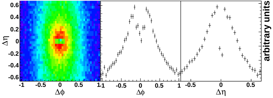
FIG. 2: Two-particle di-hadron correlation function in (\Delta\phi, \Delta\eta) space for p_T^{trig}=3-6 GeV/c and 1.5 GeV/c < p_T^{associated} < p_T^{trigger} in 0-12% central Au + Au collisions at \sqrt{s_{NN}} = 200 GeV, not corrected for track merging (left). The projection of the correlation function in \Delta\phi for |\Delta\eta| < 0.042 is shown in the middle and the projection in \Delta\eta for |\Delta\phi| < 0.17 on the right.
