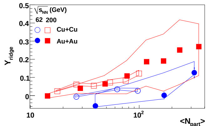
FIG. 12: Dependence of ridge yield on N_{\text{part}} for Cu + Cu and Au + Au collisions at \sqrt{s_{NN}} = 62.4 \text{ GeV} and 200 \text{ GeV} . Systematic errors due to v_2 are shown as solid lines. 5% systematic error due to the uncertainty on the associated particle's efficiency not shown. Color online.
