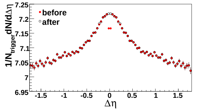
FIG. 4: The raw correlation in \Delta\eta for charged-charged correlations for 3 GeV/c < p_T^{trig} < 6 GeV/c and 1.5 GeV/c < p_T^{assoc} < p_T^{trig} for 0-12% central Au + Au collisions before and after the track merging correction is applied. The data have been reflected about \Delta\eta = 0 .
