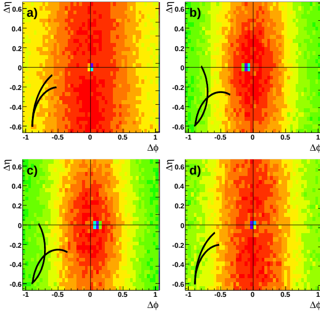
FIG. 3: The dip region in (\Delta\phi, \Delta\eta) uncorrected charged-charged correlations 0-12% in central Au + Au collisions at \sqrt{s_{NN}} = 200 GeV for 3 GeV/c < p_T^{trig} < 6 GeV/c and 1.5 GeV/c < p_T^{assoc} < p_T^{trig} unfolded to four helicity combinations of trigger and associated particles: (a) (h_{trig}, h_{assoc}) = (1,1) , (b) (h_{trig}, h_{assoc}) = (1,-1) , (c) (h_{trig}, h_{assoc}) = (-1,1) , and (d) (h_{trig}, h_{assoc}) = (-1,-1) . Cartoons indicate which dips are from track merging and which are from track crossing.
