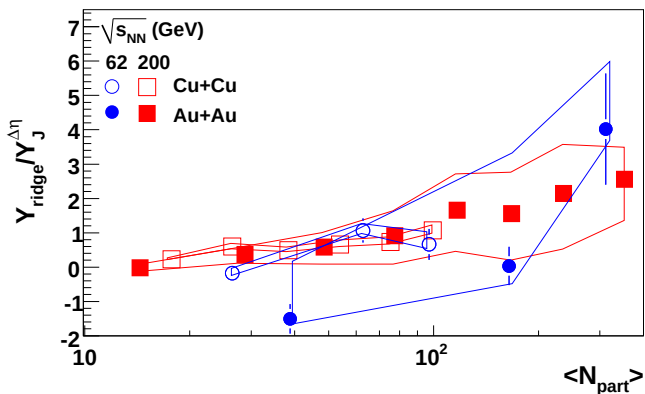
FIG. 13: Ratio of ridge and jet-like yields as a function of N_{part} . Systematic errors due to v_2 are shown as solid lines. 5% systematic error due to the uncertainty on the associated particle's efficiency not shown. Color online.
