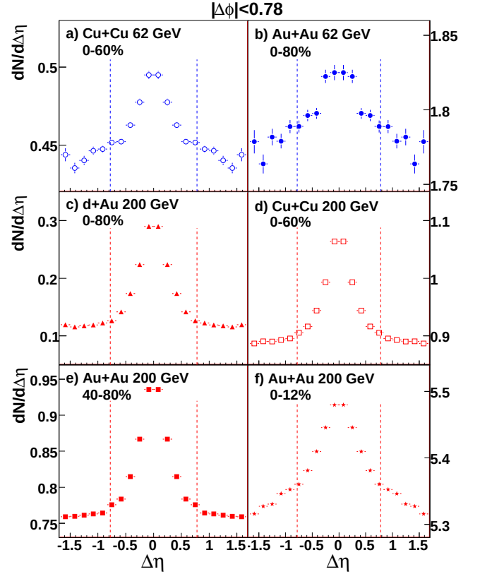
FIG. 5: Sample correlations in \Delta\eta for 3 < p_T^{trigger} < 6 GeV/c and 1.5 GeV/c < p_T^{associated} < p_T^{trigger} for (a) 0-60% central Cu + Cu at \sqrt{s_{NN}} = 62 GeV (b) 0-80% central Au + Au at \sqrt{s_{NN}} = 62 GeV, (c) minimum bias d+Au at \sqrt{s_{NN}} = 200 GeV, (d) 0-60% central Cu + Cu at \sqrt{s_{NN}} = 200 GeV, (e) 40-80% Au + Au at \sqrt{s_{NN}} = 200 GeV, and (f) 0-12% central Au + Au at \sqrt{s_{NN}} = 200 GeV. Lines show the \Delta\eta range where the jet-like yield is determined. Color online.
