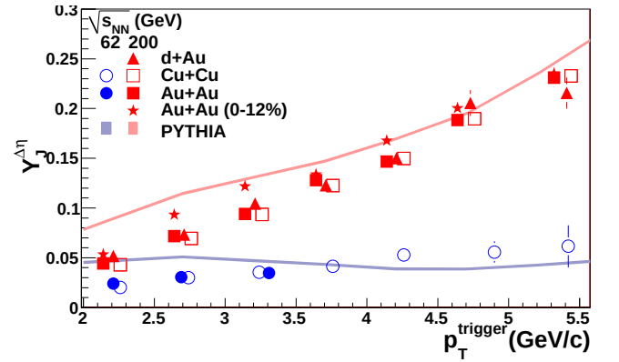
FIG. 9: Dependence of jet-like correlation yield on p_T^{trigger} for minimum bias d+Au , 0-60% Cu+Cu at \sqrt{s_{NN}} = 62 GeV and \sqrt{s_{NN}} = 200 GeV, 0-80% Au+Au at \sqrt{s_{NN}} = 62 GeV, and 0-12% and 40-80% Au+Au at \sqrt{s_{NN}} = 200 GeV. Comparisons to PYTHIA are shown as shaded bands. Color online.
