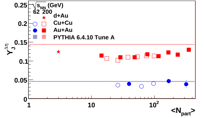
FIG. 8: Dependence of jet-like correlation yields on N_{part} for minimum bias d+Au , 0-60% Cu+Cu at \sqrt{s_{NN}} = 62 GeV and \sqrt{s_{NN}} = 200 GeV, 0-80% Au+Au at \sqrt{s_{NN}} = 62 GeV, and 0-12% and 40-80% Au+Au at \sqrt{s_{NN}} = 200 GeV. Comparisons to PYTHIA, N_{part} = 2 , are shown as shaded bands. Color online.
