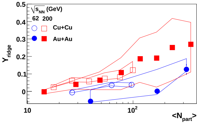
FIG. 12: Dependence of ridge yield on N_{\text{part}} for Cu+Cu and Au+Au collisions at \sqrt{s_{\text{NN}}} = 62.4 \text{ GeV} and 200 \text{ GeV} . Systematic errors due to v_2 are shown as solid lines. The 5% systematic error due to the uncertainty on the associated particle's efficiency is not shown. Color online.
