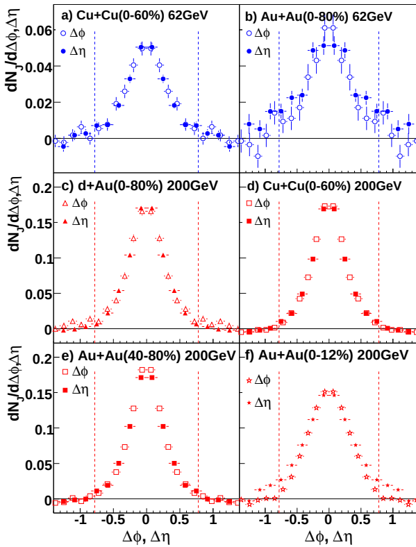
FIG. 7: Background subtracted sample correlations for 3 < p_T^{\text{trigger}} < 6 GeV/c and 1.5 GeV/c < p_T^{\text{associated}} < p_T^{\text{trigger}} on the near-side for (a) 0-60% Cu+Cu at \sqrt{s_{\text{NN}}} = 62.4 GeV, (b) 0-80% Au+Au at \sqrt{s_{\text{NN}}} = 62.4 GeV, (c) minimum bias d+Au collisions at \sqrt{s_{\text{NN}}} = 200 GeV, (d) 0-60% Cu+Cu at \sqrt{s_{\text{NN}}} = 200 GeV, (e) 40-80% Au+Au at \sqrt{s_{\text{NN}}} = 200 GeV and (f) 0-12% central Au+Au at \sqrt{s_{\text{NN}}} = 200 GeV. The dependence of the jet-like correlation is shown as a function of \Delta\phi ( |\Delta\eta| < 1.78 ) in open symbols and \Delta\eta ( |\Delta\phi| < 0.78 ) in closed symbols. Lines show the \Delta\phi and \Delta\eta ranges where the jet-like yield is determined. The data are averaged between positive and negative \Delta\eta ( \Delta\phi ) and reflected in the plot. Color online.
