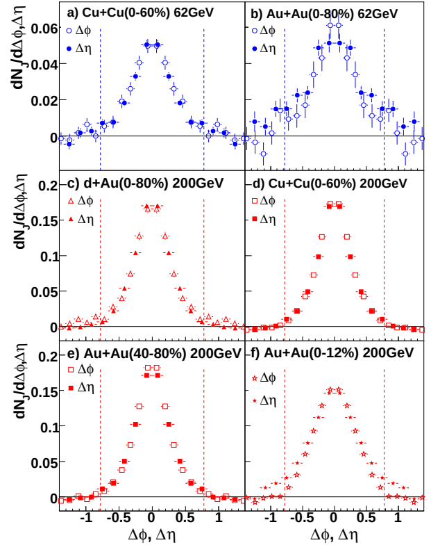
FIG. 7: Background subtracted sample correlations for 3 < p_T^{\text{trigger}} < 6 GeV/c and 1.5 \text{ GeV/c} < p_T^{\text{associated}} < p_T^{\text{trigger}} on the near-side for (a) 0-60% Cu+Cu at \sqrt{s_{\text{NN}}} = 62.4 GeV, (b) 0-80% Au+Au at \sqrt{s_{\text{NN}}} = 62.4 GeV, (c) minimum bias d+Au collisions at \sqrt{s_{\text{NN}}} = 200 GeV, (d) 0-60% Cu+Cu at \sqrt{s_{\text{NN}}} = 200 GeV, (e) 40-80% Au+Au at \sqrt{s_{\text{NN}}} = 200 GeV and (f) 0-12% central Au+Au at \sqrt{s_{\text{NN}}} = 200 GeV. The dependence of the jet-like correlation is shown as a function of \Delta\phi ( |\Delta\eta| < 1.78 ) in open symbols and \Delta\eta ( |\Delta\phi| < 0.78 ) in closed symbols. Lines show the \Delta\phi and \Delta\eta ranges where the jet-like yield is determined. The data are averaged between positive and negative \Delta\eta ( \Delta\phi ) and reflected in the plot. Color online.
