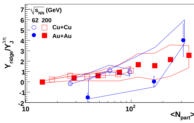
FIG. 13: Ratio of the ridge and jet-like yields as a function of N_{\text{part}} . Systematic errors due to v_2 are shown as solid lines. Color online.
