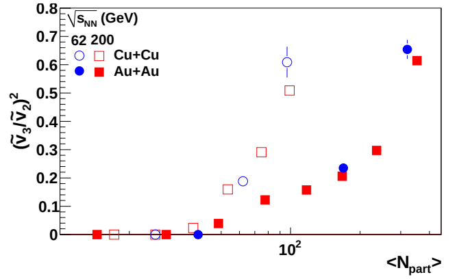
FIG. 14: (\tilde{v}_3/\tilde{v}_2)^2 ratio as a function of N_{\text{part}} . Statistical errors only. Color online.
