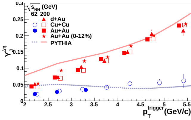
FIG. 9: Dependence of jet-like yield on p_T^{\text{trigger}} for minimum bias d+Au, 0-60% Cu+Cu at \sqrt{s_{\text{NN}}} = 62.4 GeV and \sqrt{s_{\text{NN}}} = 200 GeV, 0-80% Au+Au at \sqrt{s_{\text{NN}}} = 62.4 GeV, and 0-12% Au+Au at \sqrt{s_{\text{NN}}} = 200 GeV. Comparisons to PYTHIA are shown as shaded bands. The 5% systematic error due to the uncertainty on the associated particle's efficiency is not shown. Color online.
