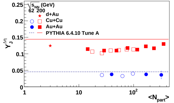
FIG. 8: Dependence of jet-like yields on N_{\text{part}} for 3 < p_T^{\text{trigger}} < 6 GeV/c and 1.5 GeV/c < p_T^{\text{associated}} < p_T^{\text{trigger}} for Cu+Cu, and Au+Au at \sqrt{s_{\text{NN}}} = 62.4 GeV and d+Au, Cu+Cu and Au+Au at \sqrt{s_{\text{NN}}} = 200 GeV. Comparisons to PYTHIA, N_{\text{part}} = 2 , are shown as shaded bands. The 5% systematic error due to the uncertainty on the associated particle's efficiency is not shown. The background level and v_2 values used for the extraction of these yields are given in Table III. Color online.
