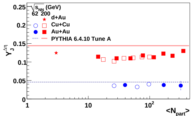
FIG. 8: Dependence of jet-like yields on N_{\text{part}} for 3 < p_T^{\text{trigger}} < 6 GeV/c and 1.5 GeV/c < p_T^{\text{associated}} < p_T^{\text{trigger}} for Cu+Cu, and Au+Au at \sqrt{s_{NN}} = 62.4 GeV and d+Au, Cu+Cu and Au+Au at \sqrt{s_{NN}} = 200 GeV. Comparisons to PYTHIA, N_{\text{part}} = 2 , are shown as shaded bands. The 5% systematic error due to the uncertainty on the associated particle's efficiency is not shown. The background level and v_2 values used for the extraction of these yields are given in Table III. Color online.
