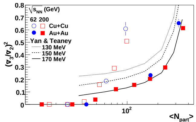
FIG. 14: (\tilde{v}_3/\tilde{v}_2)^2 ratio as a function of N_{\text{part}} . Statistical errors only. Color online.
