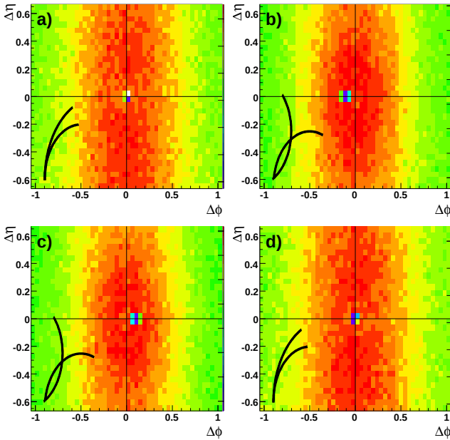
FIG. 3: The dip region in (\Delta\phi, \Delta\eta) uncorrected di-hadron correlations in 0-12% central Au+Au collisions at \sqrt{s_{\text{NN}}} = 200 GeV for 3 < p_T^{\text{trigger}} < 6 GeV/c and 1.5 GeV/c < p_T^{\text{associated}} < p_T^{\text{trigger}} in the four helicity combinations of trigger and associated particles: (a) (h_{\text{trig}}, h_{\text{assoc}}) = (1,1) , (b) (h_{\text{trig}}, h_{\text{assoc}}) = (1,-1) , (c) (h_{\text{trig}}, h_{\text{assoc}}) = (-1,1) , and (d) (h_{\text{trig}}, h_{\text{assoc}}) = (-1,-1) . Cartoons indicate which dips are from track merging and which are from track crossing.
