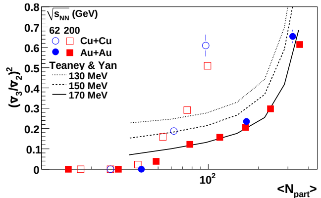
FIG. 14: (\tilde{v}_3/\tilde{v}_2)^2 ratio as a function of N_{\text{part}} . Statistical errors only. The data are compared to a hydrodynamical calculation using lattice equation of state with three different freeze-out temperatures in Au+Au collisions at \sqrt{s_{\text{NN}}} = 200 GeV from [63](lines). Color online.
