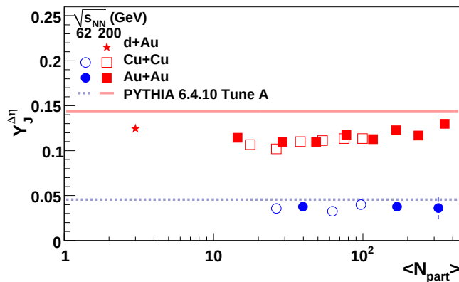
FIG. 8: Dependence of jet-like yields on N_{\text{part}} for 3 < p_T^{\text{trigger}} < 6 GeV/c and 1.5 GeV/c < p_T^{\text{associated}} < p_T^{\text{trigger}} for Cu+Cu, and Au+Au at \sqrt{s_{\text{NN}}} = 62.4 GeV and d+Au, Cu+Cu and Au+Au at \sqrt{s_{\text{NN}}} = 200 GeV. Comparisons to PYTHIA, N_{\text{part}} = 2 , are shown as shaded bands. The 5% systematic error due to the uncertainty on the associated particle's efficiency is not shown. The background level and v_2 values used for the extraction of these yields are given in Table III. Color online.
