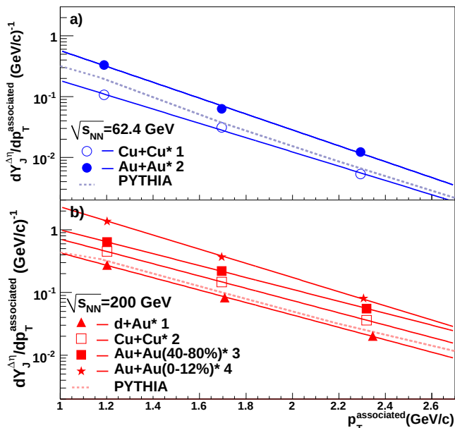
FIG. 10: Dependence of jet-like yield on p_T^{\text{associated}} for (a) 0-60% Cu+Cu and 0-80% Au+Au collisions at \sqrt{s_{\text{NN}}} = 62.4 GeV and (b) minimum bias d+Au, 0-60% Cu+Cu, 0-12% Au+Au and 40-80% Au+Au collisions at \sqrt{s_{\text{NN}}} = 200 GeV. Solid lines through the data points are fits to the data. Comparisons to PYTHIA are shown as dashed lines. The 5% systematic error due to the uncertainty on the associated particle's efficiency is not shown. Color online.
