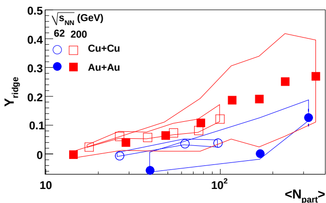
FIG. 12: Dependence of ridge on N_{\text{part}} for 3 < p_T^{\text{trigger}} < 6 \text{ GeV}/c and 1.5 \text{ GeV}/c < p_T^{\text{associated}} < p_T^{\text{trigger}} for Cu+Cu, and Au+Au at \sqrt{s_{\text{NN}}} = 62.4 \text{ GeV} and d+Au, Cu+Cu and Au+Au at \sqrt{s_{\text{NN}}} = 200 \text{ GeV} . Systematic errors due to v_2 are shown as solid lines. The 5% systematic error due to the uncertainty on the associated particle's efficiency is not shown. Color online.
