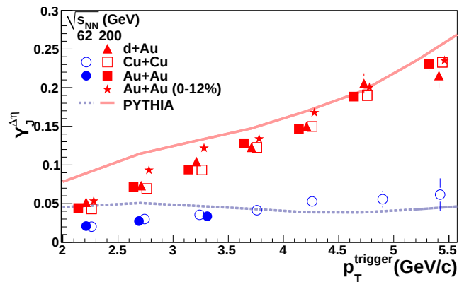
FIG. 9: Dependence of jet-like yield on p_T^{\text{trigger}} for minimum bias d+Au, 0-60% Cu+Cu at \sqrt{s_{\text{NN}}} = 62.4 GeV and \sqrt{s_{\text{NN}}} = 200 GeV, 0-80% Au+Au at \sqrt{s_{\text{NN}}} = 62.4 GeV, and 0-12% and 40-80% Au+Au at \sqrt{s_{\text{NN}}} = 200 GeV. Comparisons to PYTHIA are shown as shaded bands. The 5% systematic error due to the uncertainty on the associated particle's efficiency is not shown. Color online.
