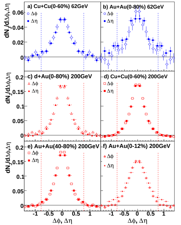
FIG. 7: Background subtracted sample correlations for 3 < p_T^{\text{trigger}} < 6 GeV/c and 1.5 \text{ GeV}/c < p_T^{\text{associated}} < p_T^{\text{trigger}} on the near-side for (a) 0-60% Cu+Cu at \sqrt{s_{\text{NN}}} = 62.4 GeV, (b) 0-80% Au+Au at \sqrt{s_{\text{NN}}} = 62.4 GeV, (c) minimum bias d+Au collisions at \sqrt{s_{\text{NN}}} = 200 GeV, (d) 0-60% Cu+Cu at \sqrt{s_{\text{NN}}} = 200 GeV, (e) 40-80% Au+Au at \sqrt{s_{\text{NN}}} = 200 GeV and (f) 0-12% central Au+Au at \sqrt{s_{\text{NN}}} = 200 GeV. The dependence of the jet-like correlation is shown as a function of \Delta\phi ( |\Delta\eta| < 1.78 ) in open symbols and \Delta\eta ranges where the jet-like yield is determined. The data are averaged between positive and negative \Delta\eta ( \Delta\phi ) and reflected in the plot. Color online.
