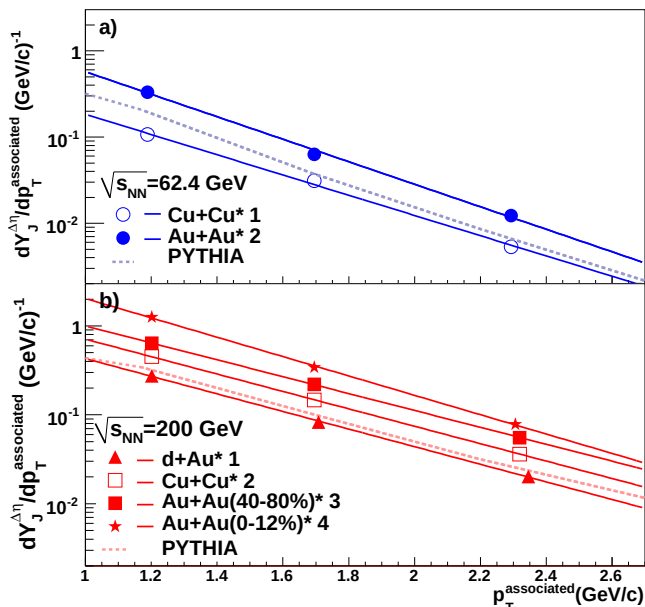
FIG. 10: Dependence of jet-like yield on p_T^{\text{associated}} for 3 < p_T^{\text{trigger}} < 6 GeV/c for (a) 0-60% Cu+Cu and 0-80% Au+Au collisions at \sqrt{s_{\text{NN}}} = 62.4 GeV and (b) minimum bias d+Au, 0-60% Cu+Cu, 0-12% Au+Au and 40-80% Au+Au collisions at \sqrt{s_{\text{NN}}} = 200 GeV. Solid lines through the data points are fits to the data. Comparisons to PYTHIA are shown as dashed lines. The 5% systematic error due to the uncertainty on the associated particle's efficiency is not shown. Color on-
