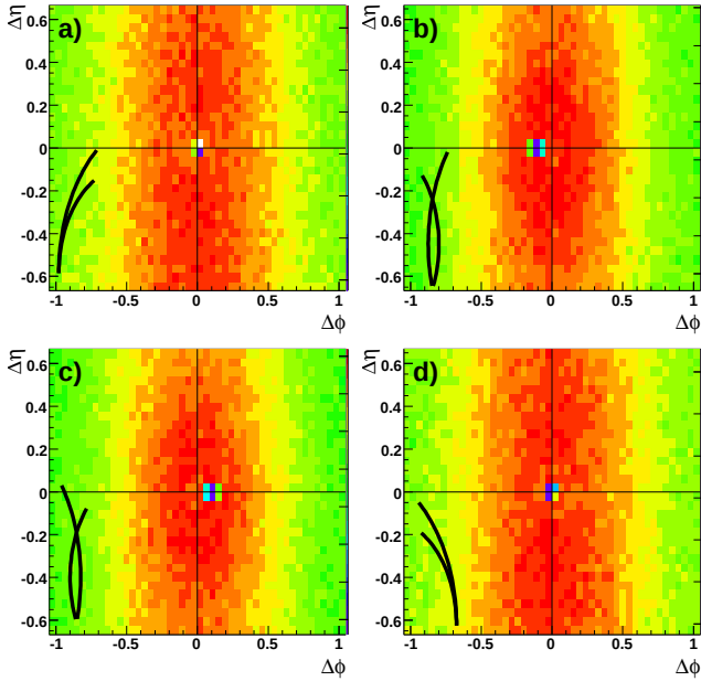
FIG. 3: The dip region in (\Delta\phi, \Delta\eta) uncorrected di-hadron correlations in 0-12% central Au+Au collisions at \sqrt{s_{\text{NN}}} = 200 GeV for 3 < p_T^{\text{trigger}} < 6 GeV/c and 1.5 GeV/c < p_T^{\text{associated}} < p_T^{\text{trigger}} in the four helicity combinations of trigger and associated particles: (a) (h_{\text{trig}}, h_{\text{assoc}}) = (1,1) , (b) (h_{\text{trig}}, h_{\text{assoc}}) = (1,-1) , (c) (h_{\text{trig}}, h_{\text{assoc}}) = (-1,1) , and (d) (h_{\text{trig}}, h_{\text{assoc}}) = (-1,-1) . Cartoons indicate which dips are from track merging and which are from track crossing. Color online.
