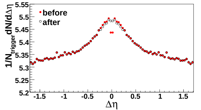
FIG. 4: The raw correlation in \Delta\eta for di-hadron correlations for 3 < p_T^{\text{trigger}} < 6 GeV/c and 1.5 GeV/c < p_T^{\text{associated}} < p_T^{\text{trigger}} for 0-12% central Au+Au collisions for |\Delta\phi| < 0.78 before and after the track merging correction is applied. The data have been reflected about \Delta\eta = 0 . Color online.
