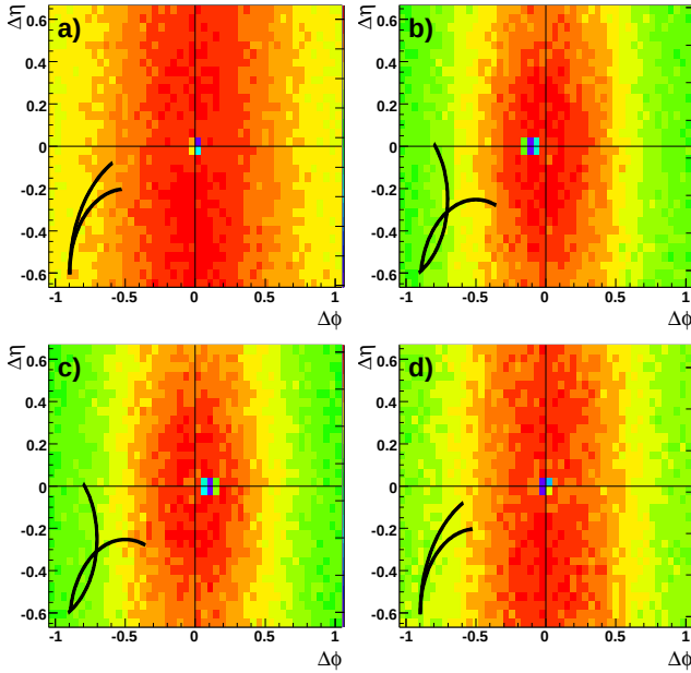
FIG. 3: The dip region in (\Delta\phi, \Delta\eta) uncorrected charged-charged correlations in 0-12% central Au + Au collisions at \sqrt{s_{NN}} = 200 GeV for 3 < p_T^{\text{trigger}} < 6 GeV/c and 1.5 GeV/c < p_T^{\text{associated}} < p_T^{\text{trigger}} in the four helicity combinations of trigger and associated particles: (a) (h_{\text{trig}}, h_{\text{assoc}}) = (1,1) , (b) (h_{\text{trig}}, h_{\text{assoc}}) = (1,-1) , (c) (h_{\text{trig}}, h_{\text{assoc}}) = (-1,1) , and (d) (h_{\text{trig}}, h_{\text{assoc}}) = (-1,-1) . Cartoons indicate which dips are from track merging and which are from track crossing.
