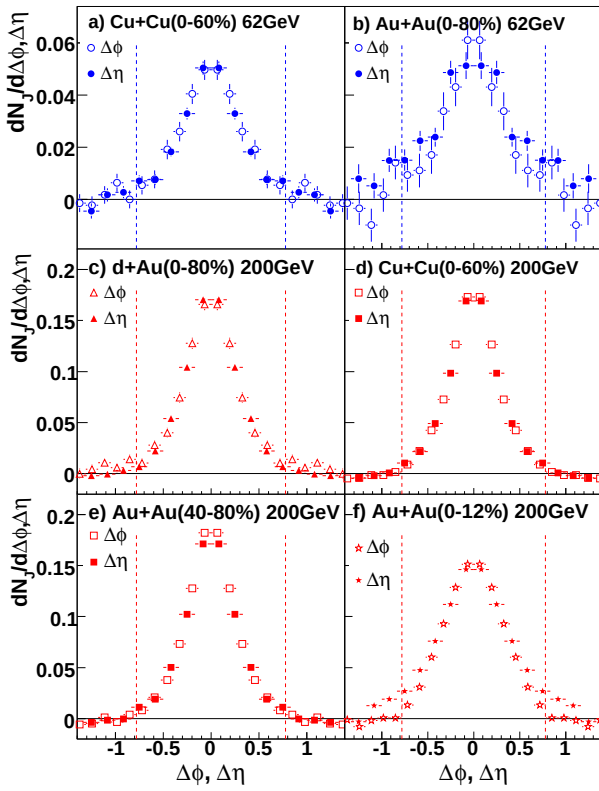
FIG. 7: Background subtracted sample correlations for 3 < p_T^{\text{trigger}} < 6 GeV/c and 1.5 GeV/c < p_T^{\text{associated}} < p_T^{\text{trigger}} on the near-side for (a) 0-60% Cu+Cu at \sqrt{s_{\text{NN}}} = 62.4 GeV, (b) 0-80% Au+Au at \sqrt{s_{\text{NN}}} = 62.4 GeV, (c) minimum bias d+Au collisions at \sqrt{s_{\text{NN}}} = 200 GeV, (d) 0-60% Cu+Cu at \sqrt{s_{\text{NN}}} = 200 GeV, (e) 40-80% Au+Au at \sqrt{s_{\text{NN}}} = 200 GeV and (f) 0-12% central Au+Au at \sqrt{s_{\text{NN}}} = 200 GeV. The dependence of the jet-like correlation is shown as a function of \Delta\phi ( |\Delta\eta| < 1.78 ) in open symbols and \Delta\eta ( |\Delta\phi| < 0.78 ) in closed symbols. Lines show the \Delta\phi and \Delta\eta ranges where the jet-like yield is determined. The data are averaged between positive and negative \Delta\eta ( \Delta\phi ) and reflected in the plot. Color online.
