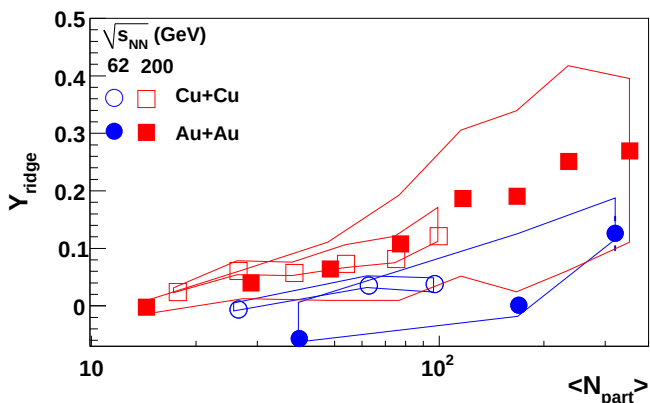
FIG. 12: Dependence of ridge yield on N_{\text{part}} for Cu+Cu and Au+Au collisions at \sqrt{s_{\text{NN}}} = 62.4 \text{ GeV} and 200 \text{ GeV} . Systematic errors due to v_2 are shown as solid lines. The 5% systematic error due to the uncertainty on the associated particle's efficiency is not shown. Color online.
