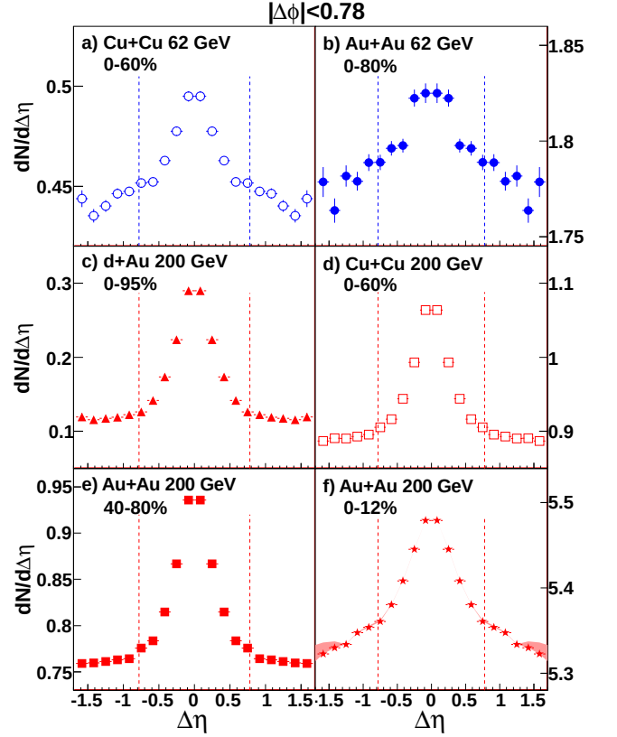
FIG. 5: (Color online) Sample correlations in \Delta\eta ( |\Delta\phi| < 0.78 ) for 3 < p_T^{\text{trigger}} < 6 GeV/c and 1.5 GeV/c < p_T^{\text{associated}} < p_T^{\text{trigger}} for (a) 0-60% Cu+Cu at \sqrt{s_{NN}} = 62.4 GeV (b) 0-80% Au+Au at \sqrt{s_{NN}} = 62.4 GeV, (c) 0-95% d+Au at \sqrt{s_{NN}} = 200 GeV, (d) 0-60% Cu+Cu at \sqrt{s_{NN}} = 200 GeV, (e) 40-80% Au+Au at \sqrt{s_{NN}} = 200 GeV, and (f) 0-12% central Au+Au at \sqrt{s_{NN}} = 200 GeV. Lines show the \Delta\eta range where the jet-like yield is determined. The data are averaged between positive and negative \Delta\eta and reflected in the plot. Shaded bands in (f) show the systematic errors discussed in III F.
