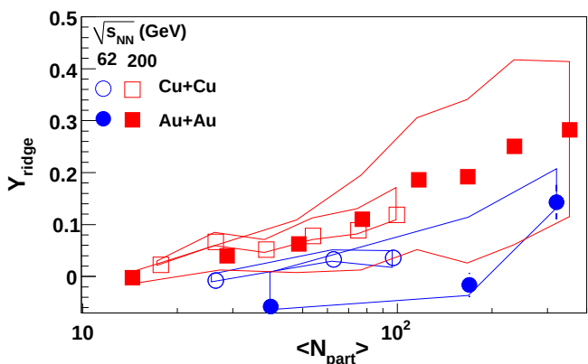
FIG. 12: (Color online) Dependence of ridge on \langle N_{\text{part}} \rangle for 3 < p_T^{\text{trigger}} < 6 GeV/c and 1.5 GeV/c < p_T^{\text{associated}} < p_T^{\text{trigger}} for Cu+Cu, and Au+Au at \sqrt{s_{NN}} = 62.4 GeV and d+Au, Cu+Cu and Au+Au at \sqrt{s_{NN}} = 200 GeV. Systematic errors due to v_2 are shown as solid lines. The 5% systematic error due to the uncertainty on the associated particle's efficiency is not shown and systematic errors due to the acceptance correction are given in Table II.
