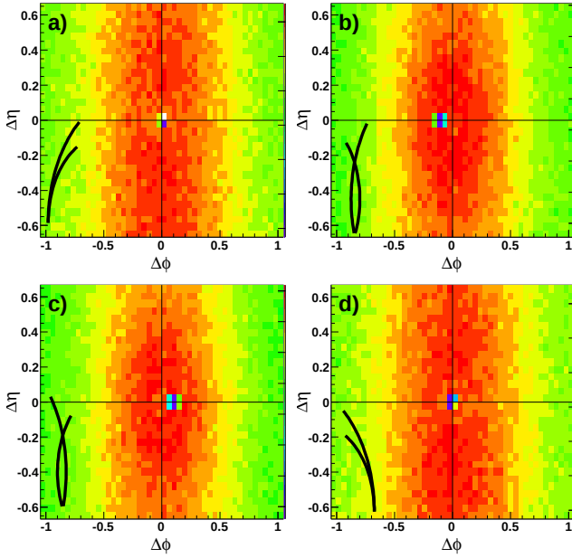
FIG. 3: (Color online) The dip region in (\Delta\phi, \Delta\eta) uncorrected di-hadron correlations in 0-12% central Au+Au collisions at \sqrt{s_{NN}} = 200 GeV for 3 < p_T^{\text{trigger}} < 6 GeV/c and 1.5 GeV/c < p_T^{\text{associated}} < p_T^{\text{trigger}} in the four helicity combinations of trigger and associated particles: (a) (h_{\text{trig}}, h_{\text{assoc}}) = (1,1) , (b) (h_{\text{trig}}, h_{\text{assoc}}) = (1,-1) , (c) (h_{\text{trig}}, h_{\text{assoc}}) = (-1,1) , and (d) (h_{\text{trig}}, h_{\text{assoc}}) = (-1,-1) . Cartoons indicate which dips are from track merging and which are from track crossing.
