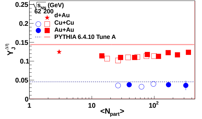
FIG. 8: (Color online) Dependence of jet-like yield on \langle N_{\text{part}} \rangle for 3 < p_T^{\text{trigger}} < 6 GeV/c and 1.5 GeV/c < p_T^{\text{associated}} < p_T^{\text{trigger}} for Cu+Cu, and Au+Au at \sqrt{s_{NN}} = 62.4 GeV and d+Au, Cu+Cu and Au+Au at \sqrt{s_{NN}} = 200 GeV. Comparisons to PYTHIA, \langle N_{\text{part}} \rangle = 2 , are shown as shaded bands. The 5% systematic error due to the uncertainty on the associated particle's efficiency is not shown and systematic errors due to the acceptance correction are given in Table II. The background level and v_2 values used for the extraction of these yields are given in Table IV.
