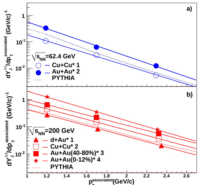
FIG. 10: (Color online) Dependence of jet-like yield on p_T^{associated} for 3 < p_T^{trigger} < 6 \text{ GeV}/c for (a) 0-60% Cu+Cu and 0-80% Au+Au collisions at \sqrt{s_{NN}} = 62.4 GeV and (b) 0-95% d+Au , 0-60% Cu+Cu , 0-12% Au+Au and 40-80% Au+Au collisions at \sqrt{s_{NN}} = 200 GeV. Solid lines through the data points are fits to the data. Comparisons to PYTHIA are shown as dashed lines. The 5% systematic error due to the uncertainty on the associated particle's efficiency is not shown and systematic errors due to the acceptance correction are given in Table II.
