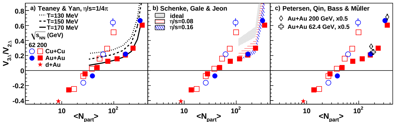
FIG. 14: (Color online) V_{3\Delta}/V_{2\Delta} ratio as a function of \langle N_{\text{part}} \rangle . Statistical errors only. The data are compared to hydrodynamical calculations using (a) lattice equation of state with three different freeze-out temperatures in Au+Au collisions at \sqrt{s_{NN}} = 200 GeV from [64] (b) using a 3+1D viscous hydrodynamical model with three different viscosity to entropy ratios, \eta/s [65], and (c) a 3+1D model incorporating both hydrodynamics and transport model [66].
