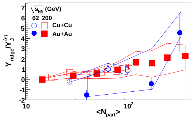
FIG. 13: (Color online) Ratio of the ridge and jet-like yields as a function of \langle N_{\text{part}} \rangle . Systematic errors due to v_2 are shown as solid lines and systematic errors due to the acceptance correction are given in Table II.
