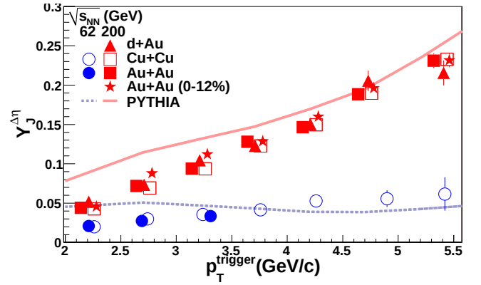
FIG. 9: (Color online) Dependence of jet-like yield on p_T^{\text{trigger}} for 0-95% d+Au, 0-60% Cu+Cu at \sqrt{s_{NN}} = 62.4 GeV and \sqrt{s_{NN}} = 200 GeV, 0-80% Au+Au at \sqrt{s_{NN}} = 62.4 GeV, and 0-12% and 40-80% Au+Au at \sqrt{s_{NN}} = 200 GeV. Comparisons to PYTHIA are shown as lines. The 5% systematic error due to the uncertainty on the associated particle's efficiency is not shown and systematic errors due to the acceptance correction are given in Table II.
