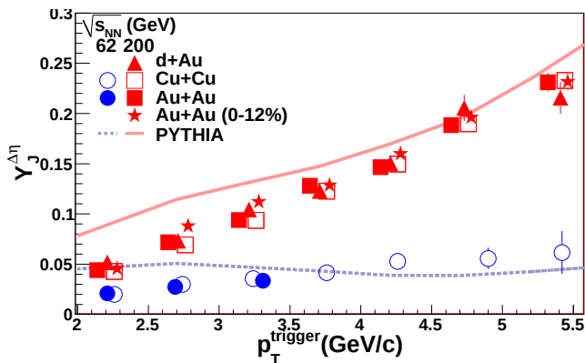
FIG. 9: (Color online) Dependence of jet-like yield on p_T^{\text{trigger}} for 0-95% d +Au, 0-60% Cu+Cu at \sqrt{s_{NN}} = 62.4 GeV and \sqrt{s_{NN}} = 200 GeV, 0-80% Au+Au at \sqrt{s_{NN}} = 62.4 GeV, and 0-12% and 40-80% Au+Au at \sqrt{s_{NN}} = 200 GeV. Comparisons to PYTHIA are shown as lines. The 5% systematic error due to the uncertainty on the associated particle's efficiency is not shown and systematic errors due to the acceptance correction are given in Table II.
