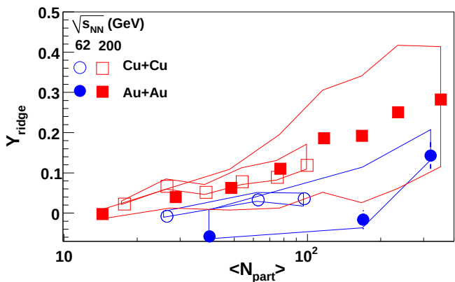
FIG. 12: (Color online) Dependence of the ridge yield on \langle N_{\text{part}} \rangle for 3 < p_T^{\text{trigger}} < 6 GeV/c and 1.5 GeV/c < p_T^{\text{associated}} < p_T^{\text{trigger}} for Cu+Cu, and Au+Au at \sqrt{s_{NN}} = 62.4 GeV and Cu+Cu and Au+Au at \sqrt{s_{NN}} = 200 GeV. Systematic errors due to v_2 are shown as solid lines. The 5% systematic error due to the uncertainty on the associated particle's efficiency is not shown and systematic errors due to the acceptance correction are given in Table II.
