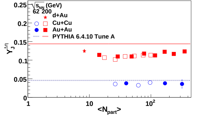
FIG. 8: (Color online) Dependence of jet-like yield on \langle N_{\text{part}} \rangle for 3 < p_T^{\text{trigger}} < 6 GeV/c and 1.5 GeV/c < p_T^{\text{associated}} < p_T^{\text{trigger}} for Cu+Cu and Au+Au at \sqrt{s_{NN}} = 62.4 GeV and d+Au, Cu+Cu and Au+Au at \sqrt{s_{NN}} = 200 GeV. Comparisons to PYTHIA, \langle N_{\text{part}} \rangle = 2 , are shown as lines. The 5% systematic error due to the uncertainty on the associated particle's efficiency is not shown and systematic errors due to the acceptance correction are given in Table II. The background level and v_2 values used for the extraction of these yields are given in Table IV.
