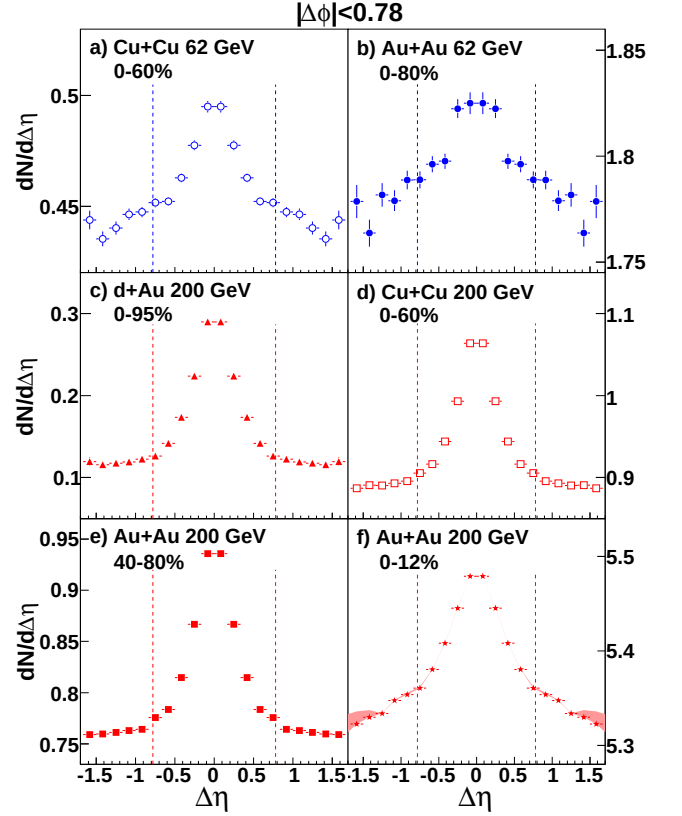
FIG. 5: Color online) Sample correlations in \Delta\eta ( |\Delta\phi| < 0.78 ) for 3 < p_T^{\text{trigger}} < 6 GeV/c and 1.5 GeV/c < p_T^{\text{associated}} < p_T^{\text{trigger}} for (a) 0-60% Cu+Cu at \sqrt{s_{NN}} = 62.4 GeV (b) 0-80% Au+Au at \sqrt{s_{NN}} = 62.4 GeV, (c) 0-95% d+Au at \sqrt{s_{NN}} = 200 GeV, (d) 0-60% Cu+Cu at \sqrt{s_{NN}} = 200 GeV, (e) 40-80% Au+Au at \sqrt{s_{NN}} = 200 GeV, and (f) 0-12% central Au+Au at \sqrt{s_{NN}} = 200 GeV. Lines show the \Delta\eta range where the jet-like yield is determined. The data are averaged between positive and negative \Delta\eta and reflected in the plot. Shaded lines in (f) show the systematic errors discussed in III F.
