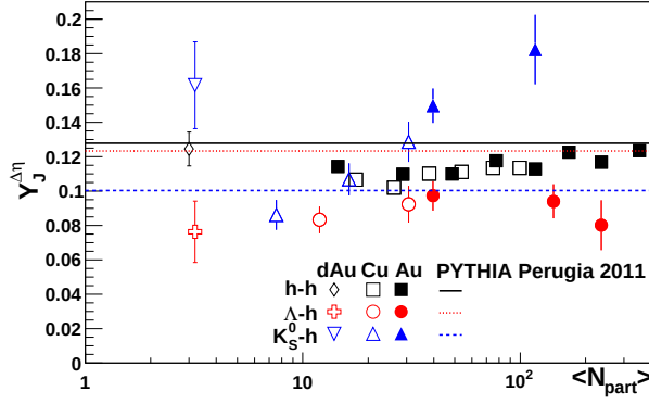
FIG. 4: (Color online.) Centrality dependence of the jet-like yield of K_S^0 -h, and \Lambda -h correlations for 3 < p_T^{\text{trigger}} < 6 GeV/c and 1.5 \text{ GeV/c} < p_T^{\text{associated}} < p_T^{\text{trigger}} in d+Au, Cu+Cu, and Au+Au collisions at \sqrt{s_{NN}} = 200 GeV. The data are compared to PYTHIA [34] calculations using the Perugia 2011 tune [53]. The systematic uncertainty due to the uncertainty on the associated particle's reconstruction efficiency (5%) and background level extraction (2%) are not shown.
