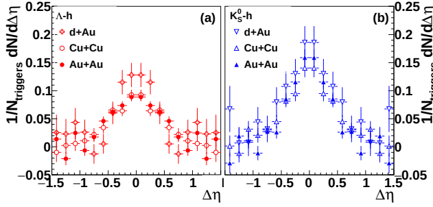
FIG. 2: (Color online.) Corrected correlation functions \frac{dN_J}{d\Delta\eta} in |\Delta\phi| \leq 1.0 - 0.78 for 3 < p_T^{\text{trigger}} < 6 GeV/c and 1.5 GeV/c < p_T^{\text{associated}} < p_T^{\text{trigger}} for (left) \Lambda -h and (right) K_S^0 -h for minimum bias d+Au, 0-20% Cu+Cu, and 40-80% Au+Au collisions at \sqrt{s_{NN}} = 200 GeV after background subtraction. The data have been reflected about \Delta\eta = 0 .
