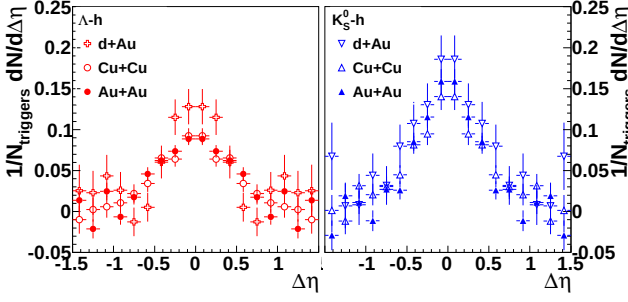
FIG. 2: Corrected correlation functions \frac{dN_J}{d\Delta\eta} in |\Delta\phi| < 1.078 for 3 < p_T^{\text{trigger}} < 6 GeV/c and 1.5 GeV/c < p_T^{\text{associated}} < p_T^{\text{trigger}} for \Lambda -h (left) and K_S^0 -h (right) for minimum bias d+Au, 0-20% Cu+Cu, and 40-80% Au+Au collisions at \sqrt{s_{NN}} = 200 GeV after background subtraction. The data have been reflected about \Delta\eta = 0 .
