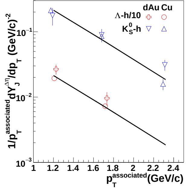
FIG. 6: (Color online.) The jet-like yield as a function of p_T^{\text{associated}} for K_S^0 -h, and \Lambda -h correlations for 3 < p_T^{\text{trigger}} < 6 \text{ GeV}/c in d +Au and 0-60% Cu+Cu collisions at \sqrt{s_{NN}} = 200 \text{ GeV} . The data are compared to the jet-like yield from h-h correlations [7] from 40-80% Au+Au collisions as a band where the width represents the error line. Data are binned in 1.0 < p_T^{\text{associated}} < 1.5 \text{ GeV}/c , 1.5 < p_T^{\text{associated}} < 2.0 \text{ GeV}/c , and 2.0 < p_T^{\text{associated}} < 3.0 \text{ GeV}/c and are plotted at the mean of the bin. The systematic uncertainty due to the uncertainty on the associated particle's reconstruction efficiency (5%) and background level extraction (2%) are not shown.
