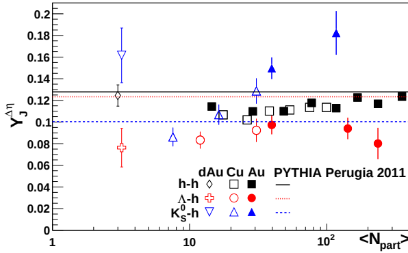
FIG. 5: (Color online.) Centrality dependence of the jet-like yield of K_S^0 -h, and \Lambda -h correlations for 3 < p_T^{\text{trigger}} < 6 \text{ GeV}/c and 1.5 \text{ GeV}/c < p_T^{\text{associated}} < p_T^{\text{trigger}} in d +Au, Cu+Cu, and Au+Au collisions at \sqrt{s_{NN}} = 200 \text{ GeV} . The data are compared to PYTHIA [28] calculations using the Perugia 2011 tune [45]. The systematic uncertainty due to the uncertainty on the associated particle's reconstruction efficiency (5%) and background level extraction (2%) are not shown.
