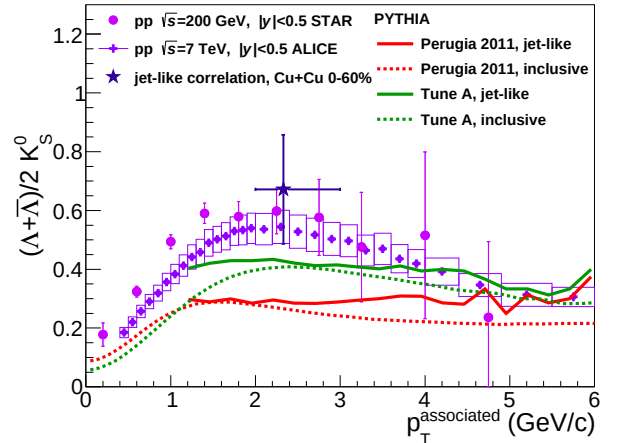
FIG. 3: (Color online.) \Lambda/K_S^0 ratio measured in the jet-like correlation in 0-60% Cu+Cu collisions at \sqrt{s_{NN}} = 200 GeV for 3 < p_T^{\text{trigger}} < 6 GeV/c and 2.0 < p_T^{\text{associated}} < 3.0 GeV/c along with this ratio obtained from inclusive p_T spectra in p+p collisions. Data are compared to calculations from PYTHIA [34] using the Perugia 2011 tunes [53] and Tune A [54].
