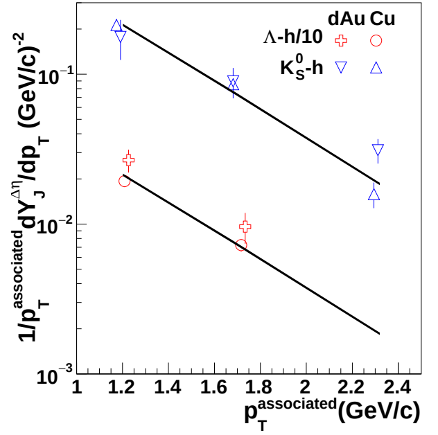
FIG. 5: (Color online.) The jet-like yield as a function of p_T^{\text{associated}} for K_S^0 -h, and \Lambda -h correlations for 3 < p_T^{\text{trigger}} < 6 GeV/c in d+Au and 0-60% Cu+Cu collisions at \sqrt{s_{NN}} = 200 GeV. The data are compared to the jet-like yield from h-h correlations [10] from 40-80% Au+Au collisions as a band where the width represents the errorline. Data are binned in 1.0 < p_T^{\text{associated}} < 1.5 GeV/c, 1.5 < p_T^{\text{associated}} < 2.0 GeV/c, and 2.0 < p_T^{\text{associated}} < 3.0 GeV/c and are plotted at the mean of the bin. The systematic uncertainty due to the uncertainty on the associated particle's reconstruction efficiency (5%) and background level extraction (2%) are not shown.
