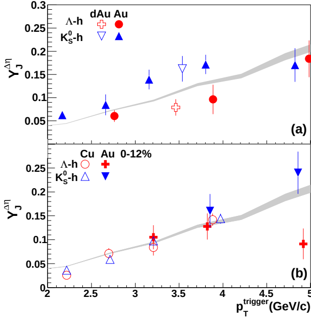
FIG. 6: (Color online.) The jet-like yield in |\Delta\eta| < 0.78 as a function of p_T^{\text{trigger}} for K_S^0 -h, and \Lambda -h correlations for 1.5 \text{ GeV}/c < p_T^{\text{associated}} < p_T^{\text{trigger}} in (a) minimum bias d+\text{Au} and 40-80% \text{Au}+\text{Au} collisions at \sqrt{s_{NN}} = 200 \text{ GeV} and (b) 0-60% \text{Cu}+\text{Cu} and 0-12% \text{Au}+\text{Au} collisions at \sqrt{s_{NN}} = 200 \text{ GeV} . For comparison h-h correlations [10] from 40-80% \text{Au}+\text{Au} collisions are shown as a band where the width represents the uncertainty. Peripheral \text{Au}+\text{Au} points have been shifted in p_T^{\text{trigger}} for visibility. The systematic uncertainty due to the uncertainty on the associated particle's reconstruction efficiency (5%) and background level extraction (2%) are not shown.
