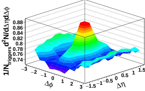
FIG. 1: (Color online.) Corrected 2D K_S^0 -h correlation function for 3 < p_T^{\text{trigger}} < 6 GeV/c and 1.5 GeV/c < p_T^{\text{associated}} < p_T^{\text{trigger}} for 0-20% Cu+Cu. The data have been reflected about \Delta\eta = 0 and \Delta\phi = 0 .
