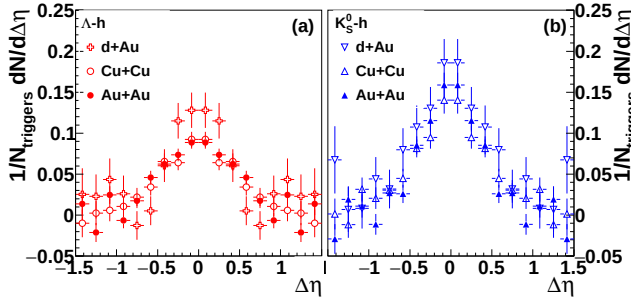
FIG. 2: (Color online.) Corrected correlation functions \frac{dN_J}{d\Delta\eta} in |\Delta\phi| \leq 1.0 for 3 < p_T^{\text{trigger}} < 6 GeV/c and 1.5 GeV/c < p_T^{\text{associated}} < p_T^{\text{trigger}} for (left) \Lambda -h and (right) K_S^0 -h for minimum bias d+Au, 0-20% Cu+Cu, and 40-80% Au+Au collisions at \sqrt{s_{NN}} = 200 GeV after background subtraction. The data have been reflected about \Delta\eta = 0 .
