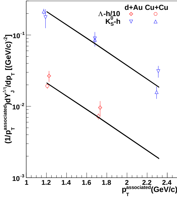
FIG. 6: (Color online.) The jet-like yield as a function of p_T^{\text{associated}} for K_S^0 -h and \Lambda -h correlations for 3 < p_T^{\text{trigger}} < 6 GeV/c in d+Au and 0-60% Cu+Cu collisions at \sqrt{s_{NN}} = 200 GeV. The data are compared to the jet-like yield from h-h correlations [9] from 40-80% Au+Au collisions shown as a line. Data are binned in 1.0 < p_T^{\text{associated}} < 1.5 GeV/c, 1.5 < p_T^{\text{associated}} < 2.0 GeV/c, and 2.0 < p_T^{\text{associated}} < 3.0 GeV/c and are plotted at the mean of the bin. The systematic uncertainty due to the uncertainty on the associated particle's reconstruction efficiency (5%) and background level extraction (2%) are not shown.
