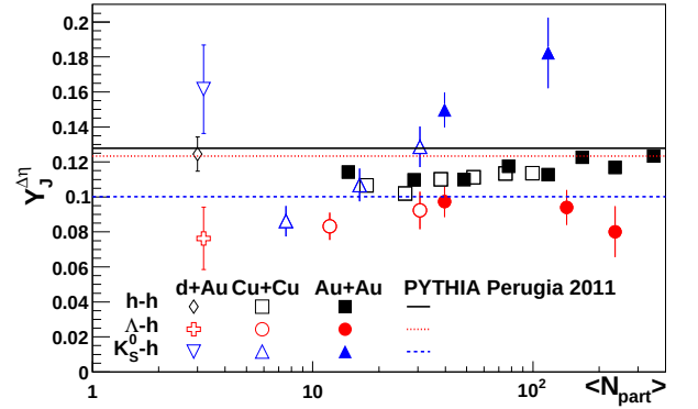
FIG. 5: (Color online.) Centrality dependence of the jet-like yield of K_S^0 -h and \Lambda -h correlations for 3 < p_T^{\text{trigger}} < 6 GeV/c and 1.5 \text{ GeV/c} < p_T^{\text{associated}} < p_T^{\text{trigger}} in d +Au, Cu+Cu, and Au+Au collisions at \sqrt{s_{NN}} = 200 GeV. The data are compared to PYTHIA [34] calculations using the Perugia 2011 tune [52]. The systematic uncertainty due to the uncertainty on the associated particle's reconstruction efficiency (5%) and background level extraction (2%) are not shown.
