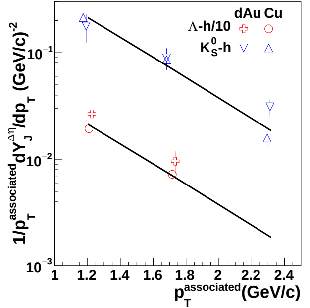
FIG. 6: The jet-like yield as a function of p_T^{\text{associated}} for K_S^0 -h, and \Lambda -h correlations for 3 < p_T^{\text{trigger}} < 6 \text{ GeV}/c in d +Au and 0-60% Cu+Cu collisions at \sqrt{s_{NN}} = 200 \text{ GeV} . The data are compared to the jet-like yield from h-h correlations [7] from 40-80% Au+Au collisions are shown as a band where the width represents the error. Data are binned in 1.0 < p_T^{\text{associated}} < 1.5 \text{ GeV}/c , 1.5 < p_T^{\text{associated}} < 2.0 \text{ GeV}/c , and 2.0 < p_T^{\text{associated}} < 3.0 \text{ GeV}/c and are plotted at the mean of the bin. The systematic errors due to the uncertainty on the associated particle's reconstruction efficiency (5%) and background level extraction (2%) are not shown.
