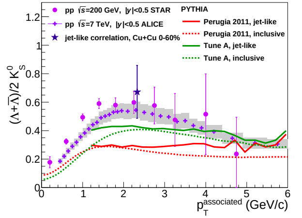
FIG. 3: \Lambda/K_S^0 ratio measured in the jet-like correlation in 0-60% Cu+Cu collisions at \sqrt{s_{NN}} = 200 GeV for 3 < p_T^{\text{trigger}} < 6 GeV/c and 2.0 < p_T^{\text{associated}} < 3.0 GeV/c along with this ratio obtained from inclusive p_T spectra in p+p collisions. Data are compared to calculations from PYTHIA [44] using the Perugia 2011 tunes [45] and Tune A [46]. The systematic errors due to the uncertainty on the associated particle's reconstruction efficiency (5%) and background level extraction (2%) are not shown.
